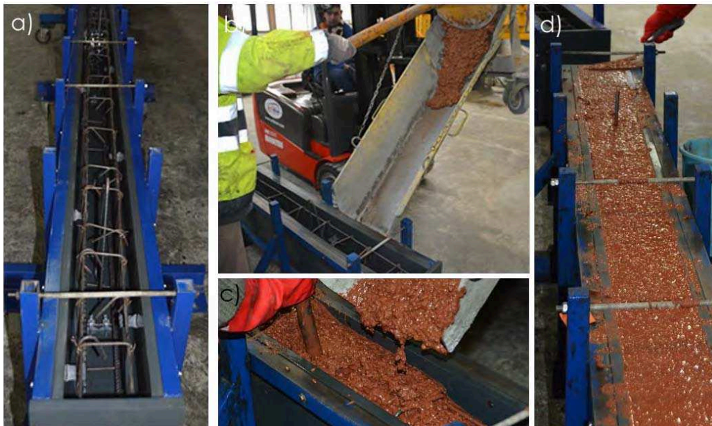
Figure 22. a) Beam mould with the steel reinforcement; b) descent of the fresh concrete by gutter; c) vibration of the fresh geopolymer concrete using a vibrating needle and d) levelling of the beam with a trowel.
