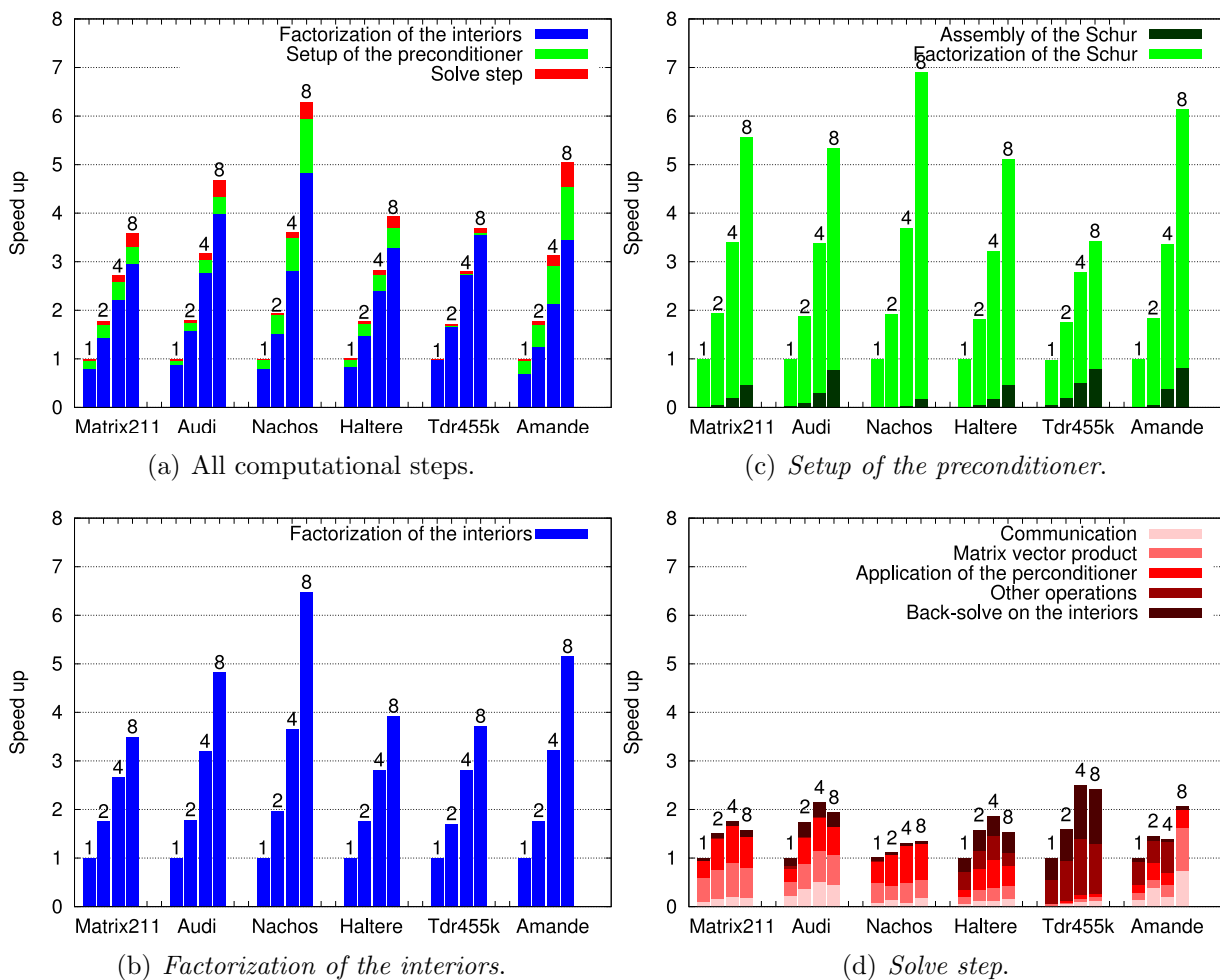
Figure 2.9: Overall speed-up with using 1, 2, 4 or 8 threads (and cores) with respect to the time when 1 thread (and core) per process, for the matrices from Table 2.1. The dense preconditioner is used. Four nodes are used and one process per node is assigned. The number of threads (1, 2, 4 or 8) for each histogram is given on the top of the bars.
