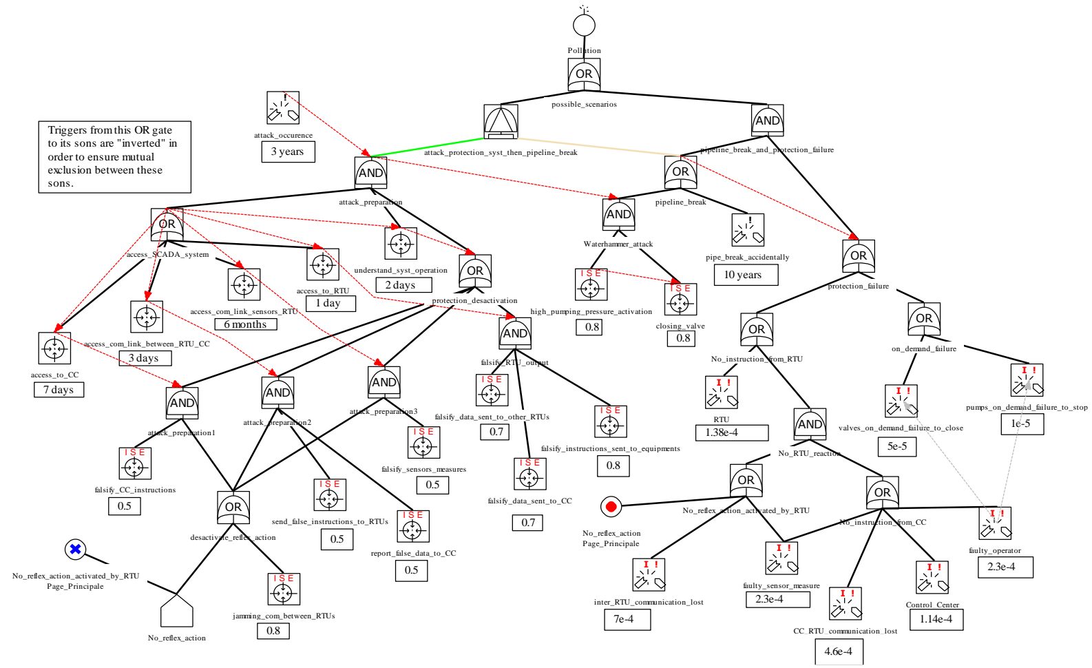
Figure 18: BDMP model of the pipeline and its control system
