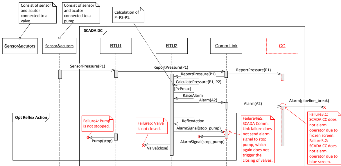
Figure 24: A decomposed FSD providing the details of failures in the SCADA system
