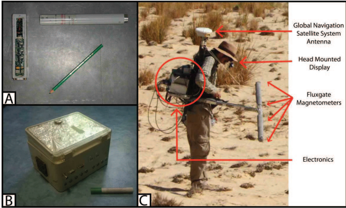
Figure 3: A- 3-axis fluxgate magnetometer (Bartington Inc., Mag-03 MC). B- Custom electronics with 8 magnetometer inputs developed by the IPGS. C- Multi-sensor device developed by the IPGS.
