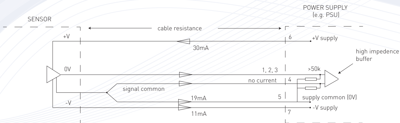
Mag-03 electrical schematic
