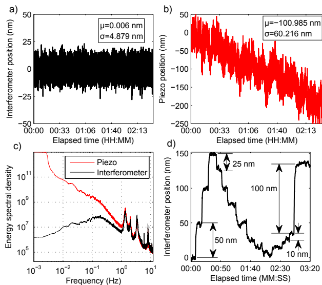
FIG. 7. Active stabilization performance. a) Position of the interferometer over more than 2 hours. b) Piezo position compensation to keep the interferometer at a fixed position. c) Comparison between the stabilized (black) and compensation (red) energy spectral density. d) Examples of interferometer positions and its stability for various step size.
