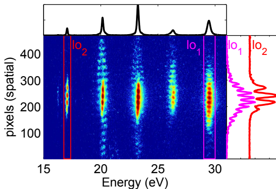
FIG. 4. Spatially resolved XUV spectrum of harmonics 11 th to 19 th of a 800nm fundamental beam in a 2 source configuration. Top marginal: average spectrum across the spatial domain. Right marginal: vertical line-outs (signal integrated over energy within the colored rectangles lo_1 and lo_2 ) highlighting the variation of the fringe spacing for different harmonics.
