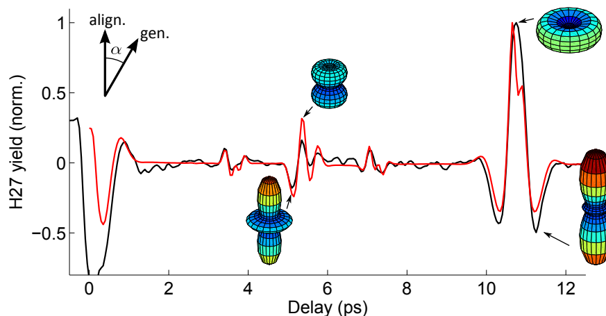
FIG. 9. Yield of the 27th harmonic generated in \text{CO}_2 as a function of the delay between alignment pump and generation probe (black) compared to a simulation using equation 5 (red). Molecular alignment probability density is depicted at specific delays. Pump and probe have parallel polarizations ( \alpha = 0^\circ )
