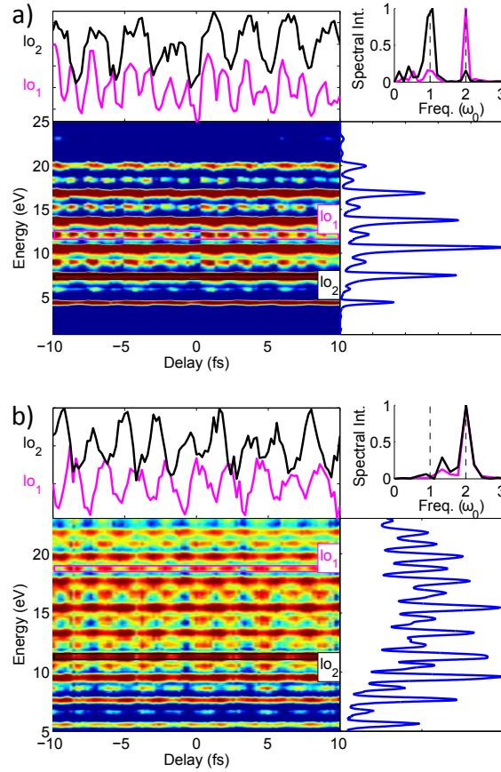
FIG. 6. RABBIT traces obtained with a) 800 nm and b) 1224 nm driving field central wavelengths. For each case, marginals are represented as a function of delay (top) and energy (right). Right top corner: Fourier transform amplitude of the temporal marginals (see details in the text).
