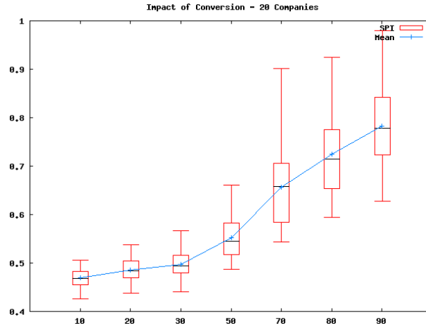
Figure 26: Impact of conversion rate on SPI indicator
