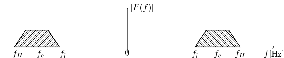
Figure 5.2: A bandpass signal occupying a bandwidth B and located around f_c
