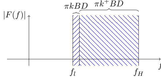
Figure 6.11: Frequency domain operation of the PNS2 technique
