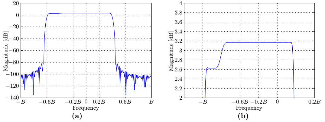
Figure 6.21: Frequency response of the first interpolant when a Kaiser window with a \beta = 6 parameter is used
