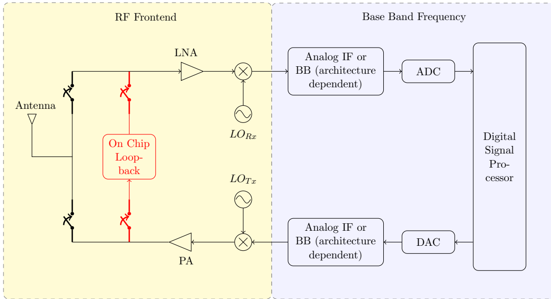
Figure 4.4: Loopback test architecture
