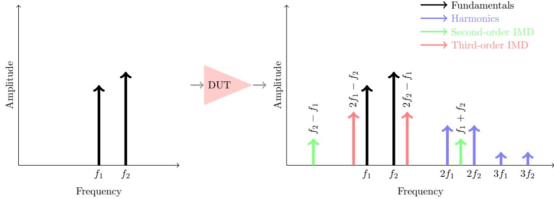
Figure 3.12: Intermodulation distortion - Graphical representation
