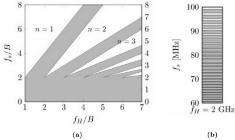
Figure 2.8: The constraints on the sampling rate f_s for undersampling [Vaughan et al., 1991]: 2.8a in general case and 2.8b a particular case where f_H = 2.03 \text{ GHz} and B = 30 \text{ MHz} . The white regions are situations where the undersampling will not result in aliasing. The gray regions represent conditions where alias is occurring.
