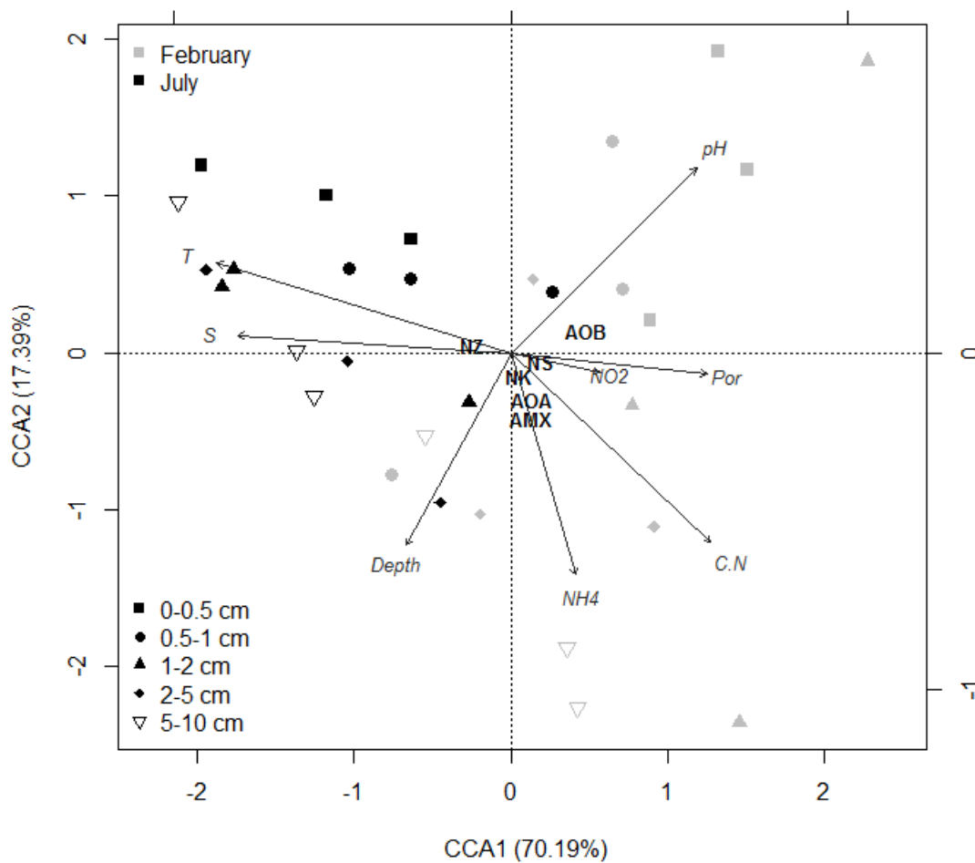
Figure 61. Canonical correlation analysis (cca) ordination of N-related functional genes abundances (copies number, \chi^2 transformed) constrained by 8 abiotic parameters among depths and sampling dates (July = July 5 th , 2012, February = February 11 th , 2013). AOB = ammonia oxidising Bacteria (bacterial amoA gene); AOA= ammonia oxidising Archaea (archaeal amoA gene); NZ = nosZ gene; NS = nirS gene; NK = nirK gene; AMX = anammox; T = temperature; S = salinity; NH4 = ammonia; Por = porosity. The cca analysis explained 67,2% of variance of the functional genes distribution.
