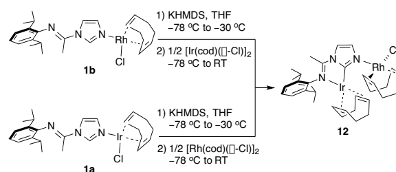
Scheme 13. Synthesis of 12 .
