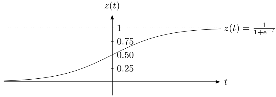
Figure 2.8: Logistic function.
