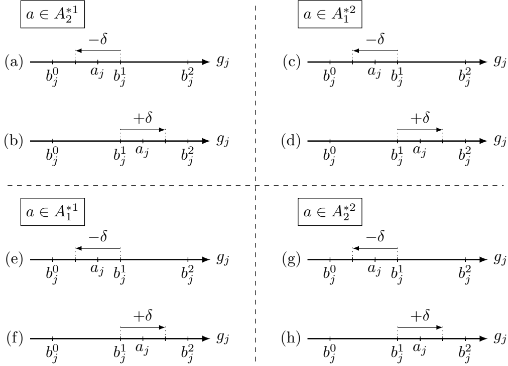
Figure 3.2: Given the evaluation of an alternative a and of the profile b^1 on a criterion j , 8 possible cases regarding the alternative assignment, the current profile value on j and a move of +\delta or -\delta .
