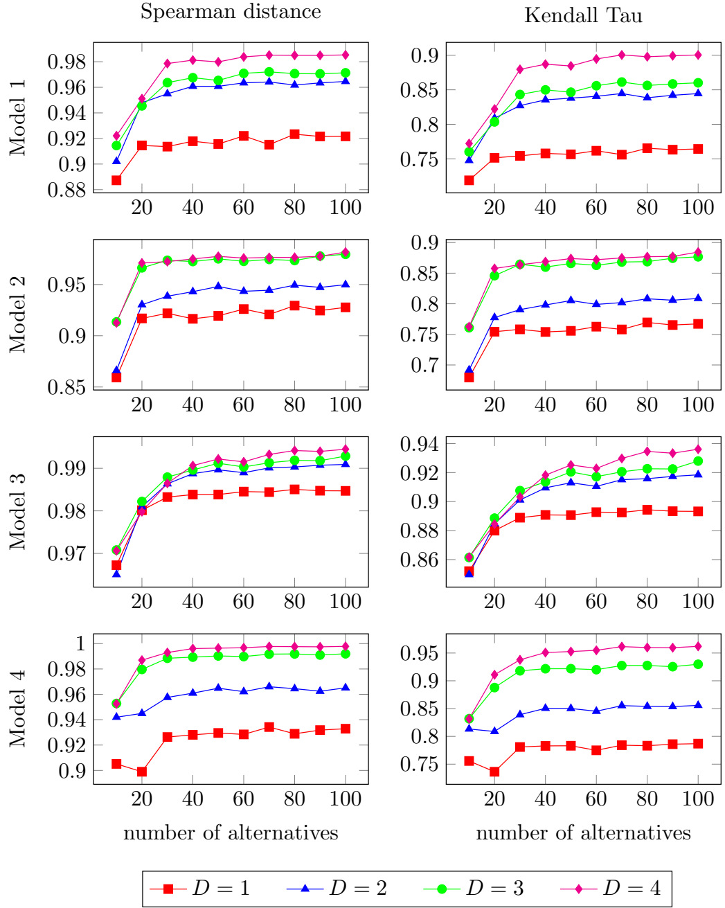
Figure F.1: Average Spearman distance and Kendall Tau of the test set of models 1 to 4 learned by UTA-poly when the degree of the marginals varies between 1 and 4.
