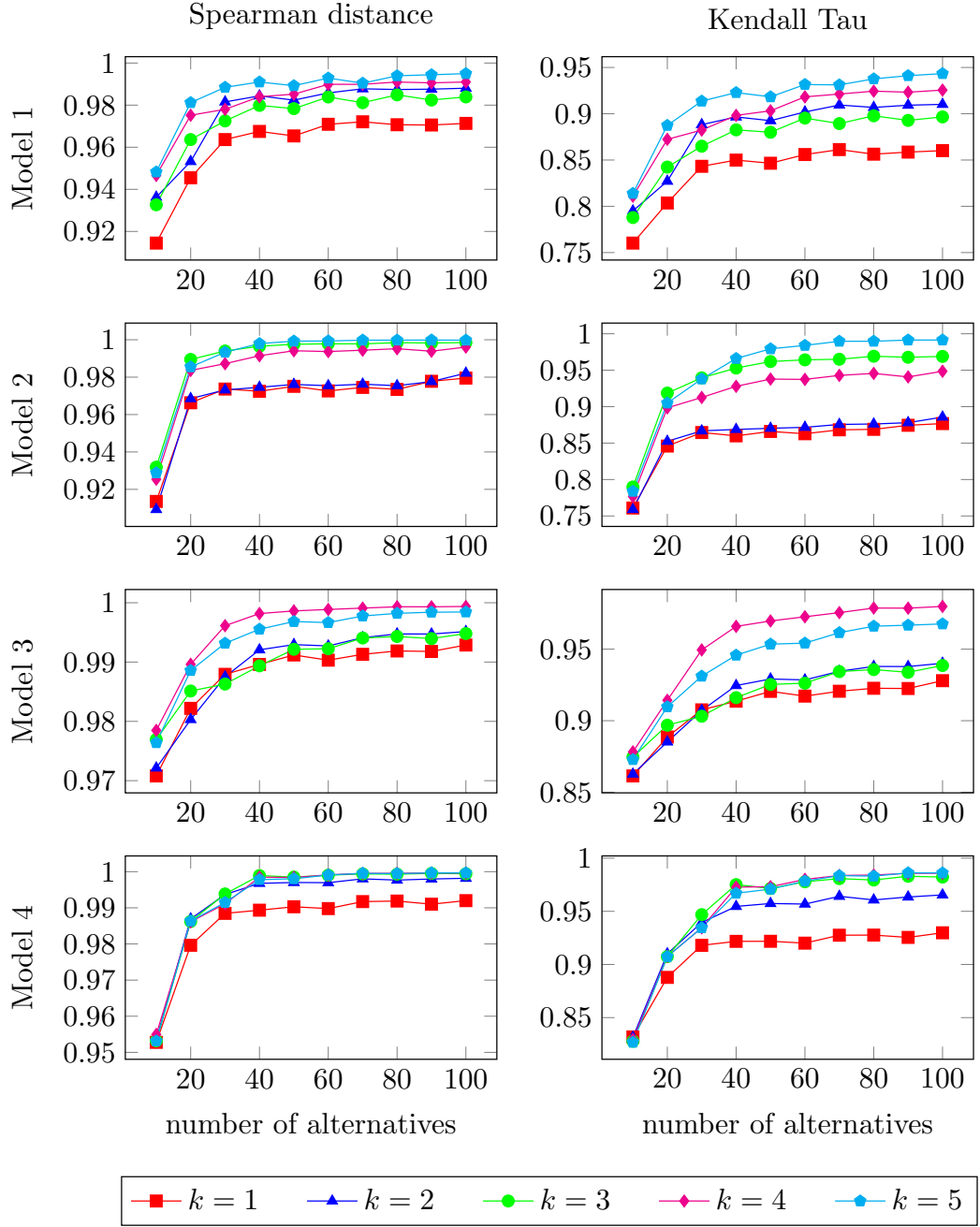
Figure F.3: Average Spearman distance and Kendall Tau of the test set of models 1 to 4 learned by UTA-splines with marginals composed of polynomials of the third degree. The continuity at the breakpoints is ensured up to the second derivative.
