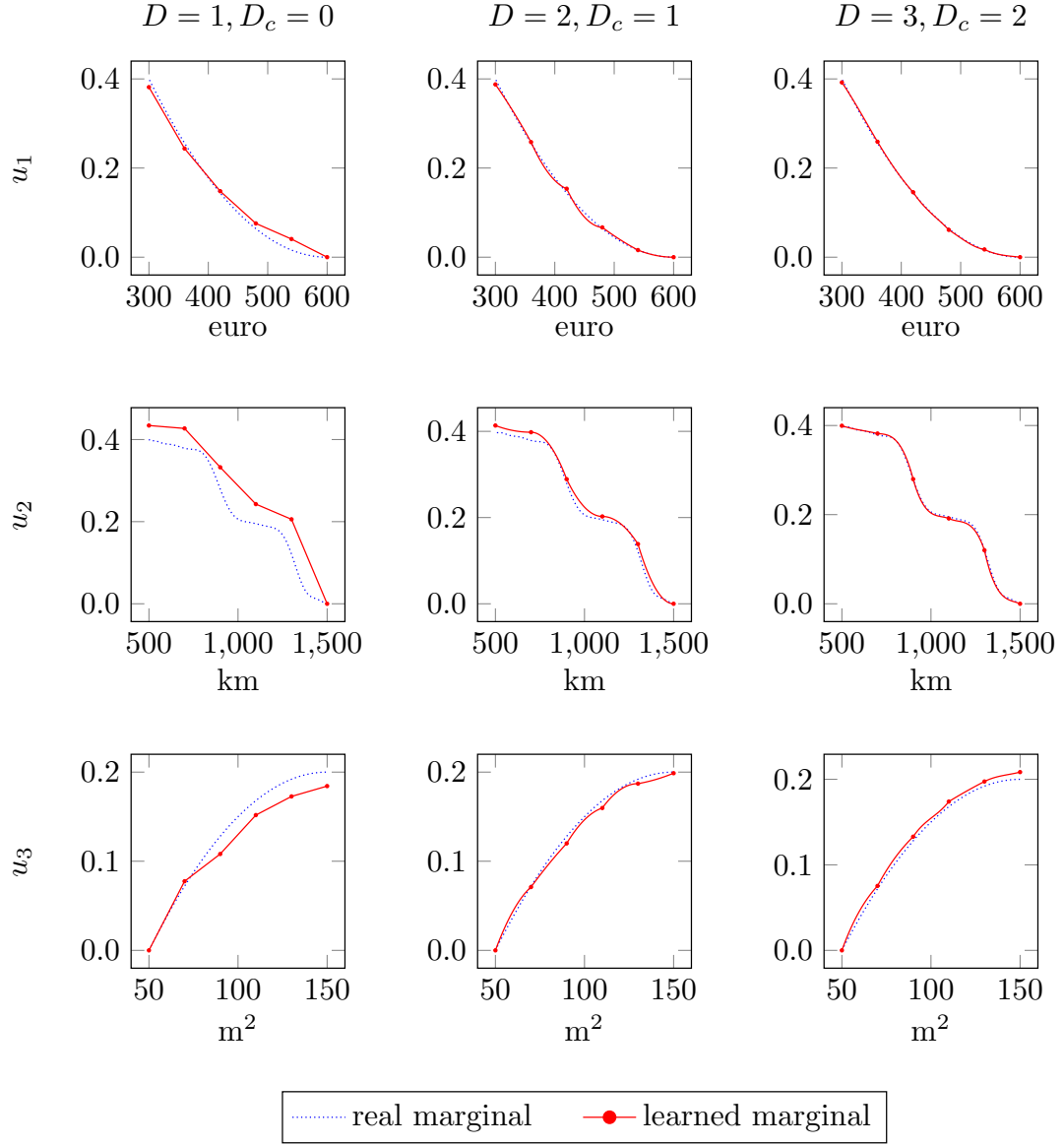
Figure 7.6: Value functions learned by UTA-splines on the basis of a learning set composed of 100 examples with polynomials of degree D = 1 to 3 and marginals composed of 5 polynomials ( k = 5 ). The continuity of the spline ( D_c ) is enforced up to D - 1 .
