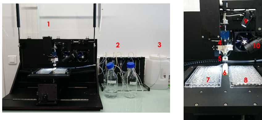
Figure 39. Robot HiClamp (Multi Channel Systems).
