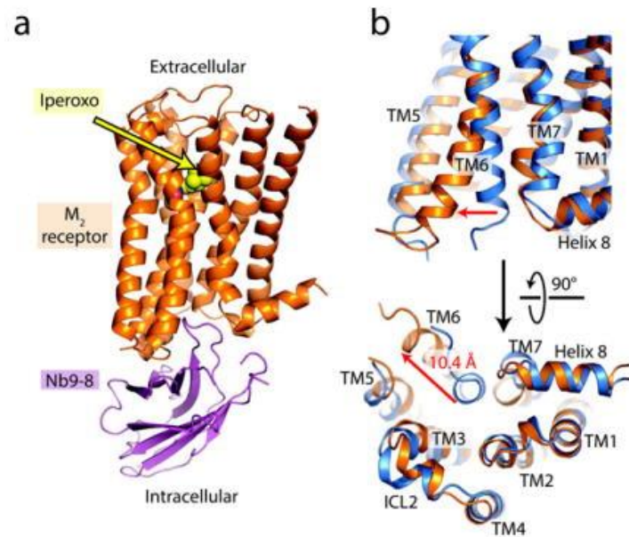
Figure 27. Intracellular changes on activation of the M2 receptor. A , overall structure of the active-state M2 receptor (orange) in complex with the orthosteric agonist iperoxo (yellow) and the active-state stabilizing nanobody (purple). B , compared to the inactive structure of the M2 receptor (blue), transmembrane helix 6 (TM6) is substantially displaced outward, and TM7 has moved inward (Kruse et al., 2013).
