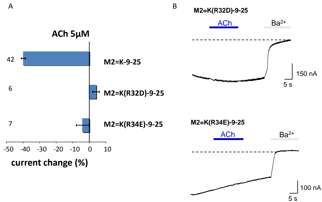
Figure 65. A , percent change in current induced by application of 5 \mu M ACh of M2=K-9-25 and M2=K(R32D)-9-25 mutants. Responses were measured in TEVC. B , representative TEVC traces from Xenopus oocytes expressing M2=K(R32D)-9-25 and M2=K(R34E)-9-25. Current amplitude was recorded at -50 mV. Dashed line indicates the Ba 2+ -sensitive current baseline. Blue and grey bars represent the application of ACh and Ba 2+ respectively.
