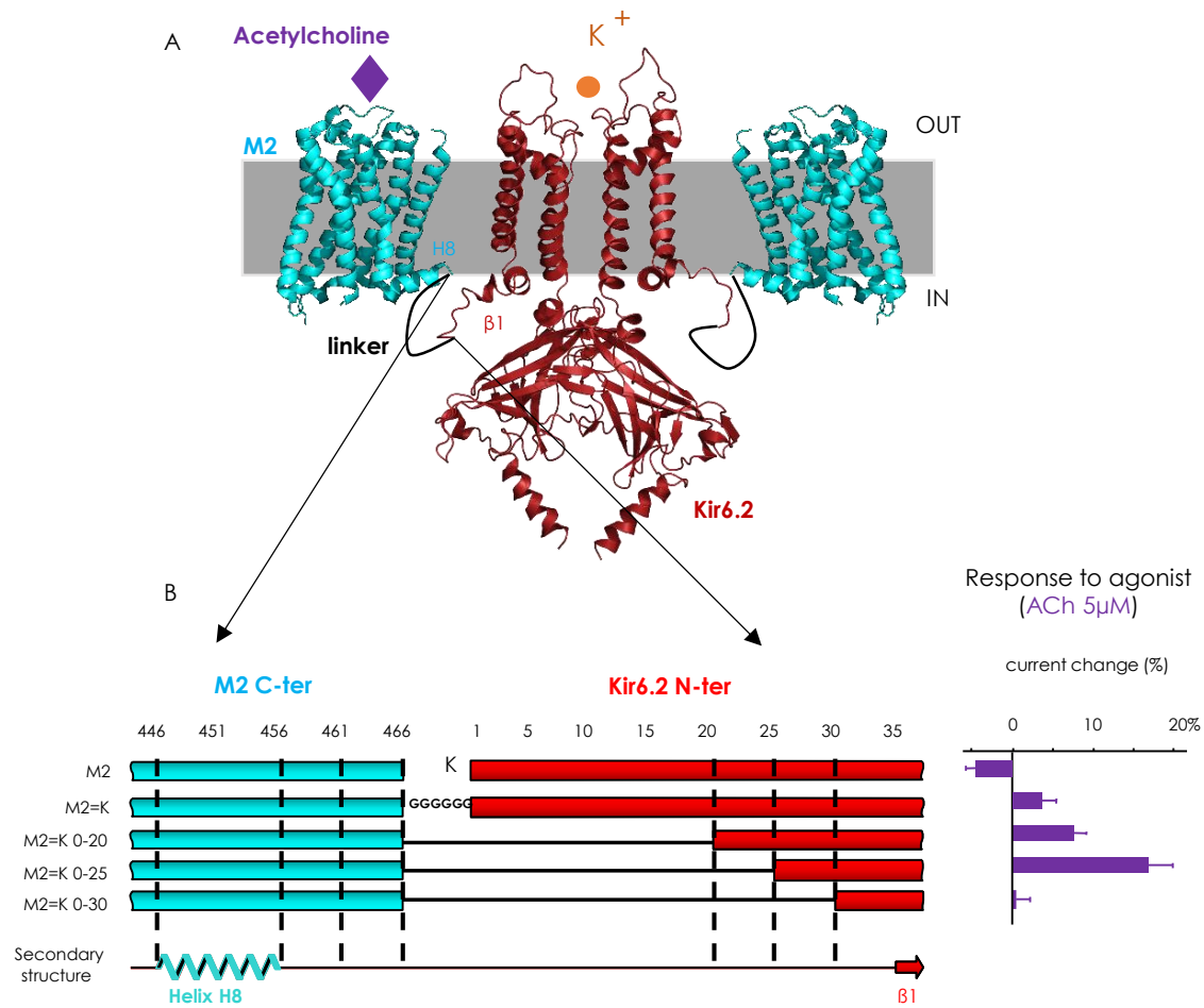
Figure 28. A , model of the M2=K ICCR as seen from the membrane plane. Front and back monomers have been removed for clarity. B , linker region engineering to obtain functional ICCRs and relative responses to Acetylcholine 5μM.
