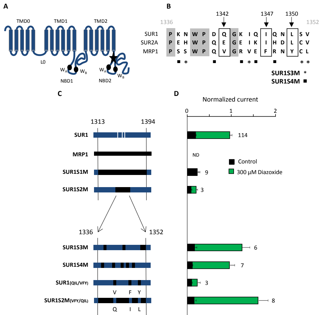
Figure 53. SUR1 residues Q1342, I1347 and L1350 are essential for K-ATP channel activation by Diazoxide. A, putative membrane topology of SUR1 (NBD, nucleotide binding domain; W A , Walker A motif; W B , Walker B motif). The star indicates the region identified by Rainbow et al. (2004) and mutated to obtain the S1M chimera. B, alignment of the amino acid sequences of human SUR1, rat SUR2A and human MRP1. Three residues (boxed) are conserved in SURs and not in MRP1: Q1342, I1347 and L1350. Stars and squares indicate the MRP1 residues introduced in SUR1 to obtain SUR1S3M and SUR1S4M, respectively. C, schematic representation of the chimeras. SUR1 and MRP1 elements are drawn in grey and black, respectively. For clarity, residues Q1342, I1347 and L1350 of SUR1 are indicated by white stripes. D, Diazoxide responses were measured in inside-out patches excised from oocytes co-expressing Kir6.2 and wild-type or chimeric SURs or MRP1 as indicated. Diazoxide (300 μM) was applied in the presence of 100 μM ATP, and currents were normalized to the current measured in the absence of nucleotides immediately before opener application. Application of 100 μM ATP alone (black bars) was used as a control. Numbers at right of bars indicate the number of patches included in each average.
