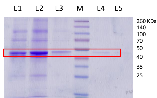
Figure 46. TMD0-eGFP SDS-PAGE of the different elution fractions after MAC in presence of MNG-3. Protein sample in complex with MNG-3 is loaded onto a column containing the high affinity resin for the His-tag present on TMD0-eGFP. The flow-through is discarded while the elution fractions are collected (E1 to E5) and then loaded on a 10 % Acrylamide SDS-PAGE. The monomeric TMD0-eGFP (red box) is shown around 50 kDa.
