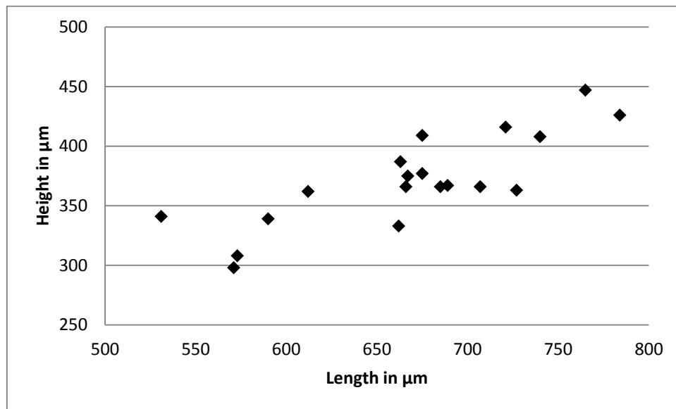
Diagram 3: Height-Length diagram of Acratia sp. 4 sensu Zazzali et al. , 2015.
