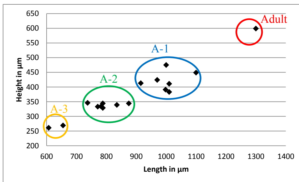
Diagram 15: Height-Length diagram of Bairdia sp. L.
