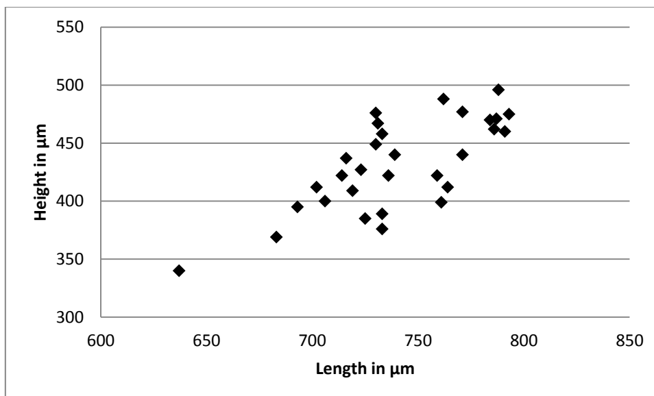
Diagram 10: Height-Length diagram of Bairdia sp. 20 sensu Zazzali et al., 2015.
