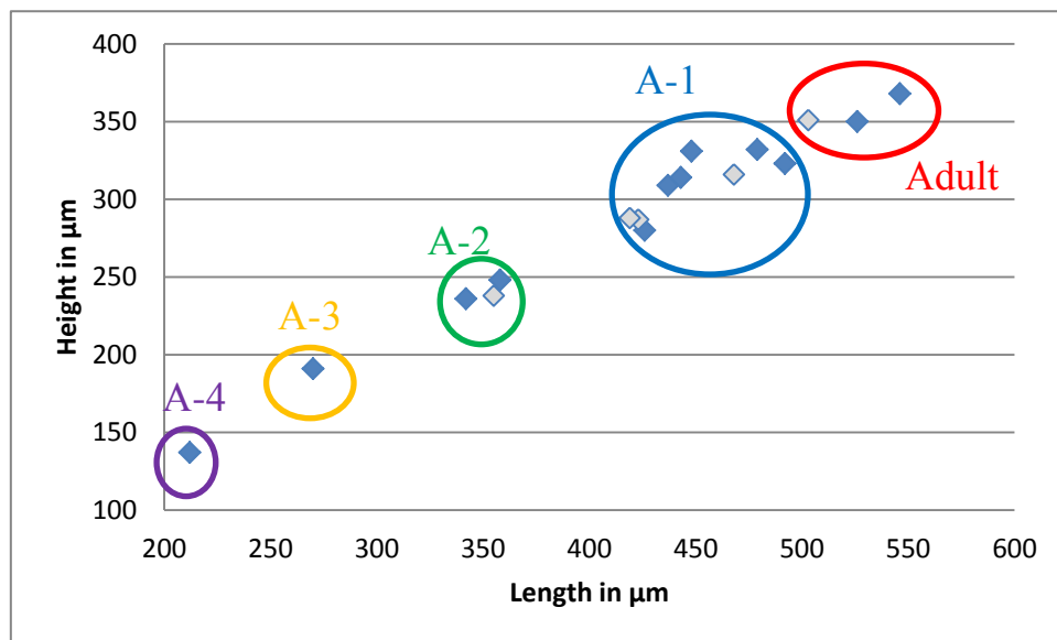
Diagram 24: Height-Length diagram of Microcheilinella sp. B (in blue) and Microcheilinella sp. 2 sensu Zazzali et al. , 2015 (in grey).
