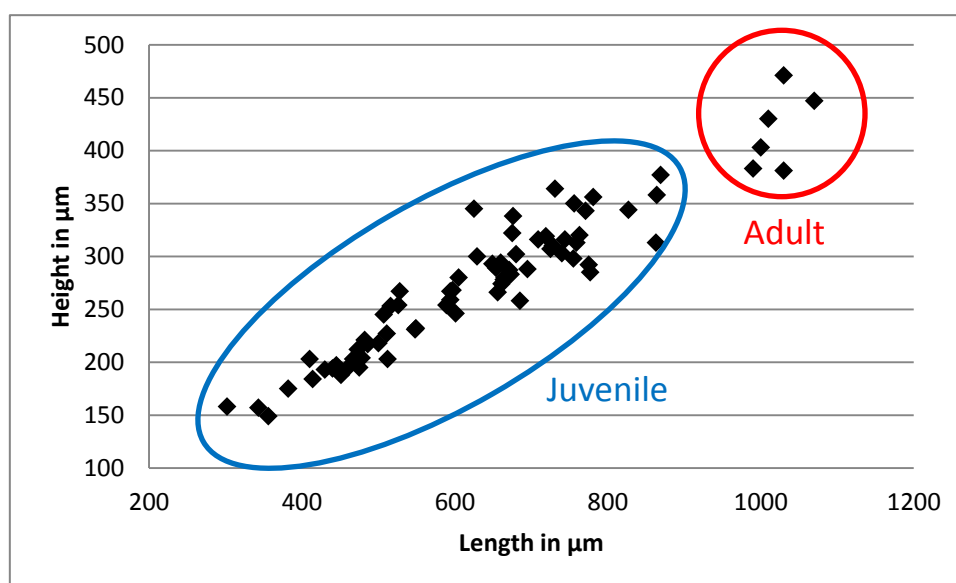
Diagram 8: Height-Length diagram of ? Bairdia cf. subcontracta Chen, 1987 sensu Crasquin-Soleau & Baud., 1998.
