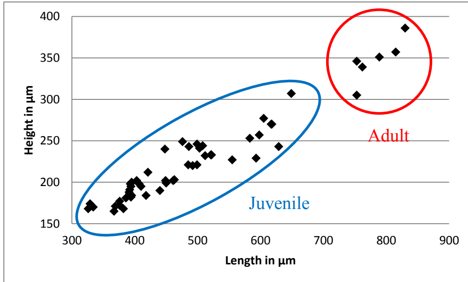
Diagram 16: Height-Length diagram of Bairdiacypris sp. A.
