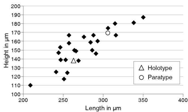
Diagram 22: Height-Length diagram of Microcheilinella pagodaensis Zazzali, 2015.
