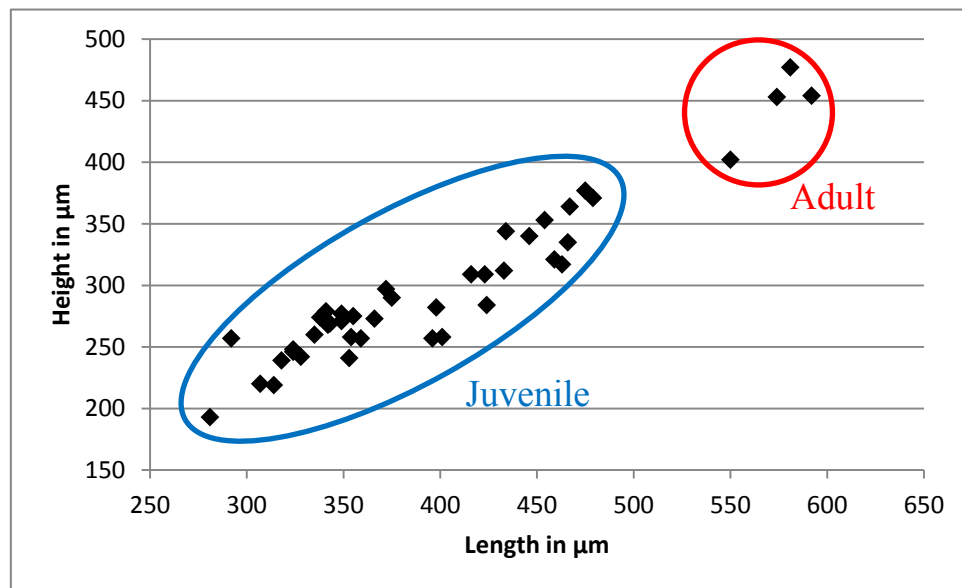
Diagram 2: Height-Length diagram of Samarella viscusforma Chitnarin, 2012.
