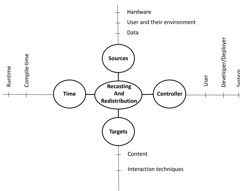
FIGURE 3.5 The problem space for the development of plastic MR user interfaces.
