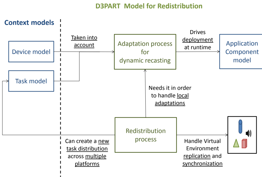
FIGURE 6.3 The D3PART model consists of a redistribution process combined with the local adaptation mechanisms presented before.
