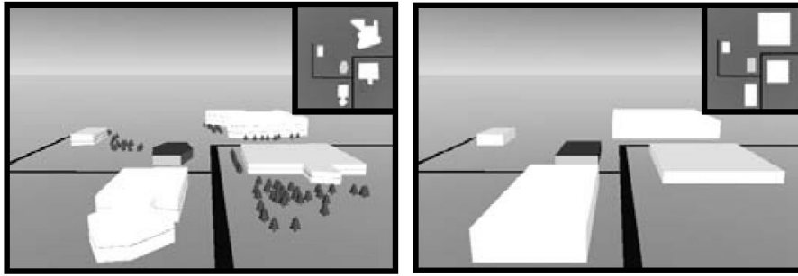
FIGURE 3.2 In the solution proposed by Bilasco [Bilasco et al., 2007], a 3D scene can be adapted according to the semantic of each element. Here, in the image on the right, the geometries of type "building" have been degraded, and the geometries of type "tree" have been removed from the scene.
