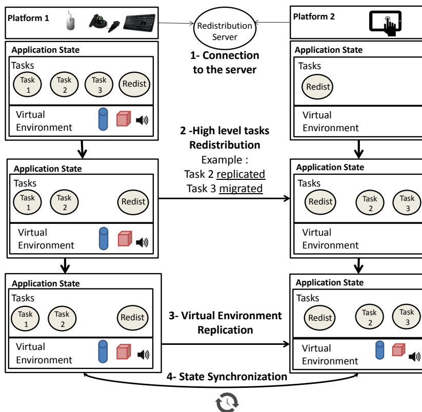
FIGURE 6.4 With D3PART, the redistribution process is performed in four steps. First, the different platforms connect to the redistribution server. An empty application runs on these distant platforms. It only contains the redistribution task. Then, the user initiates a new distribution of the system with the meta-user interface. Here he chooses to replicate the task 2 and to migrate the task 3 to a second platform. For these two tasks, thanks to the dynamic recasting mechanism handled with our adaptation process, compatible application components are automatically deployed on the second platform that fits its capabilities. The third step consists in replicating the VE from the first platform to the second one. It includes 3D meshes, their materials, and sound assets. We ensure that the state of the application remains consistent during the redistribution. Then in the last step, the redistribution server ensures state synchronization between the two platforms while the applications are running.
