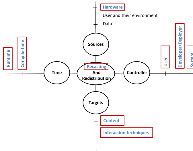
FIGURE 4.1 Regarding our design space problem of plasticity for MR user interfaces, this chapter is interested in adapting the interaction techniques and the content visualization according to the devices. The basis of our models are also described in this Chapter so we also describe how we can handle the different adaptation times and adaptation controllers.
