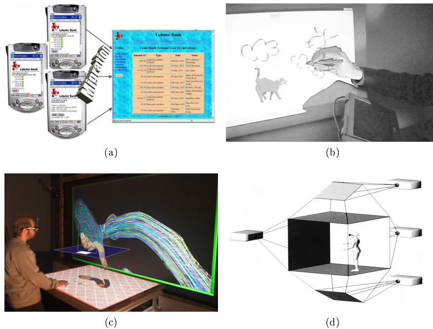
FIGURE 6.2 Four examples of distribution at different levels. (a) A bank application that can be redistributed at the application level [Bandelloni and Paternò, 2004]. (b) The painter metaphor [Rekimoto, 1997] is an example of distribution at the workspace level. (c) Slice WIM [Coffey et al., 2011] is an example of distribution at the domain concept level. (d) A CAVE [Cruz-Neira et al., 1992] is an example of distribution at the pixel level.
