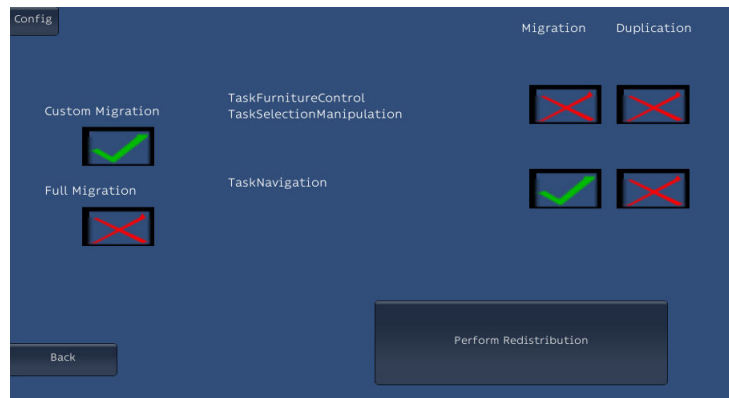
FIGURE 6.5 The extension of the meta-user interface to control the redistribution process. Here, the user chooses the high level tasks that will be redistributed to the distant platform. In this example based on the furniture planning application, three tasks can be redistributed: navigation, selection/manipulation and furniture control. The last two ones are dependent. The user chooses a partial migration, only the navigation task will be redistributed. The two others tasks remain on his current platform.
