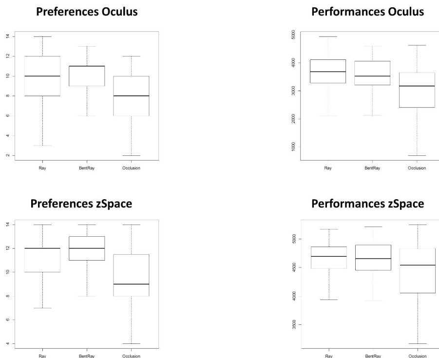
FIGURE 7.6 Comparison of the preferences and performances results for the three techniques on the two device setups. The results for the 3D Ray-based interaction technique and the 3D Bentray are similar. However, the 3D Bentray seems to be preferred on the zSpace. We can also see that participants less preferred and less performed with the Occlusion selection technique.
