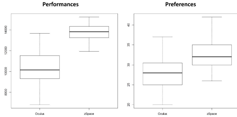
FIGURE 7.7 Comparison of the global performances and of the global grades between the two device setups. As shown the performances have been globally better on the zSpace. In the same way the three interaction techniques have globally obtained better grades on the zSpace than with the Oculus rift.
