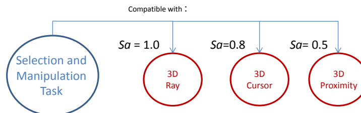
FIGURE 4.13 An example of high level task: selection and manipulation. This task is compatible with three concrete application components. As shown, this compatibility is ranked with scores.
