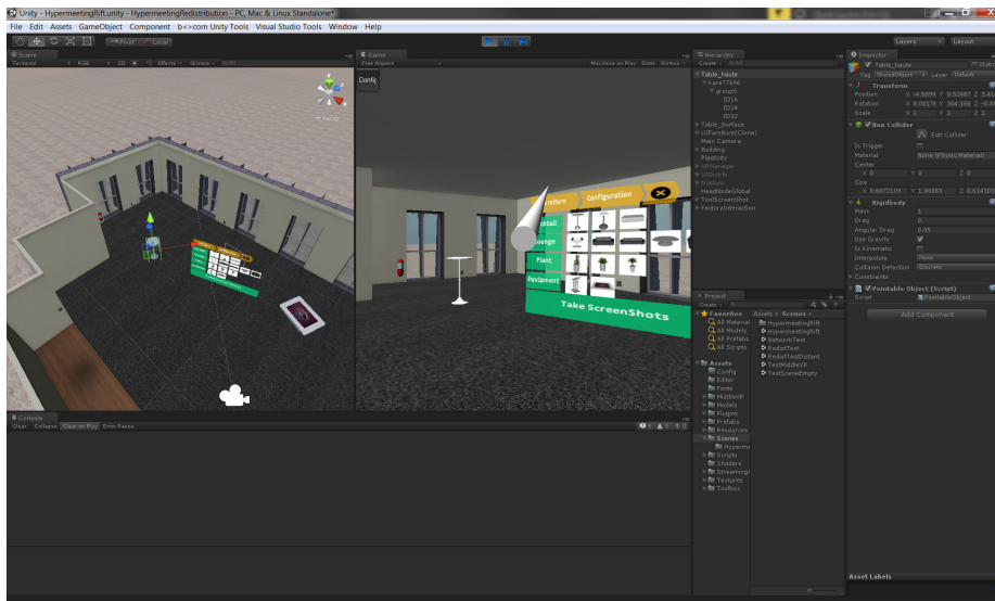
FIGURE 2.18 The Unity3D visual editor. It allows a developer or a designer to visually create and test a 3D applications.
