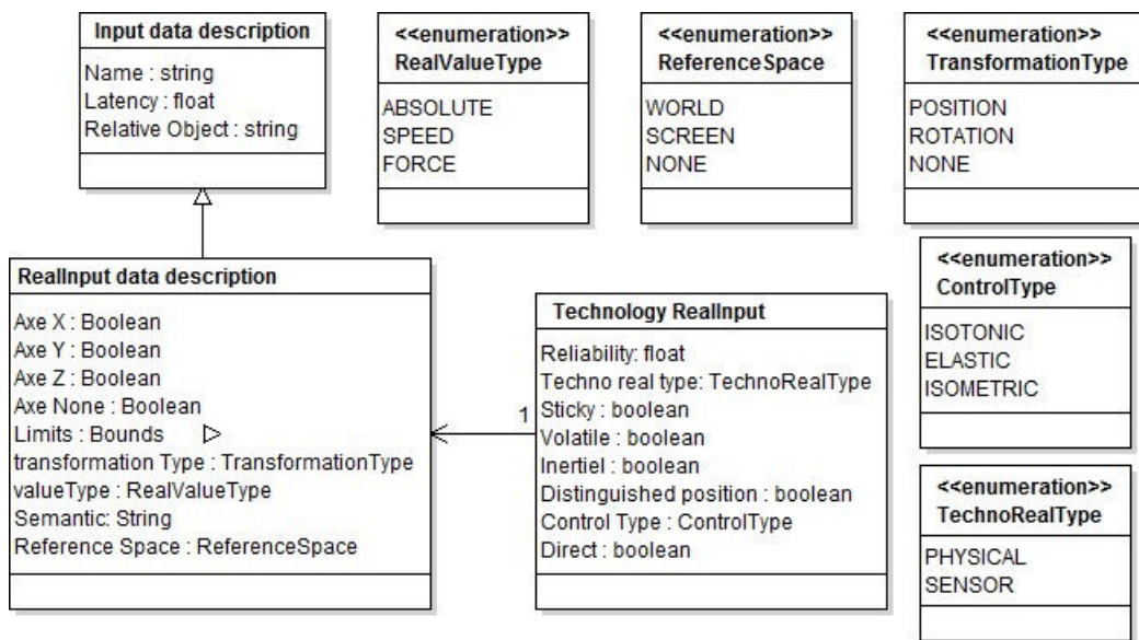
FIGURE 4.7 The description of real value input with two entities: the "data description" and the "technology".
