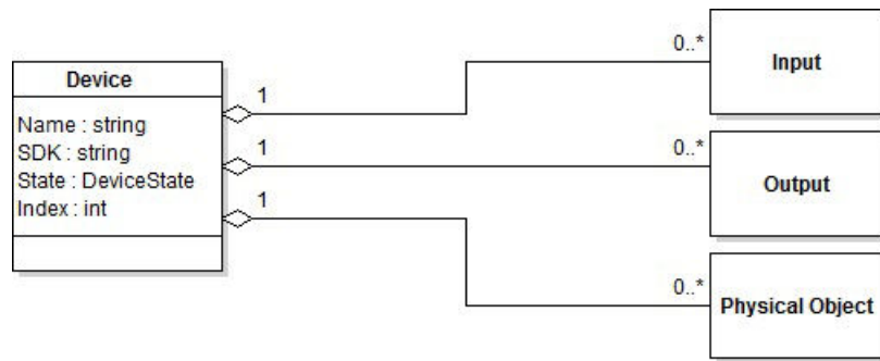
FIGURE 4.6 A device is a set of inputs and outputs as well as a collection of physical objects for its real representation.
