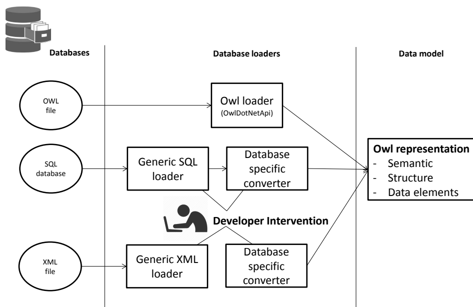
FIGURE 8.3 The 3DPlasticToolkit data model based on a OWL representation and compatible other databases through the implementation of specific converters by the developer.
