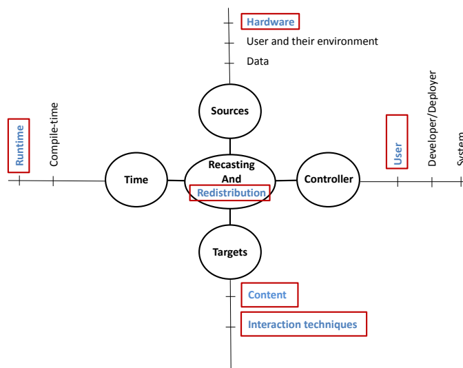
FIGURE 6.1 Regarding our design space problem of plasticity for MR user interfaces, this chapter is interested in allowing the end user to change dynamically the distribution of a MR user interface.
