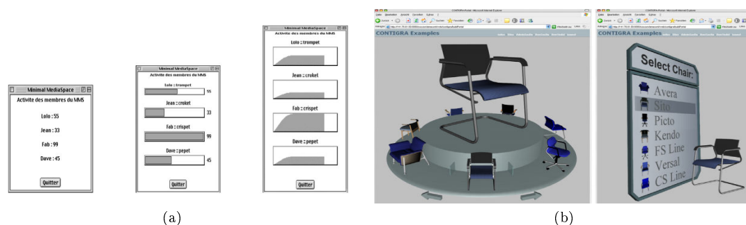
FIGURE 3.1 Two examples of how the layout of an application can be adapted according to the output capabilities of a given platform (here, the screen size). (a) In [Thevenin and Coutaz, 1999], the quantity of information displayed and how this information is represented change according to the screen space variations. (b) In [Dachsel et al., 2006], depending on the screen size the layout of the 3D scene is changed. Here, on the left a ring menu is chosen for a large screen and on the right a floating menu is chosen when the screen is smaller.
