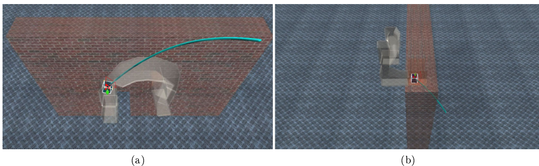
FIGURE 5.11 The Giant has a global view of the scene. He can translate the object with a 3D bent ray.
