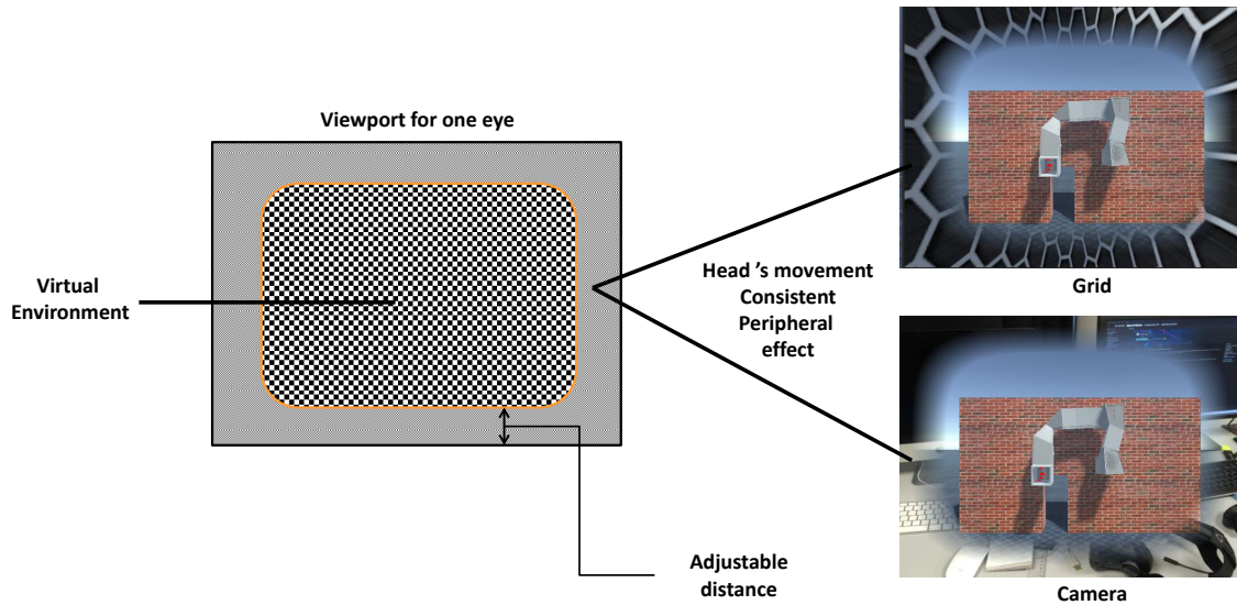
FIGURE 5.15 Our peripheral effect that aims at reducing cybersickness. This effect makes the peripheral view of the user consistent with his/her head movement. It progressively blends the rendered VE on the screen extremities to a grid displayed on a fixed object or to the images acquired by the cameras of a video see-through HMD.
