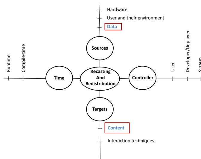
FIGURE 8.1 Regarding our design space problem of plasticity for MR user interfaces, this chapter is interested in adapting the content visualization of an application according to data structure and semantics. At a lower level, we also show that the data can also be combined with the devices properties and the users properties.
