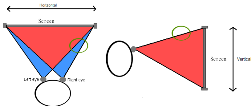
FIGURE 5.4 Top view and side view of camera volumes with horizontally aligned eyes. In red, the area without conflict. In blue, the area where objects will be visible only by one camera (binocular rivalry). The green circle represents a virtual object subject to frame cancellation. In case of non horizontally aligned eyes, the blue area could also be visible on the side view.
