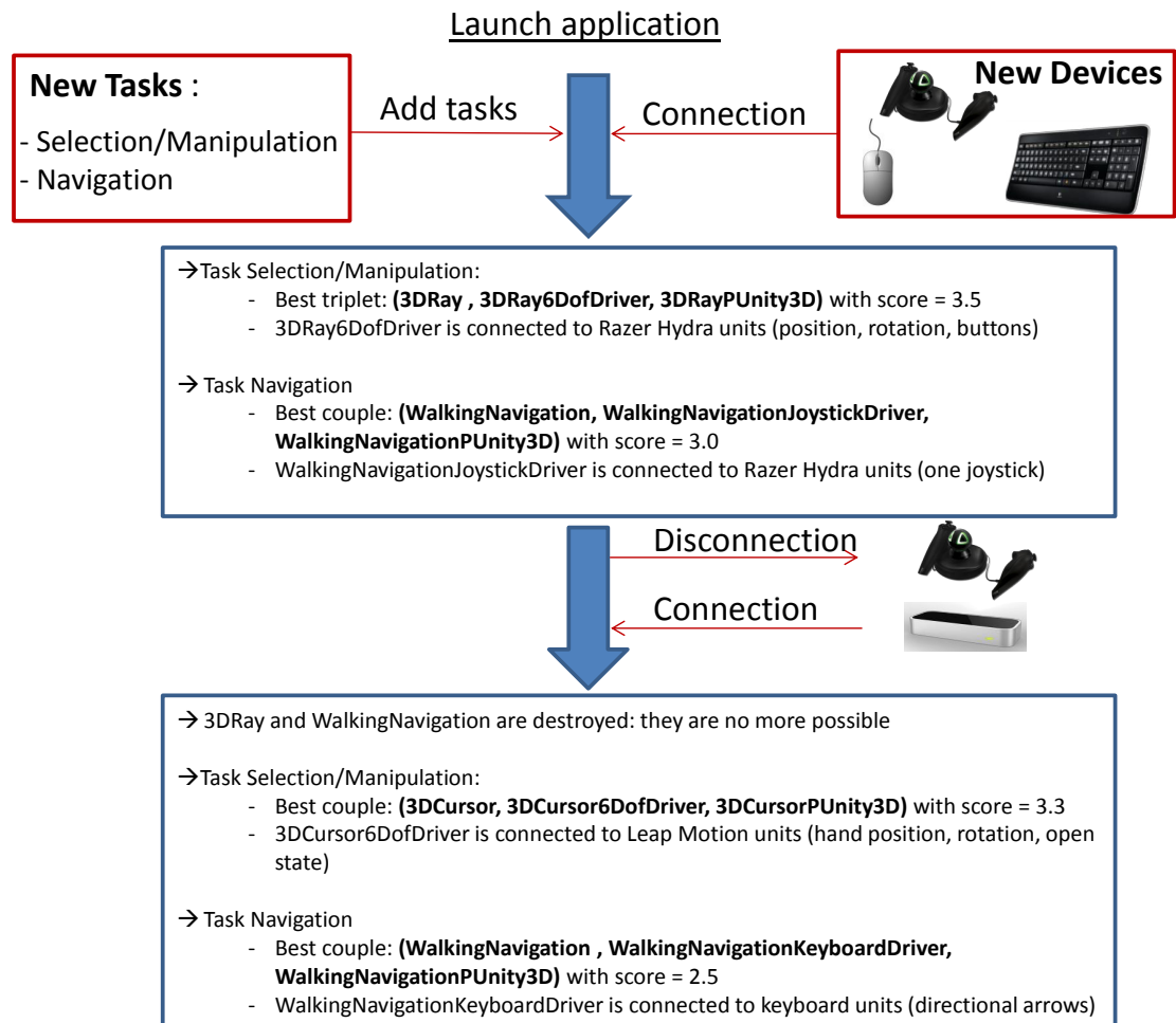
FIGURE 4.14 A usage scenario of the furniture planning application developed with 3DPlastic-Toolkit. It demonstrates how the application can handle context changes: here the replacement of an interaction device by another one. This example represents the adaptation steps that correspond to the transition from the situation illustrated in Figure 4.12a to the one illustrated in Figure 4.12b
