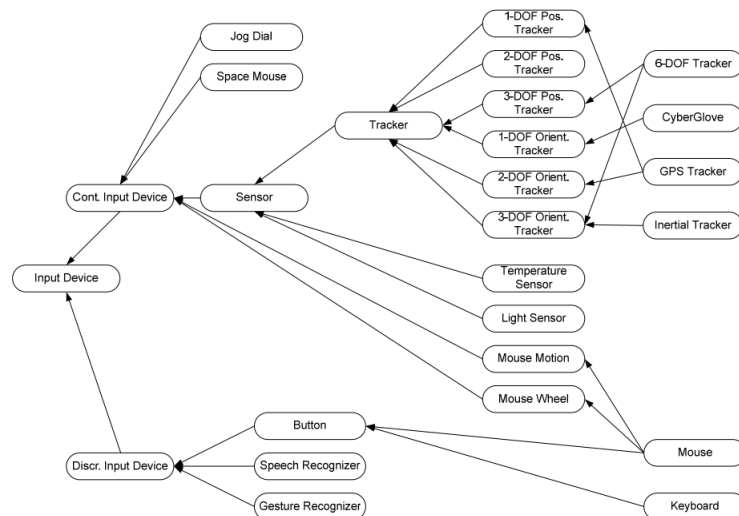
FIGURE 4.3 The hierarchy for input devices proposed by DEVAL [Ohlenburg et al., 2007]. This hierarchy includes a wide variety of input device units including trackers, buttons and gesture recognizers.
