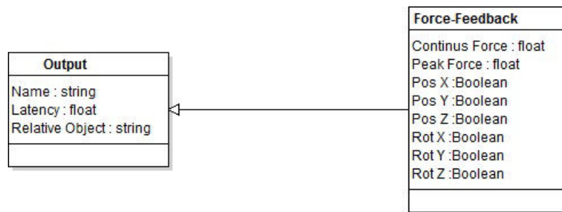
FIGURE 4.8 The description of a force feedback output device
