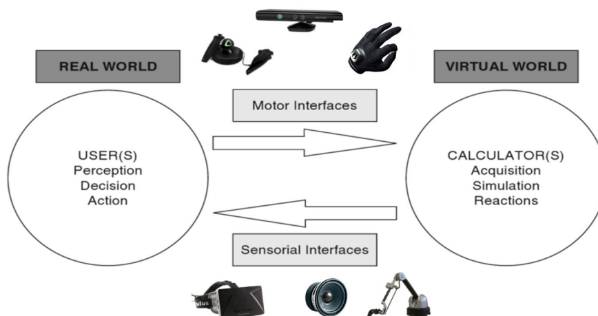
FIGURE 2.2 The "perception, cognition, action" loop involved in Virtual Reality described by Fuchs et al. [Fuchs et al., 2011]
