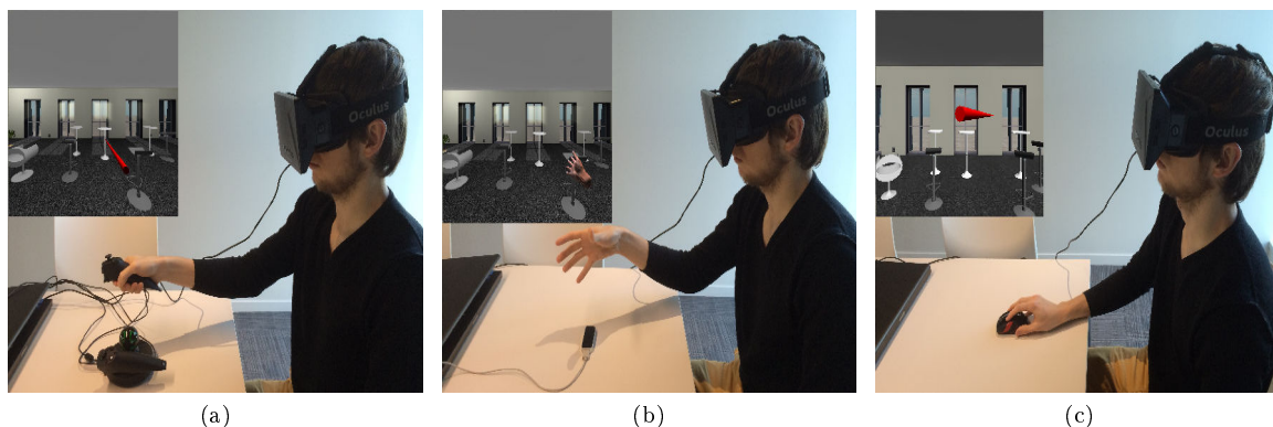
FIGURE 4.12 An illustrative case of the possibilities offered by 3DPlasticToolkit. (a) On a laying-out scenario a user is manipulating the furnitures with a Razer Hydra and a 3D-ray based interaction technique (in red). (b) When the Razer Hydra is unplugged and a leap motion is plugged, the current interaction technique is replaced by cursor based-interaction technique represented with a virtual hand. Usability continuity is ensured with this adaptation. (c) Even without any 3D interaction device the user can still drive a 3D-ray based interaction technique with a mouse, mapping the mouse movements on the ray target.
