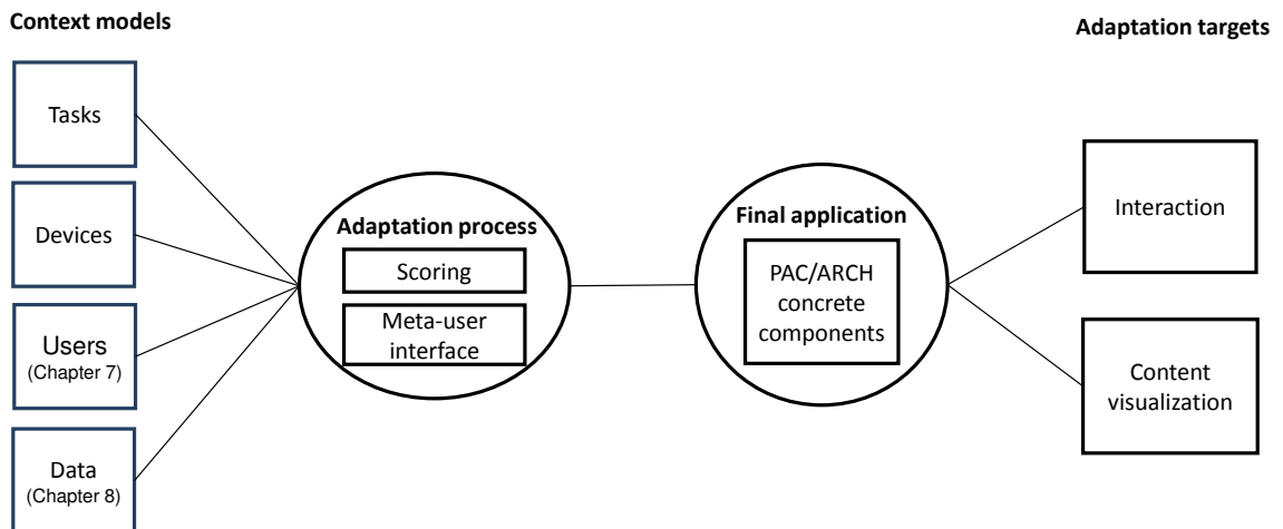
FIGURE 4.5 The 3DPlasticToolkit overview.
