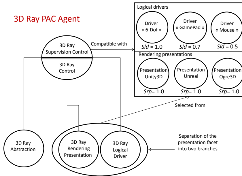
FIGURE 4.11 The PAC agent of the 3D ray-based technique. This agent is compatible with three concrete logical drivers and three rendering presentations. As shown each compatibility is ranked with a score.
