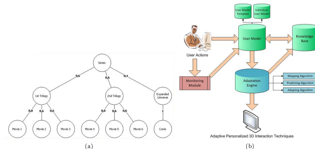
FIGURE 7.2 Two software solutions for user adaptation (a) In [Bonis et al., 2009] a user model is represented by a semantic graph with scores of interest (b) The conceptual framework for adaptation and personalization in VEs proposed by Octavia et al. [Octavia et al., 2009].
