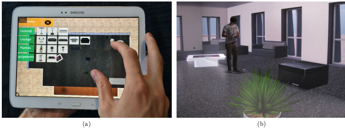
FIGURE 6.6 The redistributed World-In-Miniature: an example of redistribution that demonstrates how D3PART can be used for platform combination.
