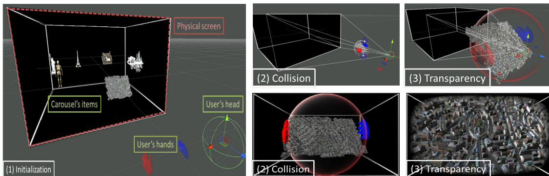
FIGURE 5.9 Illustrative use case (inspired from [Gaucher et al., 2013]) of the manipulation technique smartly merging the two proposed approaches to handle frame cancellation. The user is interacting with a virtual carousel carrying several virtual objects (1). The user can turn the whole carousel and manipulate the front object. The object can be a map that the user can bring very close to him/her with the collision detection-based approach activated (2). Then, he/she can switch the manipulation mode to scale the map and perceive small details with the virtual alpha blended window approach activated (3). The first line shows the scene from an external point of view while the second line is captured from the user's point of view.
