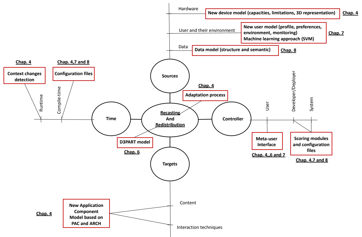
FIGURE 9.1 A summary of our contributions for the creation of plastic MR user interfaces. We also give the associated Chapter for each of these contributions.
