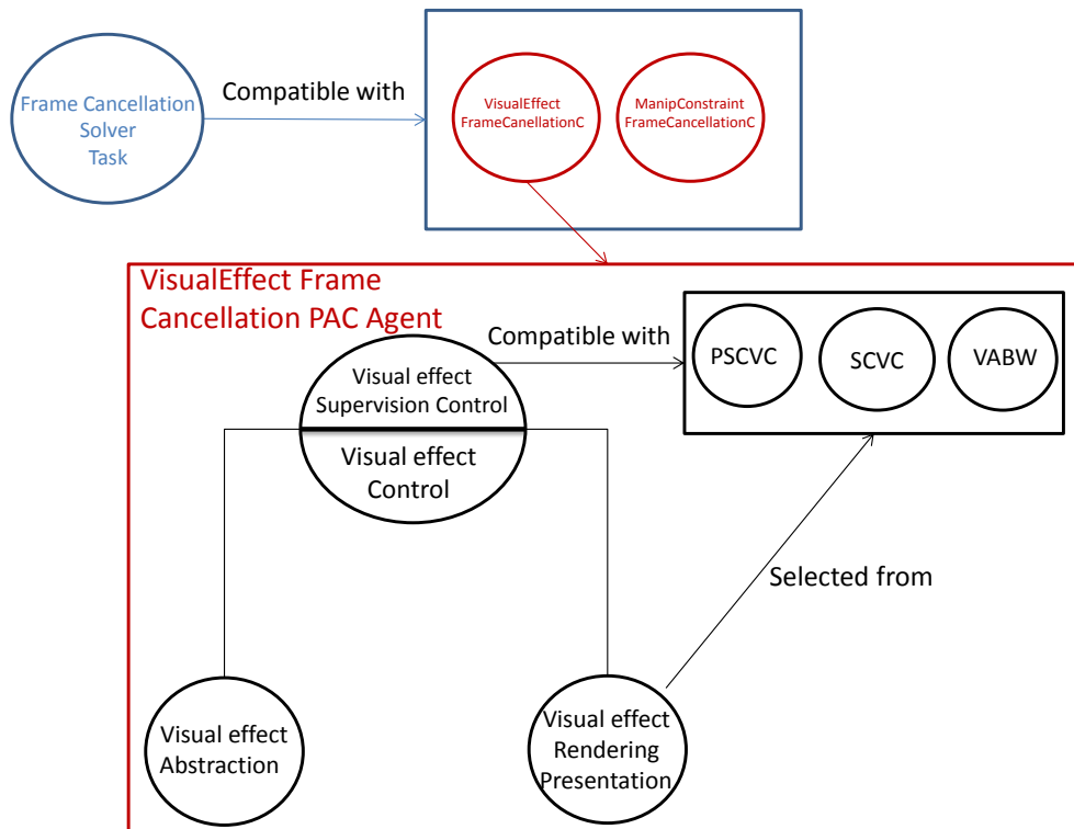
FIGURE 5.8 The "FrameCancellationSolver" task and its compatible application components. Here, the application component that applies a visual effect is described.
