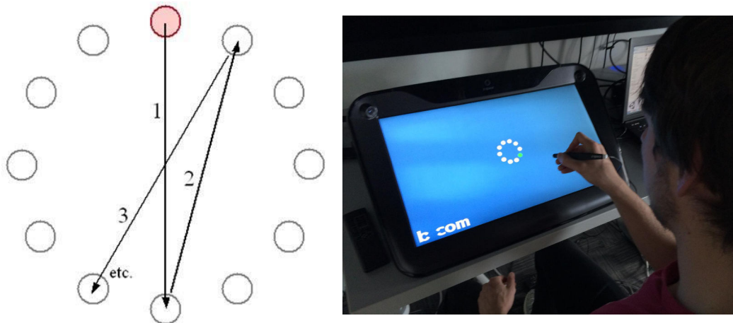
FIGURE 7.3 ISO 9241-9 multi-directional pointing task. The user first selects the highlighted circle, then the next circles to select follow the pattern drawn with the arrows. On the image on the right, a participant is performing this selection test on the zSpace. As shown, the green disk is the one to select.
