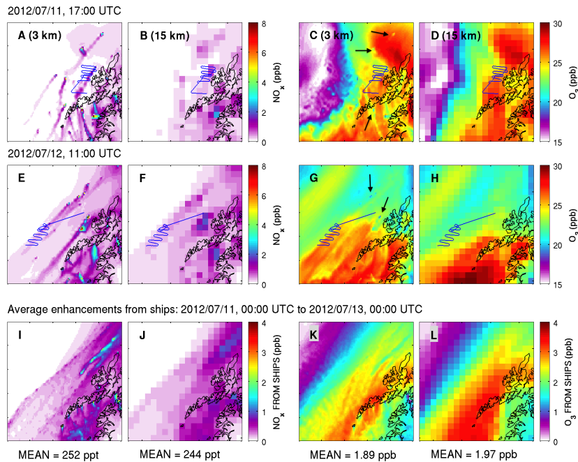
Figure 5-5 – Snapshots of model predicted surface \text{NO}_x and \text{O}_3 from the CTRL3 (3 km) simulation ( a , c , e , g ) and the CTRL (15 km) simulation ( b , d , f , h ) during the flights on 11 and 12 July 2012. Model results for the CTRL3 simulation are shown over the full model domain. CTRL run results are shown over the same region for comparison. The aircraft flight tracks are indicated in blue. On panels ( c ) and ( g ), black arrows indicate several areas of \text{O}_3 titration due to high \text{NO}_x from ships. ( i , j ) \text{NO}_x and ( k , l ) \text{O}_3 2-day average surface enhancements (00:00 UTC 11 July 2012 to 00:00 UTC 13 July 2012) due to shipping emissions, ( i , k ) CTRL3 simulation, ( j , l ) CTRL simulation. The 2-day average enhancements of \text{NO}_x and \text{O}_3 over the whole area are given below each respective panel.
