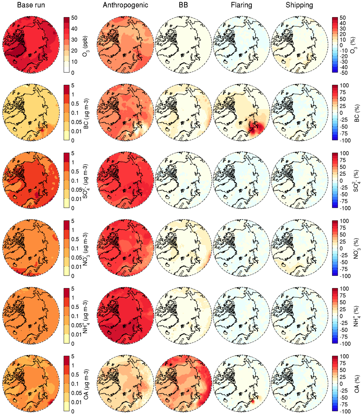
Figure 6-10 – Same as Figure 6-7, for spring (MAM) 2050.
