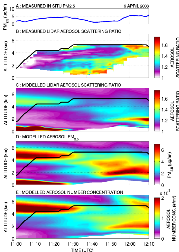
Figure 4-10 – (a) PM_{2.5} measured in situ during the last part of the 9 April 2008 flight, (b) lidar 532 nm pseudo-backscatter ratio measured at nadir during the same portion of the flight (altitude in black, white areas represent topography or cloudy areas where no aerosol data is available), (c) simulated WRF-Chem lidar 532 nm pseudo-backscatter ratio, (d) modeled PM_{2.5} cross section at the same position, and (e) modeled aerosol number concentration cross section at the same position.
