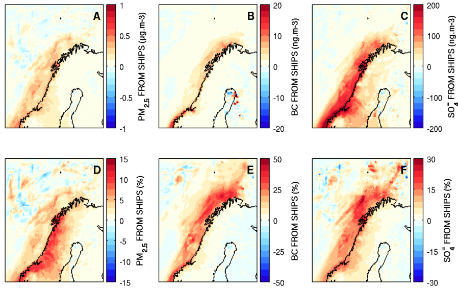
Figure 5-10 – 15-day average (00:00 UTC 11 July 2012 to 00:00 UTC 26 July 2012) of (top) absolute and (bottom) relative surface enhancements (CTRL – NOSHIPS) in (a, d) PM_{2.5} , (b, e) BC and (c, f) SO_4^{2-} due to ship emissions in northern Norway from STEAM2.
