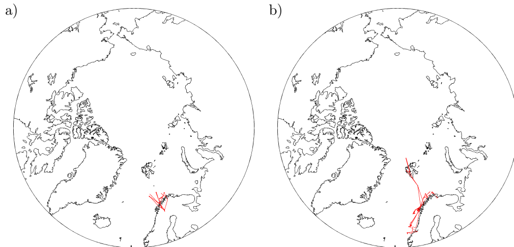
Figure 3-11 – Flight tracks (red) from the (a) POLARCAT-France spring campaign in March–April 2008, (b) ACCESS aircraft campaign in July 2012.
