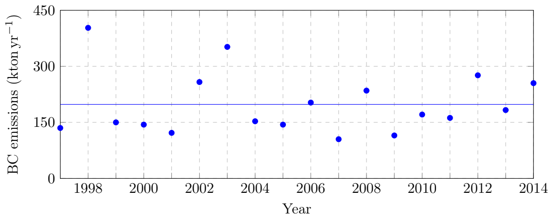
Figure 3-5 – Total boreal (boreal Asia + boreal North America) biomass burning BC emissions ( \text{kton yr}^{-1} ) in the GFED4.1 inventory between 1997 and 2014, individual years (blue markers) and average (blue line).
