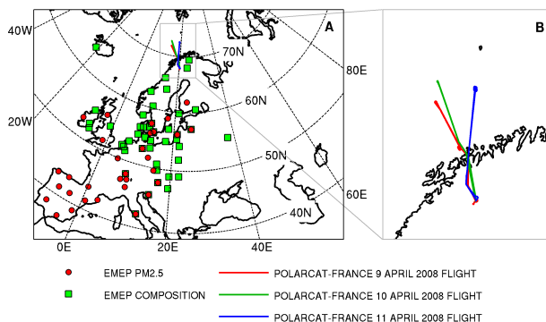
Figure 4-1 – (a) WRF-Chem domain including the location of ground-based EMEP measurement stations used for this study. Stations measuring PM 2.5 are marked by red circles, and stations measuring aerosol composition are marked by green squares. Stations with both measurements are indicated with both symbols. The POLARCAT-France spring flight tracks are shown in red, green, and blue, with a close up over the flight region shown in (b).
