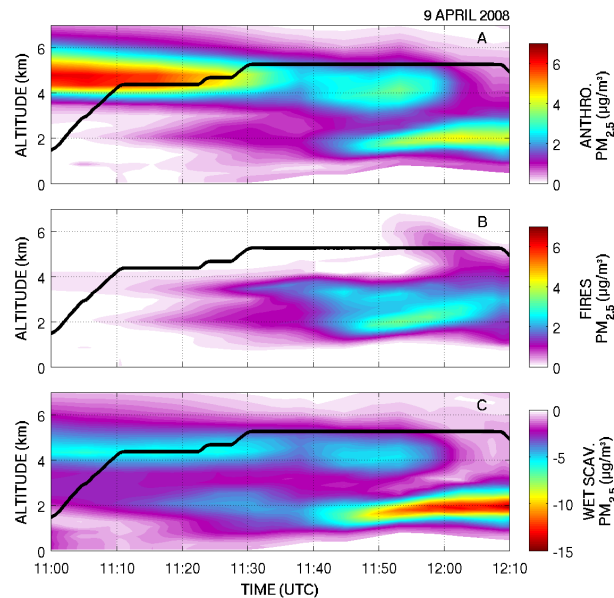
Figure 4-11 – Modeled aerosol cross sections along the flight track (plane altitude in black), showing the sensitivity of the modeled PM_{2.5} to (a) anthropogenic emissions, (b) fire emissions, and (c) wet scavenging.
