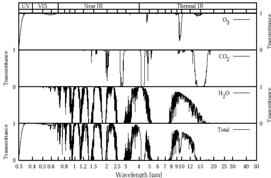
Figure 2-3 – Zenith atmospheric transmission spectrum, (0.3 to 50 μm), and the contributions from the 3 strongest greenhouse gases H 2 O, CO 2 and O 3 . Figure from Petty (2006).
