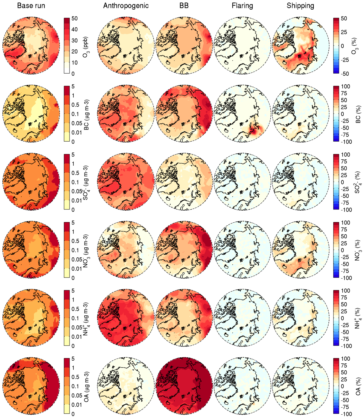
Figure 6-8 – Same as Figure 6-7, for summer (JJA) 2012.
