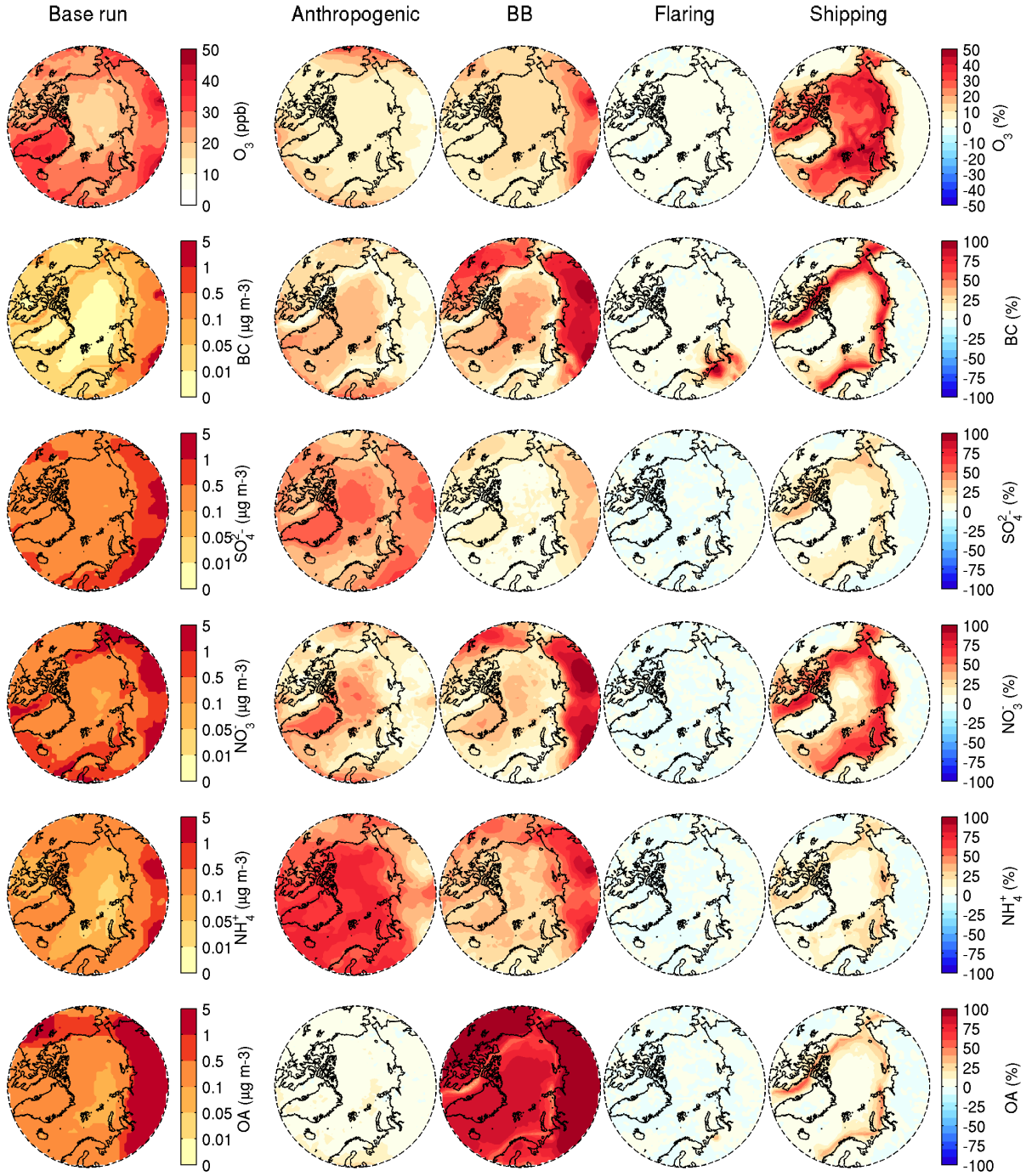
Figure 6-11 – Same as Figure 6-7, for summer (JJA) 2050.
