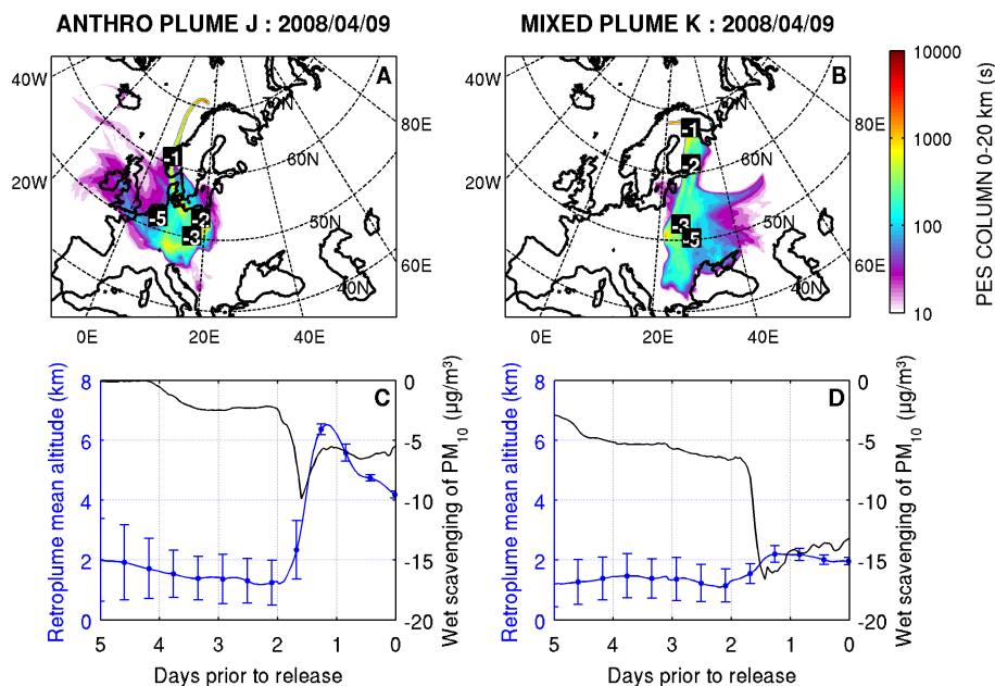
Figure 4-9 – Backward mode FLEXPART-WRF column-integrated PES (a and b), showing typical transport pathways for an anthropogenic plume (left, plume J, originating on 9 April 2008 at 11:19 UTC on the POLARCAT flight track) and a mixed anthropogenic/biomass burning plume (right, plume K, originating on 9 April 2008 at 12:19 UTC on the flight track). Numbers in white indicate the plume age, in days. Panels (c) and (d) show each plume’s mean altitude with rms error bars showing vertical dispersion (blue) and the difference between the CTL PM 10 and the NOWETSCAV PM 10 along transport, indicating wet scavenging events (black).
