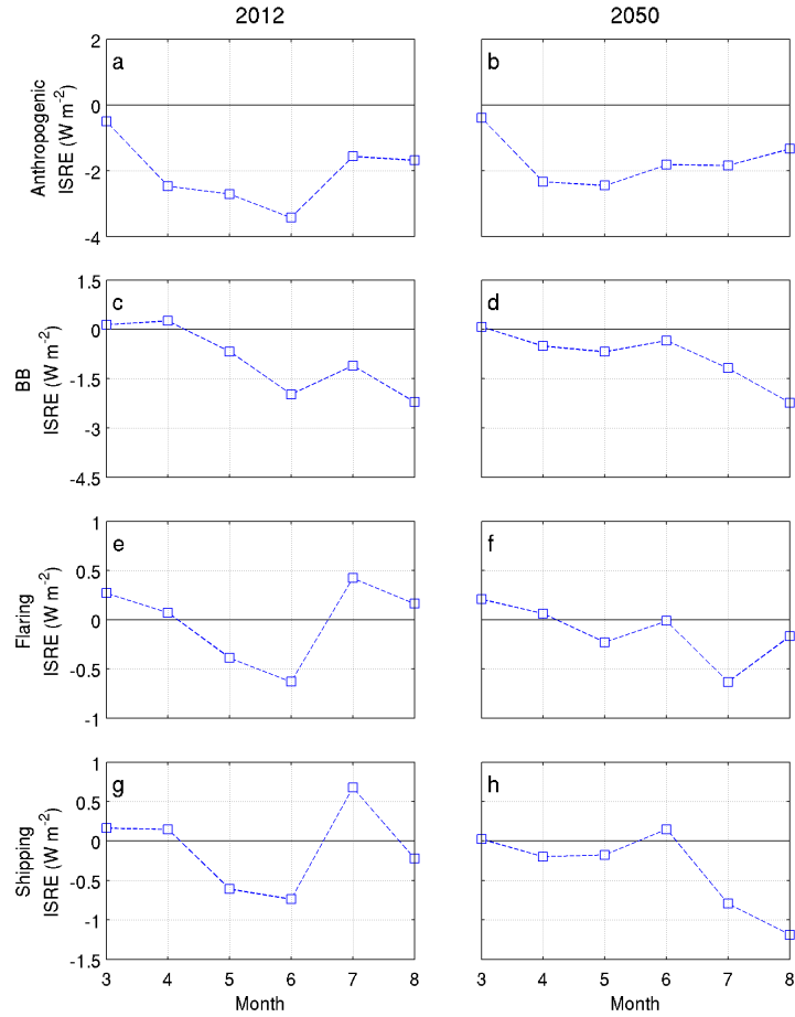
Figure 6-16 – Average Arctic (latitude > 60°N) indirect and semi-direct radiative effects (ISRE) from each source in spring and summer 2012, at top-of-atmosphere. Note differences in scales. The values for Arctic shipping and Arctic flaring are likely to be spurious results due to cloud variability within the model.
