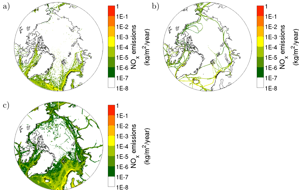
Figure 3-8 – Yearly averaged shipping \text{NO}_x emissions (as \text{NO}_2 ) in the Arctic (latitude > 60^\circ\text{N} ), (a) RCP8.5 (Riahi et al., 2011) in 2010, (b) Corbett et al. (2010) in 2004 and (c) Winther et al. (2014) in 2012.
