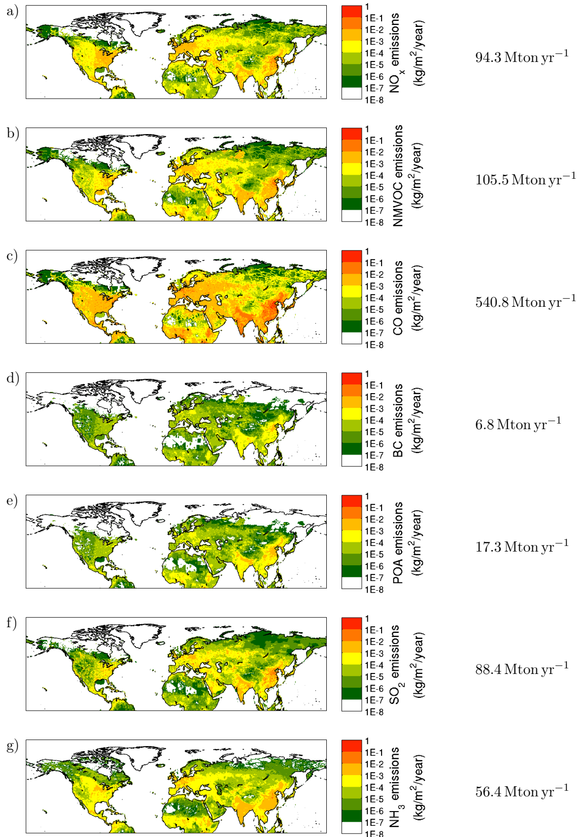
Figure 3-2 – 2010 yearly averaged ECLIPSEv5 anthropogenic emissions in the northern hemisphere (excluding agricultural waste burning) for (a) NO x (as NO 2 ) (b) NMVOC (as NMVOC) (c) CO (d) BC (e) POA (f) SO 2 (g) NH 3 . Global yearly emission totals are indicated on the right of each panel.
