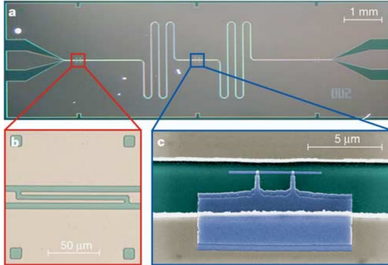
Figure 2.2: Integrated circuit for cavity QED. a) The superconducting niobium coplanar waveguide resonator is fabricated on chip using optical lithography. The stripline resonator consists of the center conductor and two lateral ground planes. The meandering resonator is coupled by a capacitor at each end of the resonator (see b) to an input and output feed line, fanning out to the edge of the chip and keeping the impedance constant. b) The capacitive coupling to the input and output lines and hence the coupled quality factor Q is controlled by adjusting the length and separation of the finger capacitors formed in the center conductor. c) False color electron micrograph of a Cooper pair box (blue) fabricated onto the silicon substrate (green) into the gap between the center conductor (top) and the ground plane (bottom) of a resonator (beige). The Josephson tunnel junctions are formed at the overlap between the long thin island parallel to the center conductor and the fingers extending from the much larger reservoir coupled to the ground plane. Reproduced from [101].
