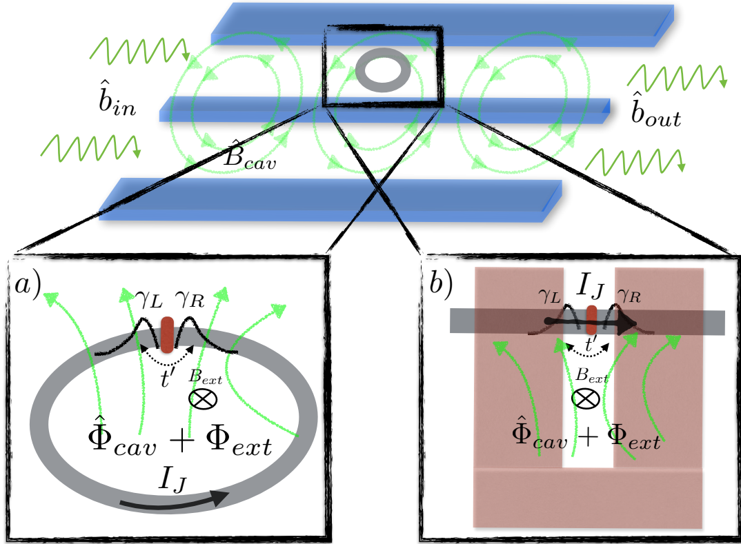
Figure 7.1: Top: A sketch of the combined topological superconductor flux-biased by the cavity. This is probed in the input-output method, and the output signal \hat{b}_{out} is to be compared with the input one \hat{b}_{in} . Bottom: a) A zoom into the topological superconductor in the shape of a ring. The magnetic field of the cavity \hat{B}_{cav} pierces the ring and gives rise to a fluctuating magnetic flux. A perpendicular, external magnetic field B_{ext} is also applied, so that the total flux felt by the electrons in the ring is \Phi_{tot} = \Phi_{ext} + \hat{\Phi}_{cav} . The ring is interrupted by a weak link, that pertains to the hopping strength t' \ll t ( t is the hopping strength within the ring, see the text). In the topological region, there are Majorana fermions on the left ( \gamma_L ) and on the right ( \gamma_R ) of the superconductor, and a Josephson current I_J is flowing within the ring. b) A possible implementation of the geometry in a) based on a spin-orbit nanowire flux-biased in a SQUID geometry. Depicted in light red is a conventional superconducting loop that is interrupted so that there is the Josephson current flowing only through the wire.
