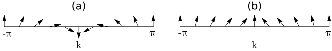
Figure 3.4: The pseudospin vector \hat{h}(k) for parameters: t = \Delta = 1 . a) \mu = -0.5 ; the pseudospin winds once along the Brillouin zone, i.e. w = -1 , b) \mu = -1.5 ; the pseudospin does not wind along the Brillouin zone, i.e. w = 0 .
