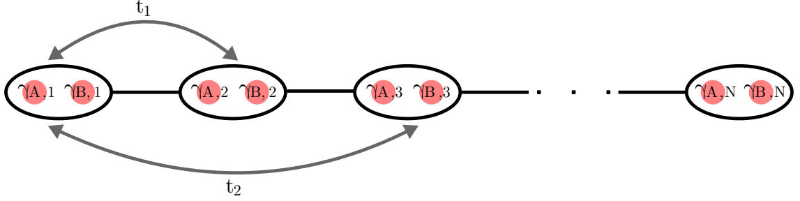
Figure 6.1: Scheme of the extended Kitaev chain. t_1 is the nearest-neighbor hopping amplitude and t_2 is the next-nearest-neighbor hopping amplitude.
