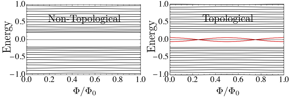
Figure 7.2: The spectrum of the ring as a function of the flux \Phi in the non-topological (left) and topological (right) regions, respectively. In red are depicted the Majorana energy levels that show oscillations with a period \Phi_0 .
