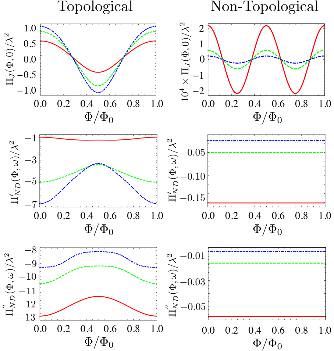
Figure 7.3: Left column (right column), from top to bottom: Dependence of the Josephson, non-diagonal real, non-diagonal imaginary susceptibilities respectively, in the topological (non-topological) region on the magnetic flux \Phi/\Phi_0 for f_M = 0 . The red, green, and blue lines correspond to \mu = -1.5 ( \mu = -2.5 ), \mu = -1 ( \mu = -3 ), and \mu = -0.5 ( \mu = -3.5 ), respectively. The phase transition point is at \mu = -2 . The parameters for the plots are \Delta = 0.1 , t' = 0.2 , N = 50 , and all energies are expressed in terms of t = 1 .
