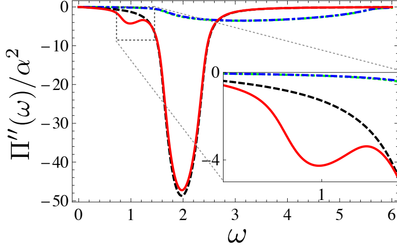
Figure 5.6: Dependence of \Pi''(\omega) on the cavity frequency \omega for N = 50 . The full-red (dashed-black) line corresponds to the susceptibility in the topological regime for \mu = -0.2 , while the dot-dashed-blue (dotted-green) corresponds to the non-topological regime with open (periodic) BCs with \mu = -1.8 , so that the effective gap is the same \Delta_{\text{eff}} = \|\mu\| - t = 0.8 in both regions. Inset: a zoom in the region where the Majorana peak emerges. For all the plots we used t = \Delta = 1 , and all energies are expressed in terms of t .
