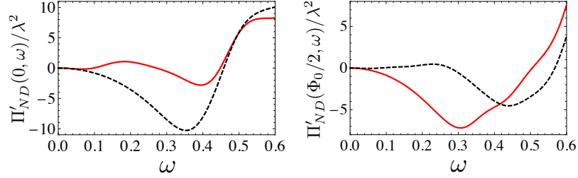
Figure 7.5: Dependence of the real part of the non-diagonal susceptibility on the frequency \omega for two values of the external flux, \Phi = 0 (left) and \Phi = \Phi_0/2 (right), and for the two parity states f_M = 0 (dashed-black) and f_M = 1 (full-red) lines, respectively. The parameters for the plots are: \mu = -0.5 , \Delta = 0.1 , t' = 0.5 , N = 50 , and all energies are expressed in terms of t = 1 .
