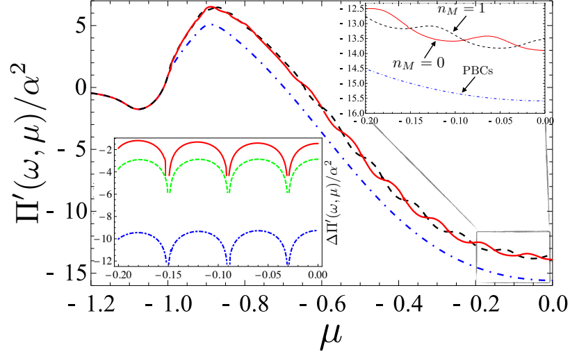
Figure 5.4: Dependence of \Pi'(\omega, \mu) on the chemical potential \mu . The blue (dot-dashed), red (full), and the black (dashed) lines correspond to the susceptibility for PBCs, OBCs for parity n_M = 0 , and OBCs for parity n_M = 1 , respectively. Lower Inset: the relative strength of the susceptibility \Delta\Pi' = 2|(\Pi_{\text{BM}}^+ - \Pi_{\text{BM}}^-)/(\Pi_{\text{BM}}^+ + \Pi_{\text{BM}}^-)| as a function of \mu in logarithmic scale, for \Delta = 0.1 (red-full), \Delta = 0.2 (green-dashed), and \Delta = 0.3 (blue-dot-dashed). The size of \Delta\Pi' is exponentially reduced as a function of \Delta . We used N = 50 , \omega = 0.2 , \Delta = 0.1 , t = 1 , and all energies are expressed in terms of t .
