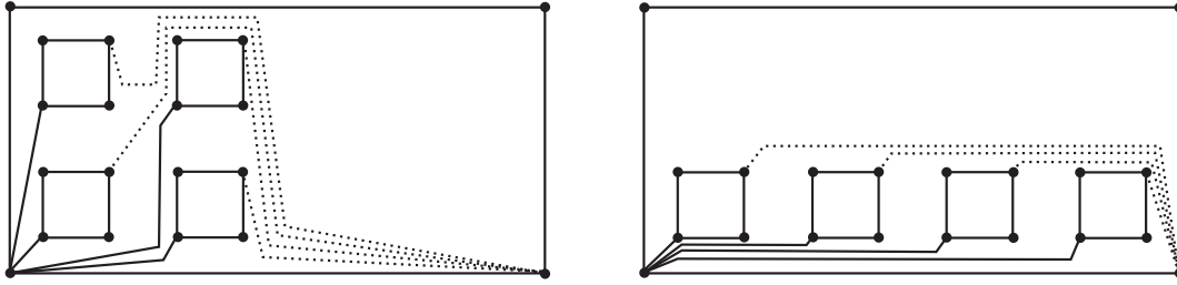
FIGURE 20. Graphs \mathbb{G}_1 and \mathbb{G}_2 .
