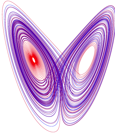
Figure 1.2: A solution in the Lorenz attractor.
