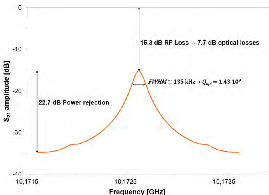
Figure II-17 RF transmission characteristics of the 100m long immunized fiber ring resonator.
