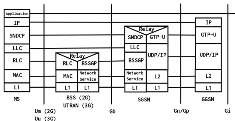
Figure 1.4 : Encapsulation GTP [3]
