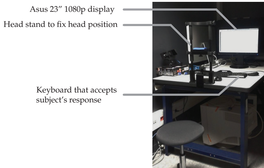
FIGURE 4.6: Experimental setup.
