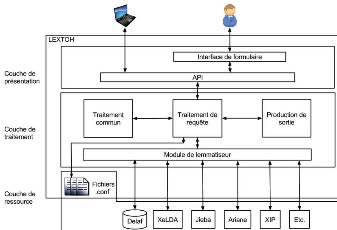
Figure 75 : Architecture de LEXTOH
