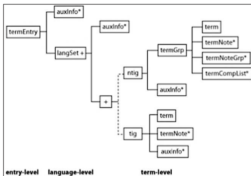
Figure 41 : Structure TBX standard
