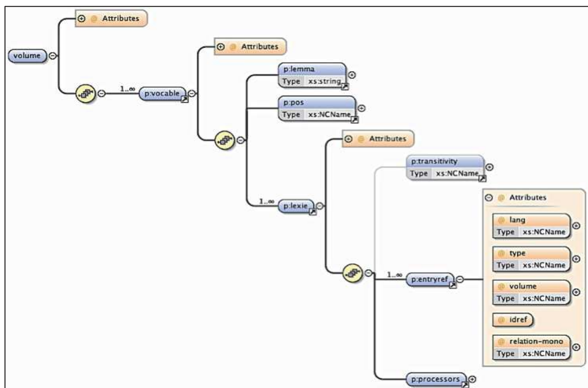
Figure 23 : Microstructure de volume monolingue de COMMONUNLDICT
