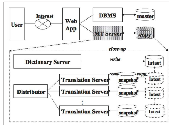
Figure 3 : Architecture de YAKUSHITE.NET
