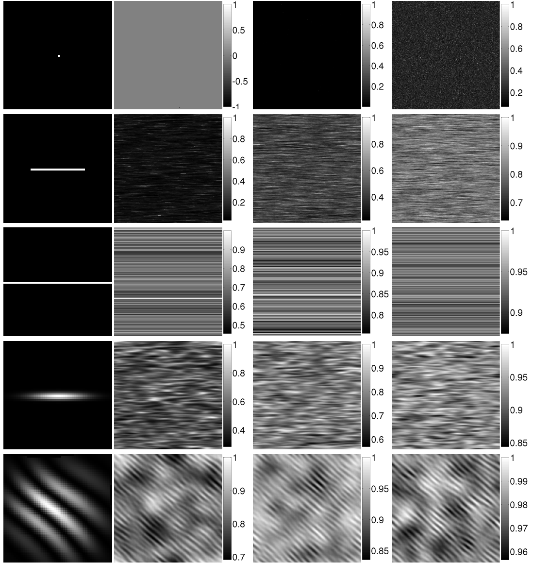
Figure 6.2 – Examples of a random process of type 1 \otimes (\psi \star \lambda) , where \lambda[i] \sim \text{Gamma}(a, a) are independent random variables. First column: filter \psi . From the second to the last column: realizations with different values of a : 0.2, 1.1 and 2.
