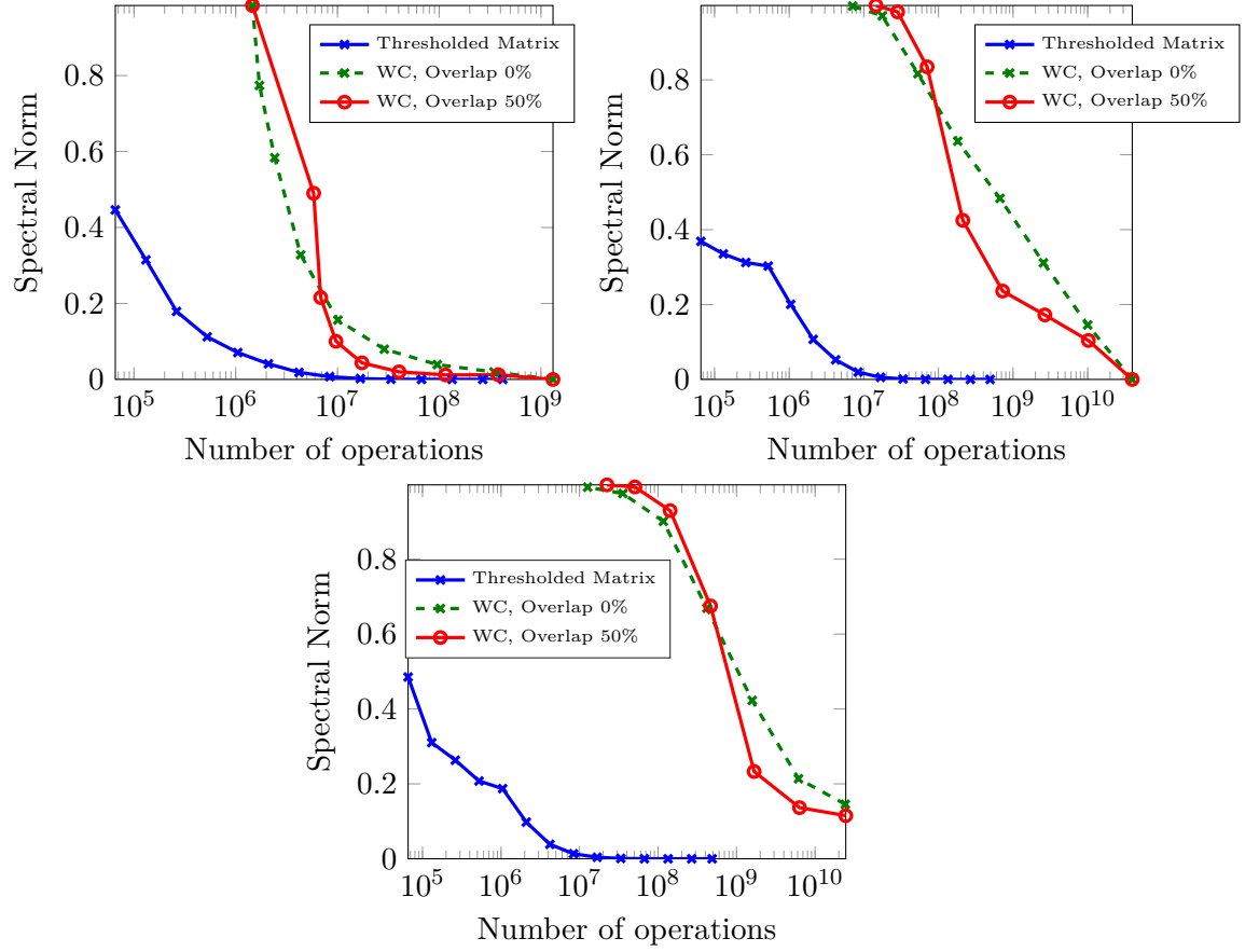
Figure 3.10 – The operator norms \|\mathbf{H} - \tilde{\mathbf{H}}\|_{2 \rightarrow 2} are displayed for the three proposed kernels. (Left: kernel Figure 3.8a, middle: kernel in Figure 3.8b, right: kernel in Figure 3.8c). Norms are plotted with respect to the number of operations needed to compute \tilde{\mathbf{H}}\mathbf{u} . The abscissas are in log scale.
