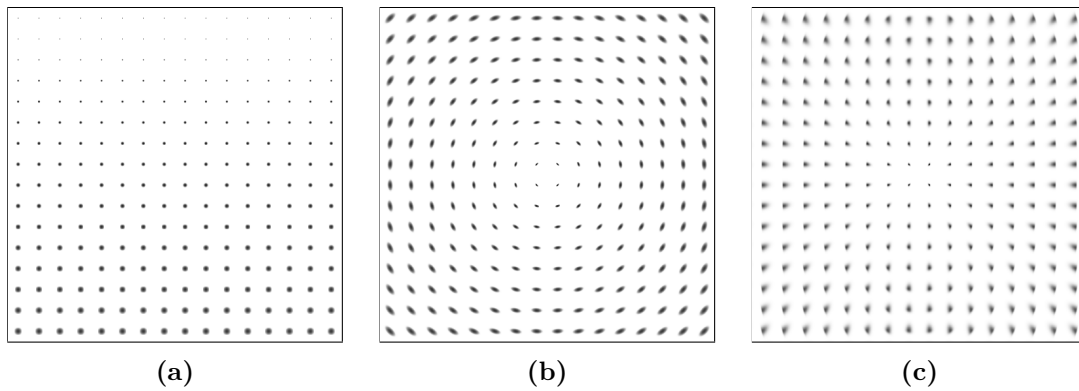
Figure 3.8 – PSFs maps used in the paper. The PSFs in Figure 3.8a are Gaussians with equal variances increasing in the vertical direction. The PSFs in Figure 3.8b are anisotropic Gaussians with covariance matrices that depend on the polar coordinates. The PSFs in Figure 3.8c are based on paper [212].
