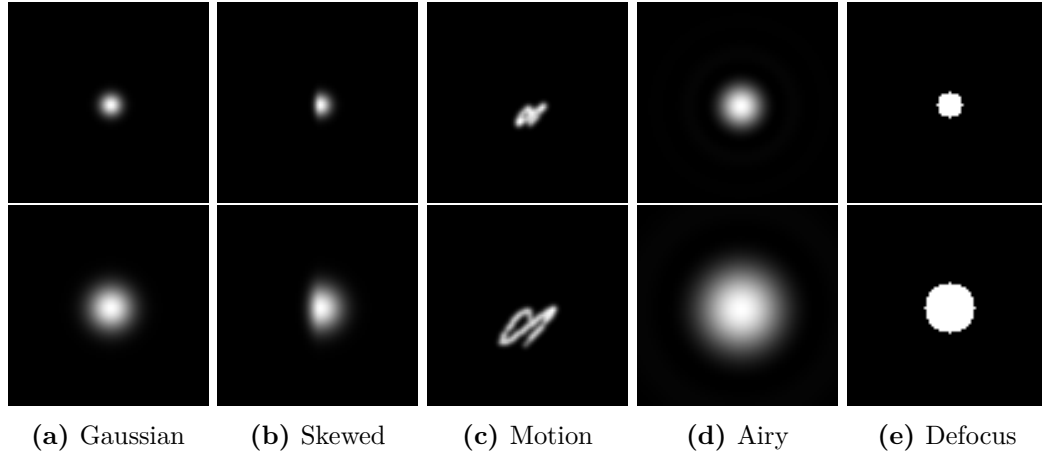
Figure 4.10 – The different blurs used to analyze the method’s efficiency.
