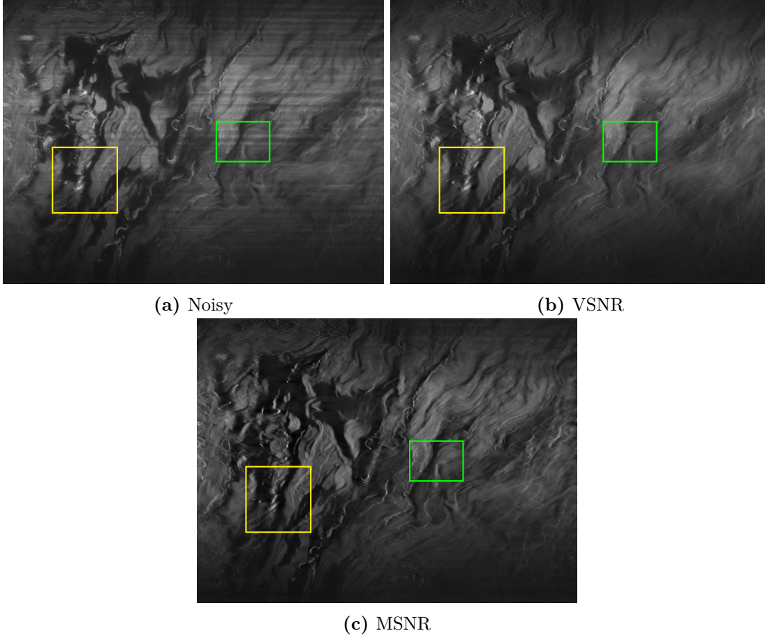
Figure 6.8 – Denoising experiment on real data: 1040 \times 1390 . The degraded image is a XY plane of an skin dermis acquired using a SPIM. The image is used here by courtesy of Claire Jardet from Genoskin. The iterates stabilize visually after 300 iterations. Computing time GPU: 3.3s (about 11ms per iteration)
