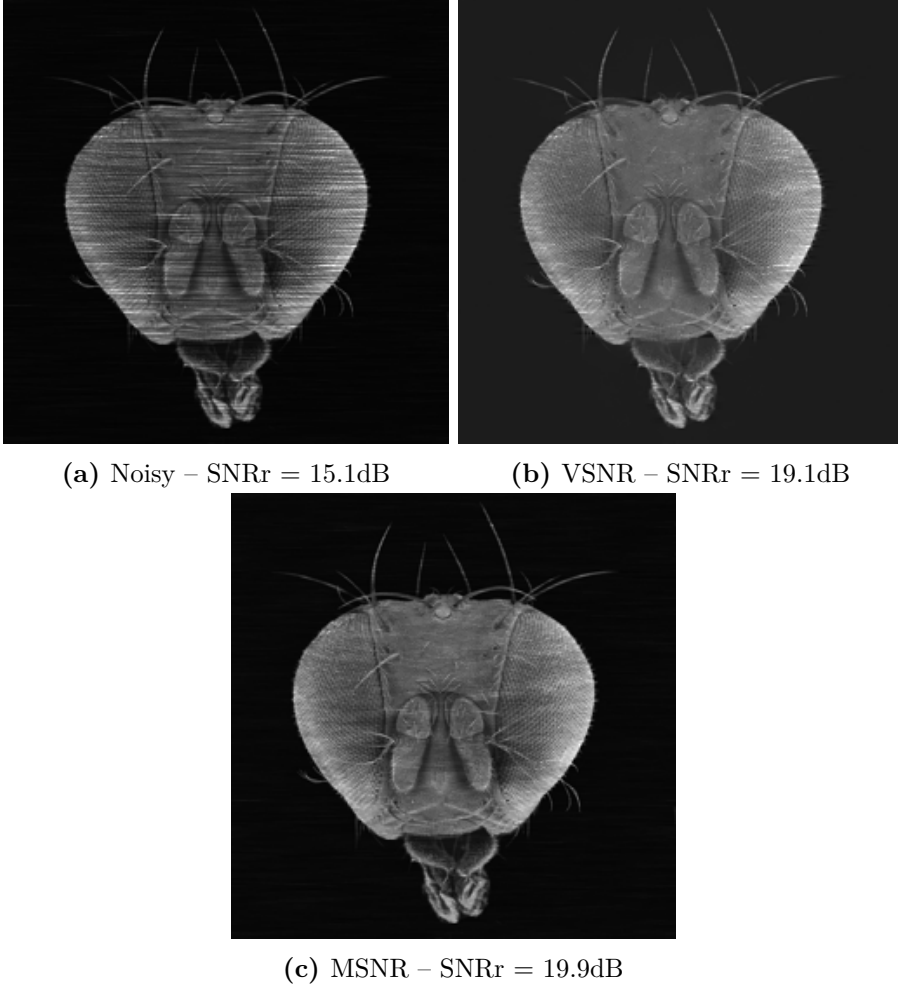
Figure 6.6 – Denoising simulation with structured noise. The image is corrupted with \psi a segment and a = 1.1 see Figure 6.3 bottom-left. The \text{SNRr} is stable after 50 iterations. Computing time GPU: 0.03s.
