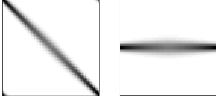
Figure 5.2 – Two representations of an integral operator H acting on L^2([0, 1]) . The kernel is defined by K(x, y) = \frac{1}{\sqrt{2\pi\sigma(y)}} \exp\left(-\frac{1}{2\sigma(y)^2}|x - y|^2\right) , where \sigma(y) = 0.05(1 + 2\min(y, 1 - y)) . Left: kernel representation (see equation (5.1)). Right: SVIR representation (see equation (5.4)).
