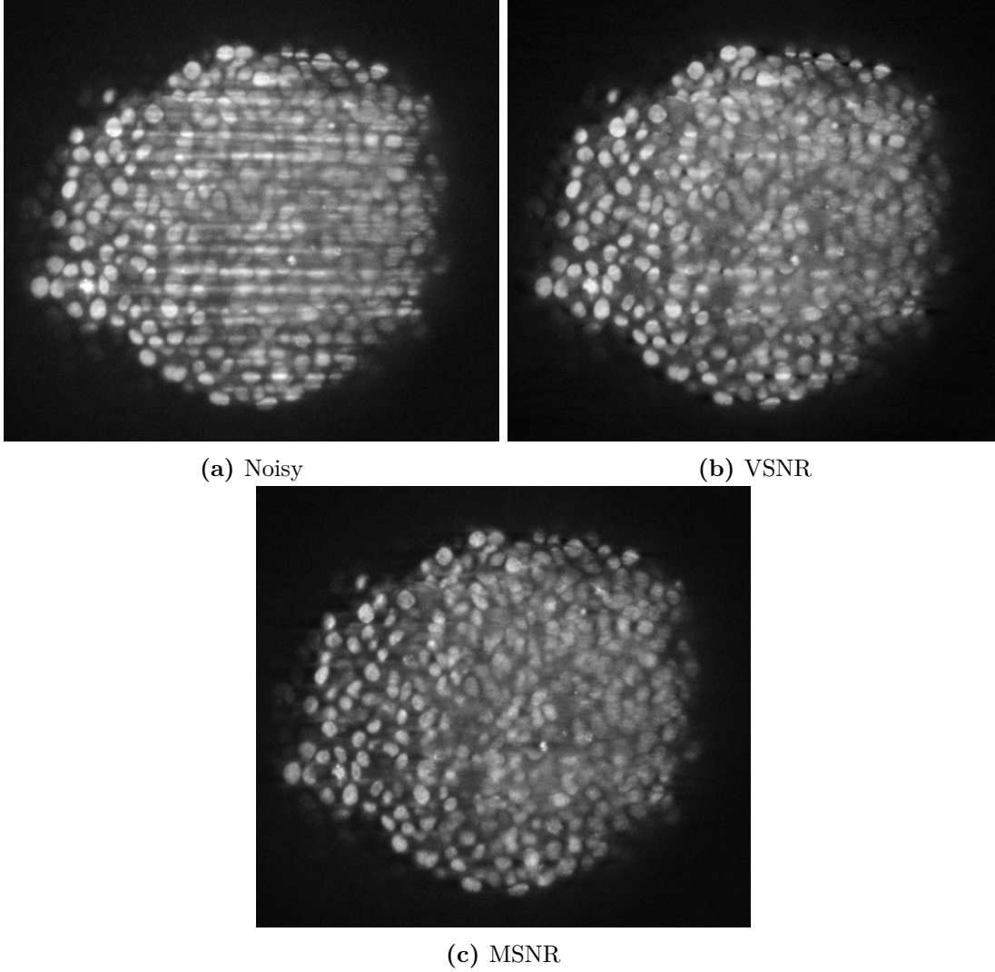
Figure 6.10 – Denoising experiment on real data : 499 \times 561 . The degraded image is a XY plane of spheroid acquired using a SPIM. The iterates stabilize visually after 500 iterations. Computing time GPU: 3s (about 6ms per iteration)
