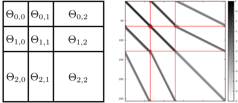
Figure 4.2 – Left: structure of \Theta . Right: \Theta in \log_{10} -scale when H is a convolution with a Gaussian kernel.
