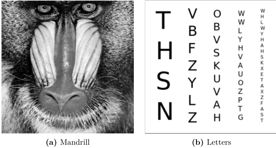
Figure 3.7 – The two images of size 256 \times 256 used in these numerical experiments
