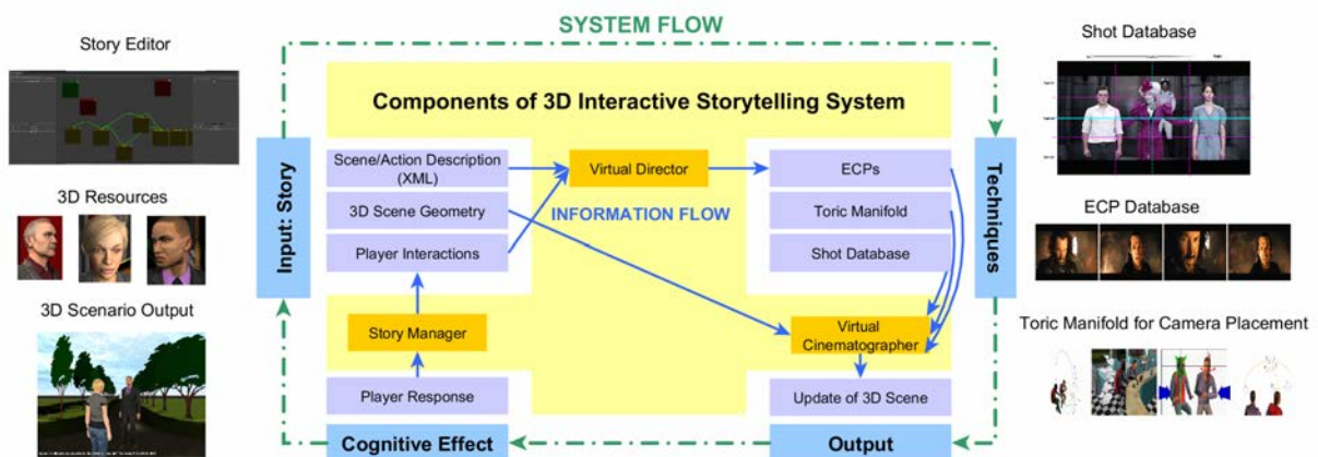
Figure 5.1 – This workflow shows how our system follows the cinematography system for storytelling we outlined in Chapter 2. The green arrows present the overall flow of the system, and the blue ones represent the flow of information on the geometry, story, and communicative goals.
