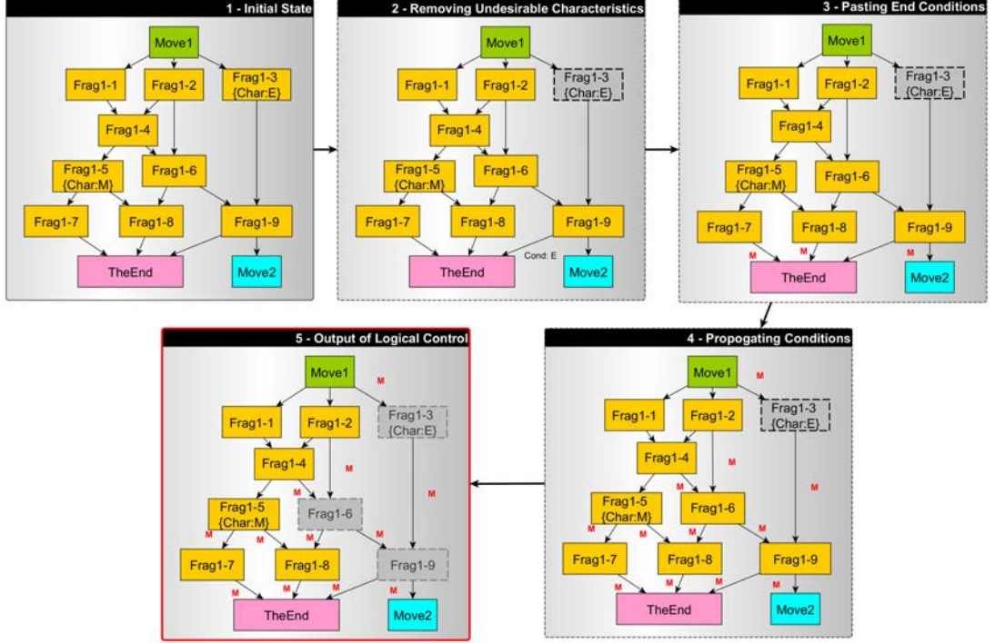
Figure 3.3 – Graph traversal algorithm for logic control. Given an authored move and authorial goal \neg E \wedge M (“(NOT Evil) AND Magic”), the algorithm (1) removes plotpoints contradicting the goal (E), (2) pastes the goal (M) as an end precondition, (3) reverses and (4) propagates the preconditions on all edges, and (5) removes dead ends. As a result, remaining paths ensure the story logic as well as authorial goals.
