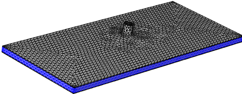
FIGURE 4.5 – Maillage de la structure composite sandwich.
