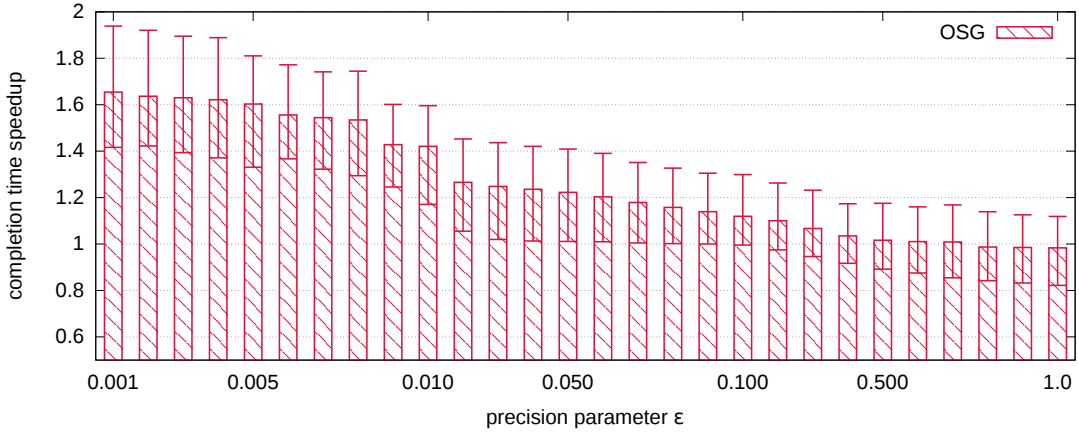
Figure 7.26 – Speed up \Lambda_L^{OSG} as a function of the precision parameter \epsilon ( i.e. , number of columns c = e/\epsilon ).
