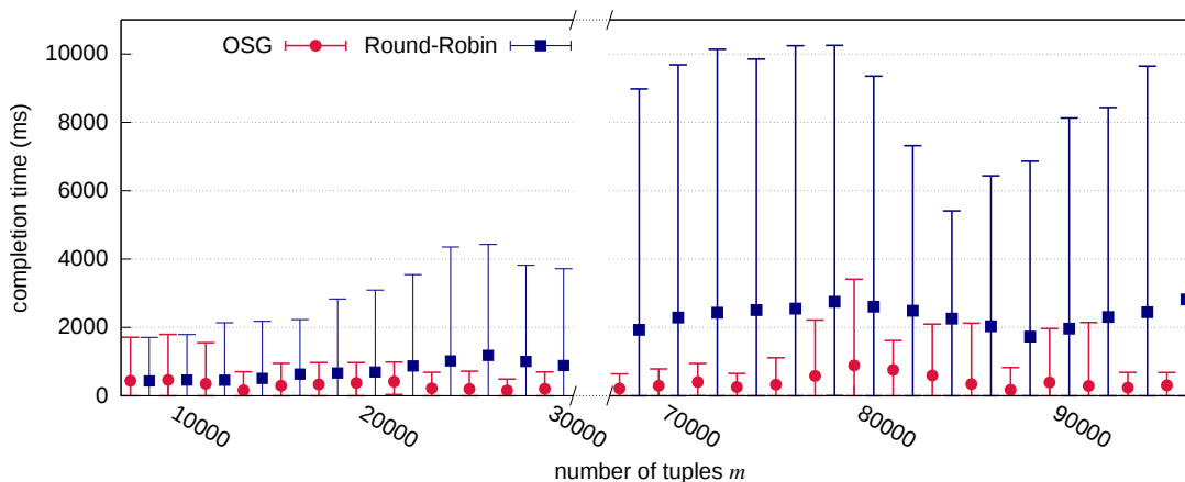
Figure 7.27 – Simulator per tuple completion time time-series.
