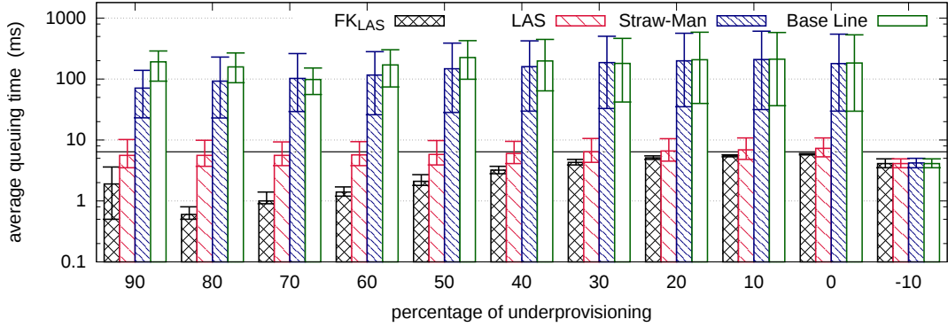
(a) Average queuing time \bar{Q}
