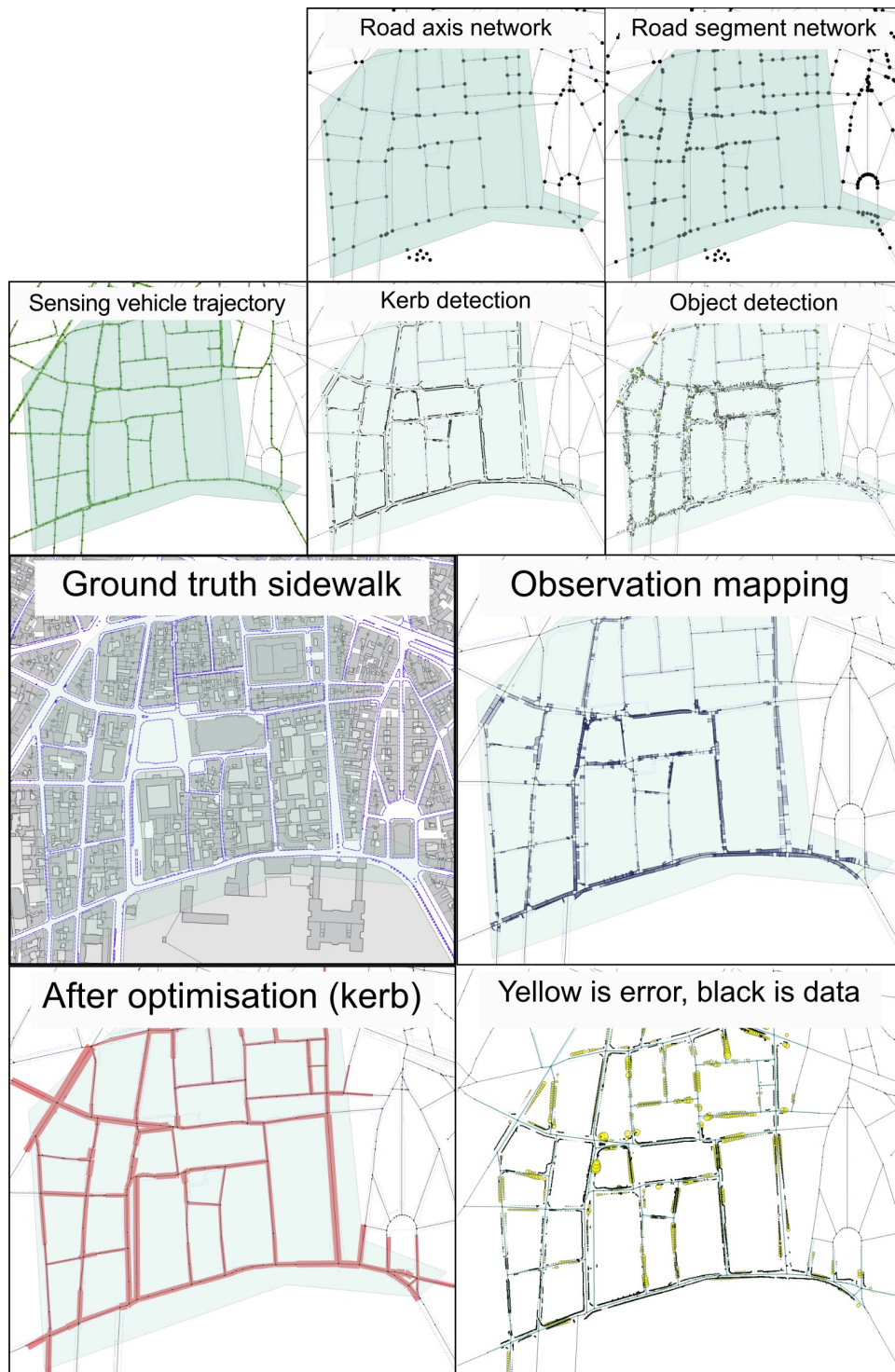
Figure 132: Optimisation parameters are the street axis network and width attribute, which get split into a road segment network. A street sensing vehicle detects kerbs and objects, which are processed into observations, and matched to street segments. Non-linear least square optimisation fits the parameters to these observations.
