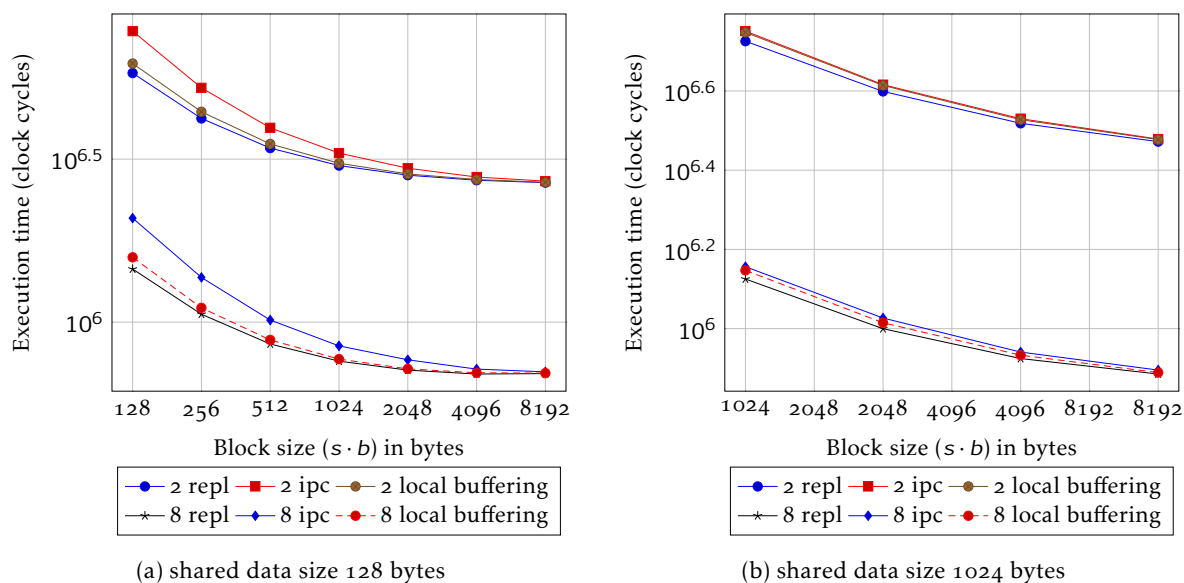
Figure 8.15 – Measurements for shared data in computation regime
