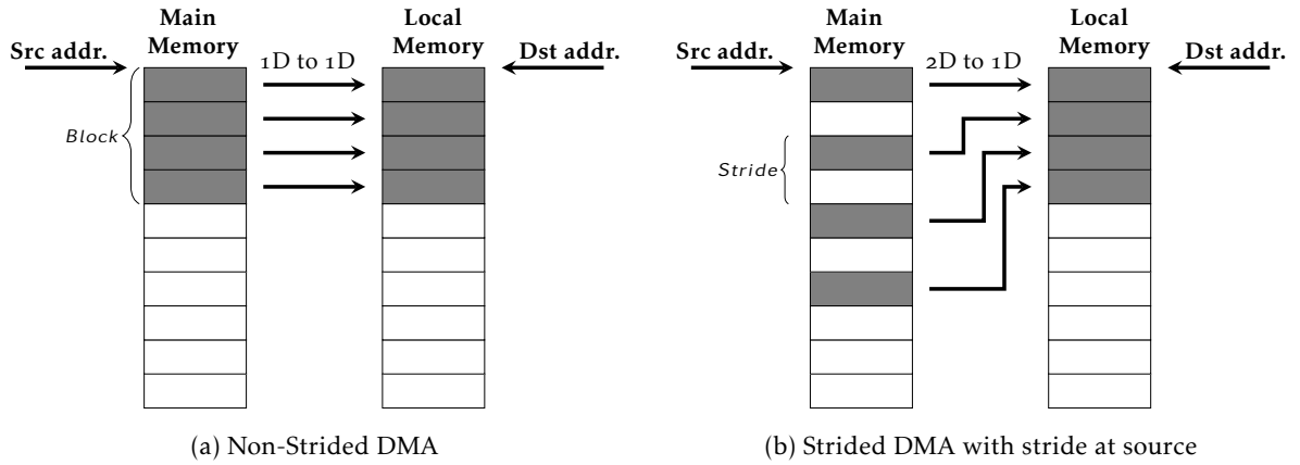
Figure 3.7 – DMA transfers
