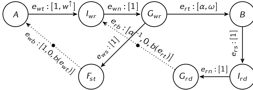
Figure 7.6 – Buffer aware graph model for a channel with DMA
