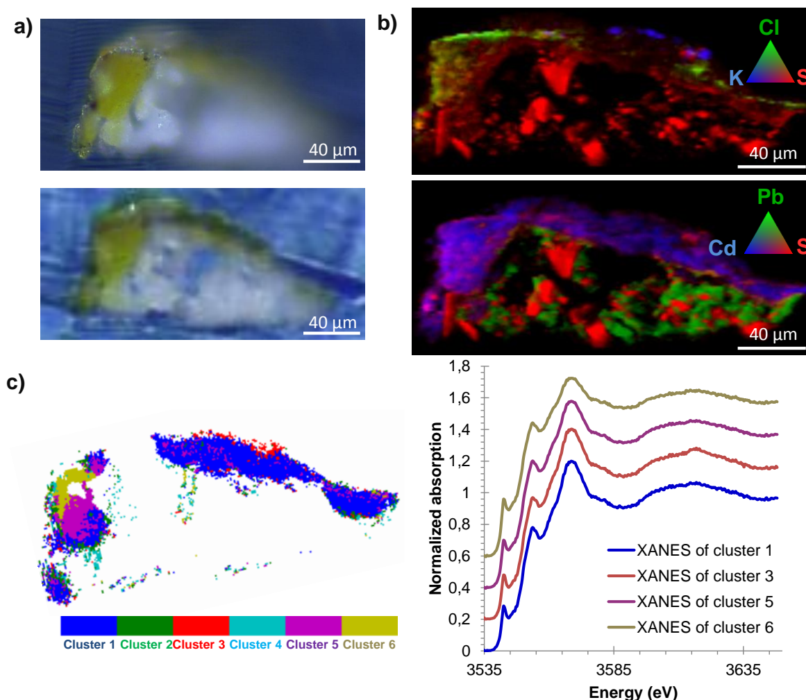
Figure 5-13 : a) Visible light microscope images of S111 10 μm thick thin-section; b) μXRF elemental maps of Cl, K, S, Cd and Pb acquired at 3.7keV(step size: 0.7 \times 0.7 \mu\text{m}^2 ); c) Results of k-means clustering combined with PCA analyses of FF-XANES acquisition at Cd L III -edge (step size: 0.7 \times 0.7 \mu\text{m}^2 ).
