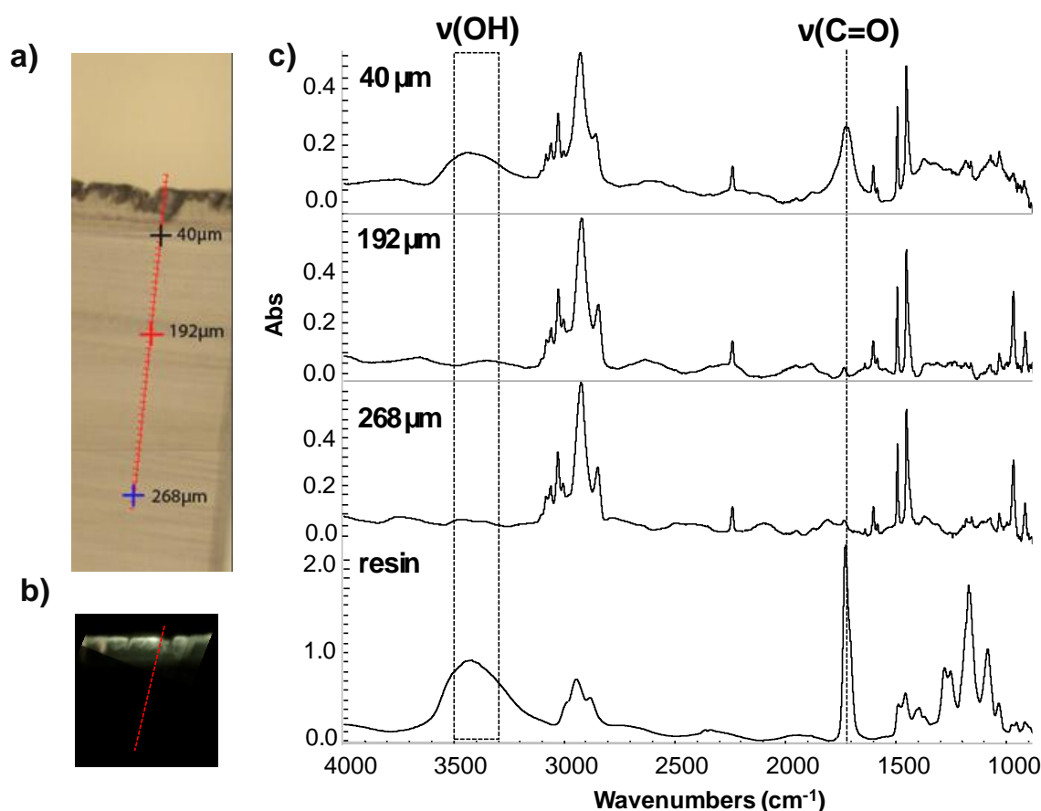
Figure 5-17: SR \mu\text{FTIR} study of the oxidation of an ABS model film (sample exposed to UV-irradiation for 1000 hours); a) Visible light microscope image of a 2 \mu\text{m} thin-section prepared following the SES method, b) UV light microscope images of 1000h aged ABS sample on the left, and of pure resin thin-section (2 \mu\text{m} ) on the right c) FT-IR spectra acquired at different positions corresponding to three different depths from the sample surface and one spectrum characteristic of the absorption of a resin 2 \mu\text{m} thin-section.
