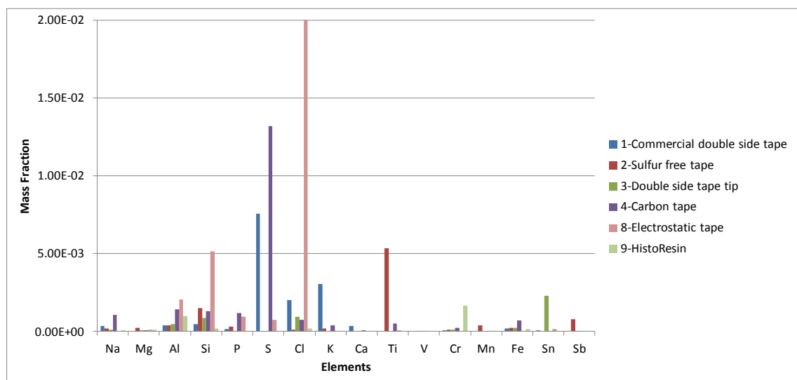
Figure 3-14: a) Comparative fit results of XRF spectra corresponding to substrates analysed, and their elemental mass fraction in b) films, c) tapes and embedding resin.
