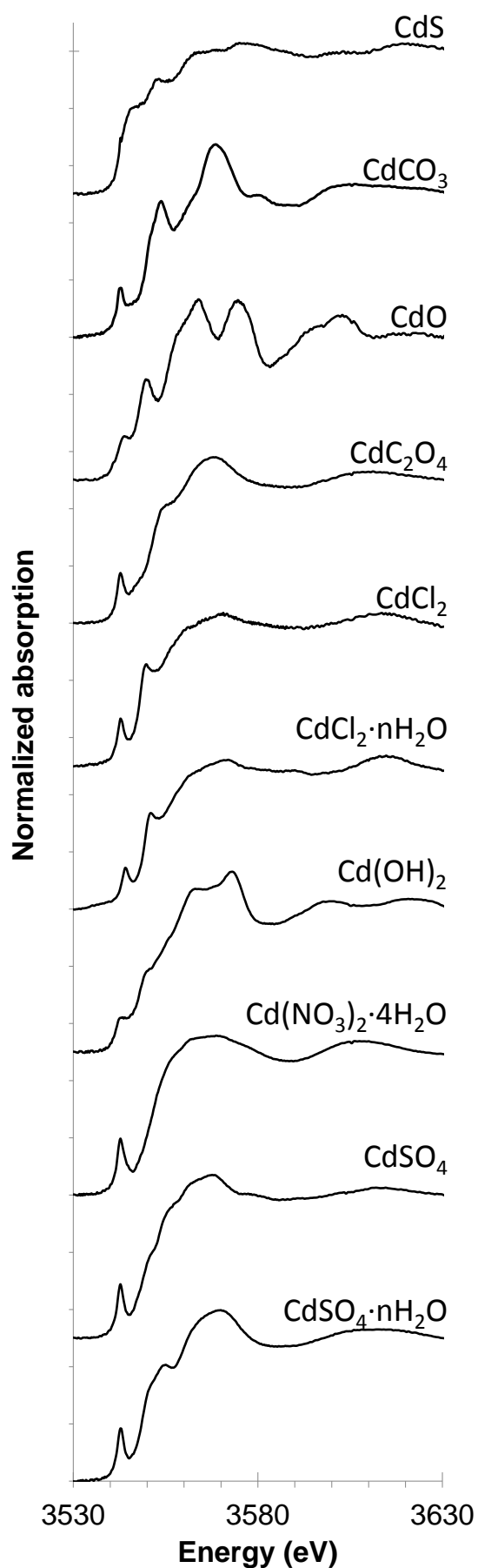
Figure 5-10: Cd L_{III} -edge XANES spectra acquired in transmission mode using FF-XANES technique on various cadmium references: cadmium sulphate ( CdSO_4 , 99.99 % metals basis), hydrated cadmium sulphate ( CdSO_4 \cdot nH_2O , 99.999 % metals basis), cadmium sulphide ( CdS , 99.995 % metals basis), cadmium nitrate tetrahydrate ( Cd(NO_3)_2 \cdot 4H_2O , >99.999 % metals basis), cadmium chloride ( CdCl_2 , >99.99 % metals basis), hydrated cadmium chloride ( CdCl_2 \cdot nH_2O , >99.99 % metals basis), cadmium oxide ( CdO , >99.99 % metals basis), cadmium carbonate ( CdCO_3 , >99.999 % metals basis) (all purchased from Sigma Aldrich) and cadmium oxalates (synthesized at Washington and Lee University).
