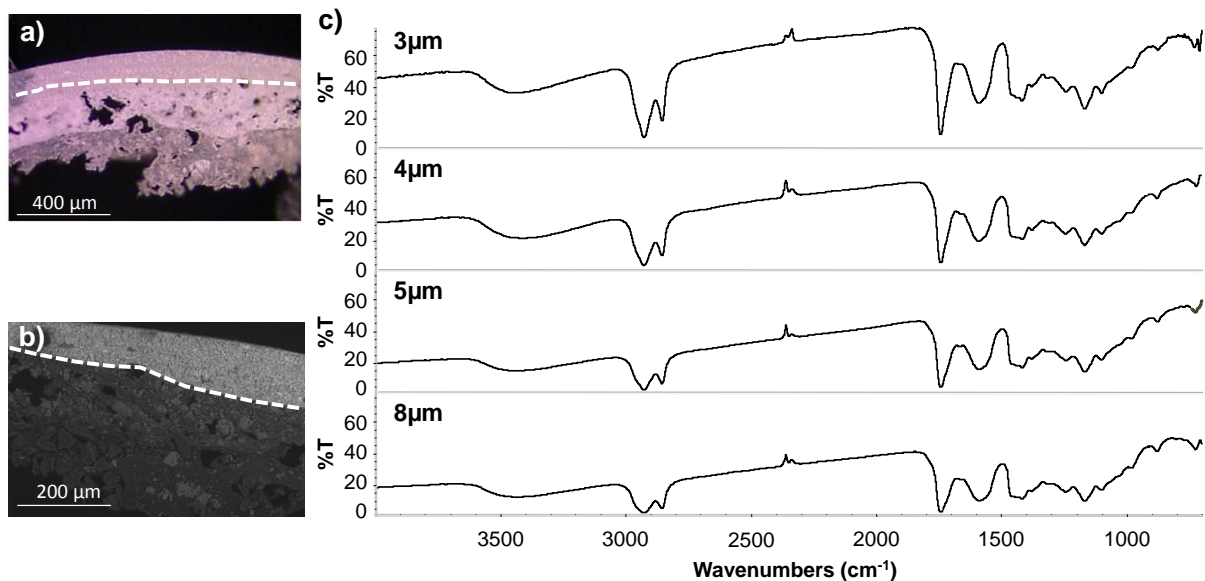
Figure 2-3: Example of \mu\text{FTIR} transmission spectra of thin-sections of a lead white model painting obtained following the SES method developed in section 3.5.2. a) Visible light microscope and b) SEM images of the 3 \mu\text{m} -thick section, c) FTIR spectra on 3 to 8 \mu\text{m} -thick sections with a 8 \times 8 \mu\text{m}^2 beam size.
