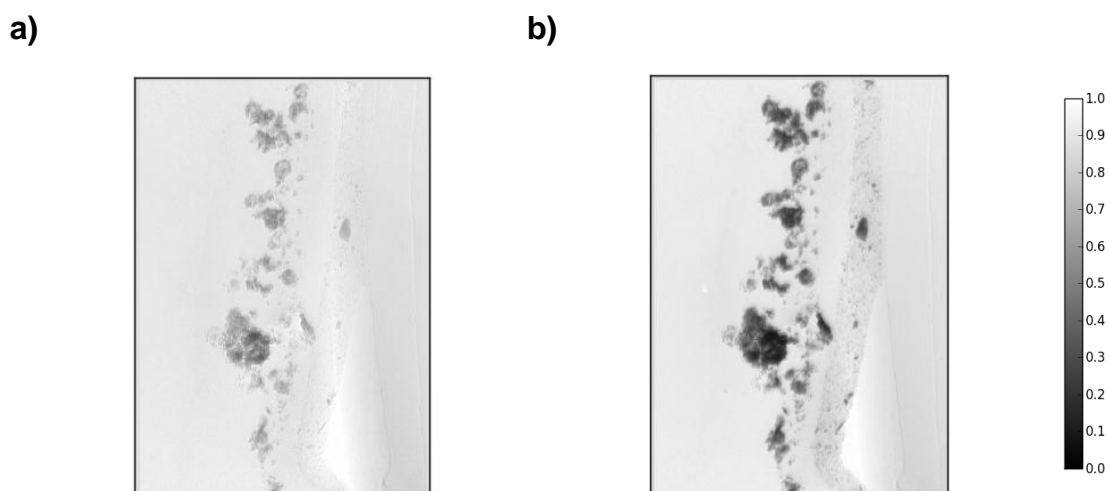
Figure 4-3: Sample transmittance images acquired on a 30 \mu m section of a bilayer model painting ( MnO_2/MnSO_4 ) a) in the pre-edge region at 6.53keV and b) in the post-edge region at 6.63keV of the Mn K-edge. Cf. visible picture and sketch in Figure 4-4a.
