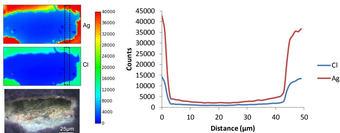
Figure 5-4: XRF maps(left) and profiles, as sum over 10 vertical lines represented as a dotted rectangle (right), of Ag and Cl acquired on the ARE thin-section at 7.2keV. Map size: 50×100 μm 2 , pixel size: 1×1 μm 2 .
