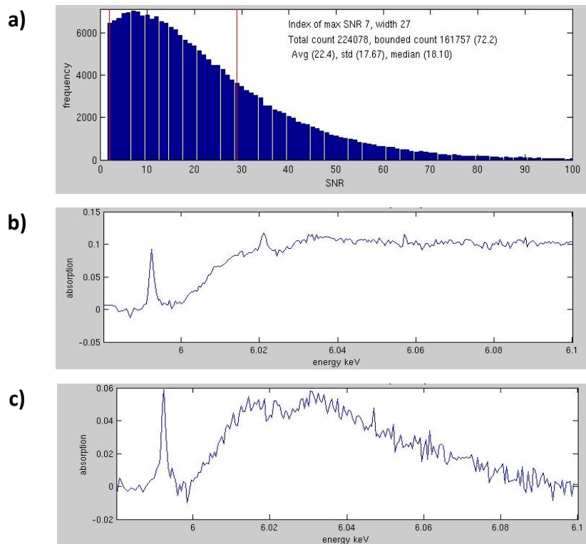
Figure 4-8: SNR automated calculation applied to full pixels of the acquisition, with complementary histogram of distribution of the SNR values a) and relative XANES with highest (224) b) and smallest (1) c) SNR values.
