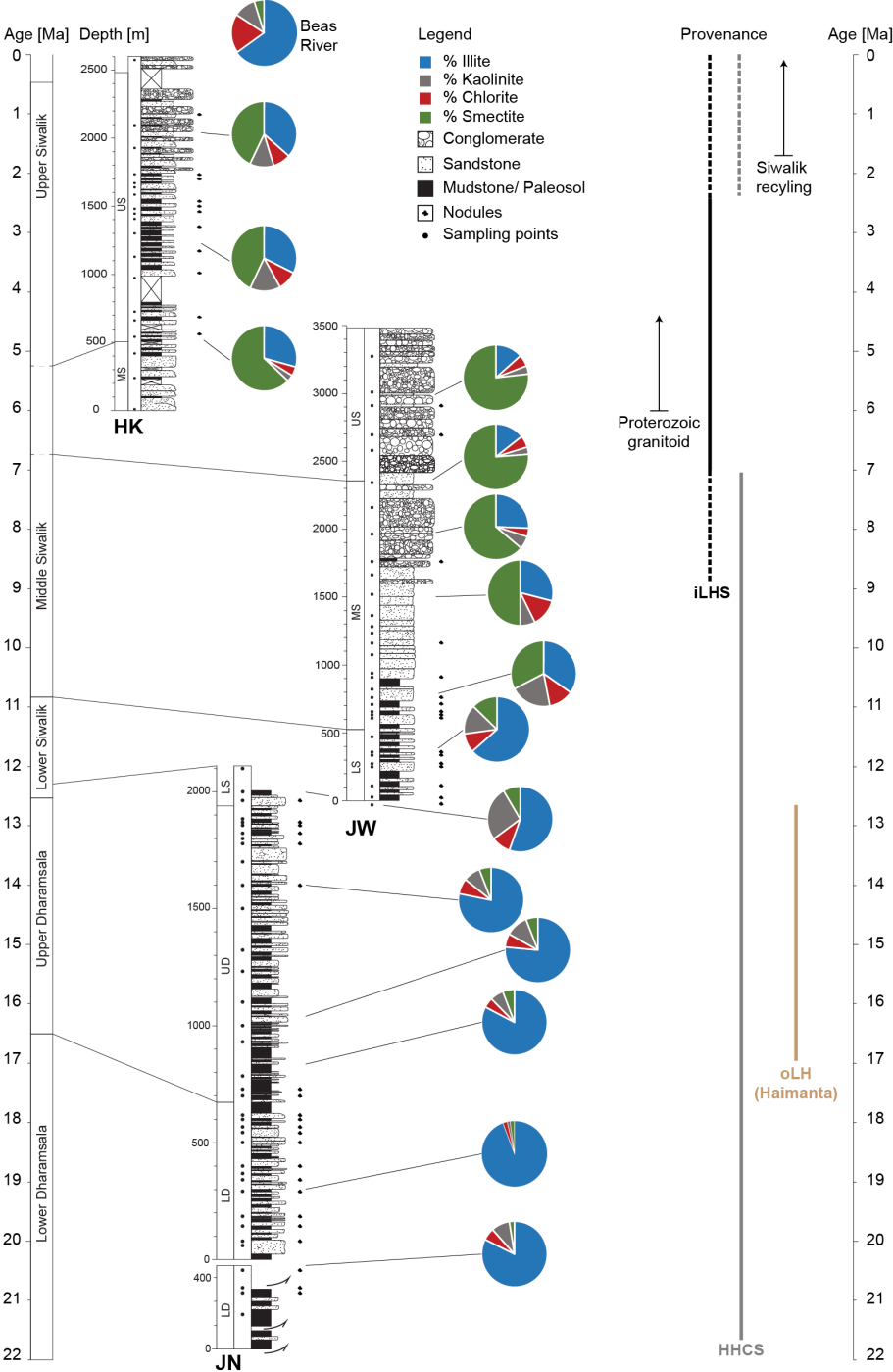
Figure 4.2: Stratigraphy, sampling points, clay mineral assemblages and inferred provenance of the Joginder Nagar, Jawalamukhi and Haripur Kolar sections. Stratigraphy and age-dating after Meigs et al. (1995); Sangode et al. (1996); White et al. (2001). Provenance from White et al. (2001, 2002), Najman et al. (2009) and Suresh et al. (2004).
