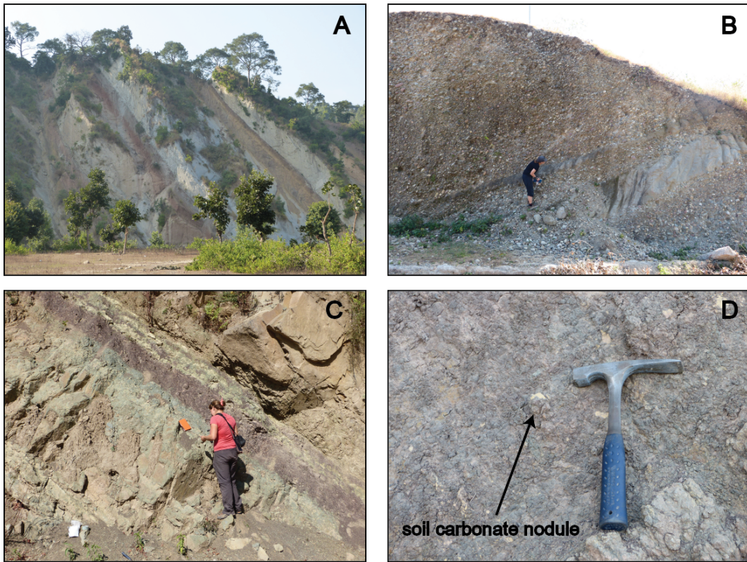
Figure 1.6: Paleosols of the Haripur Kolar section near HK14-2; B: Upper Siwalik conglomerates of the Jawalamukhi section near JW14-7; C: Paleosol of the Joginder Nagar section near JN14-28; D: Soil carbonate nodule in a paleosol of the Joginder Nagar section near JN14-10.
