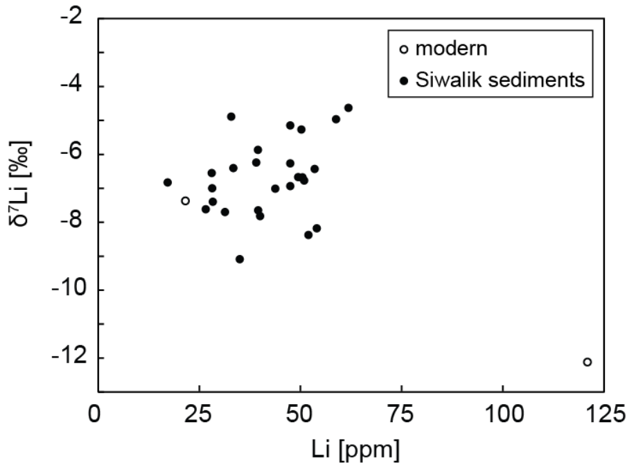
Figure 5.3: Relationship between \delta^7\text{Li} [‰] and Li concentration [ppm].
