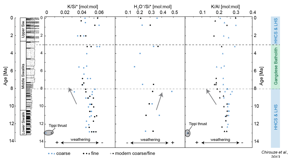
Figure 3.9: Evolution of K/Si*, H 2 O + /Si* and K/Al over time in the Kameng River section. Arrows indicate a change in weathering regime. H 2 O + /Si* is anti-correlated to K/Si* and K/Al. Modern River values are indicated in grey/black diamonds. Outliers are encircled and show sediments influenced by the formation of the Tippi thrust. Provenance change from Sm and Nd isotopes are indicated in blue and green (Chirouze et al., 2013)
