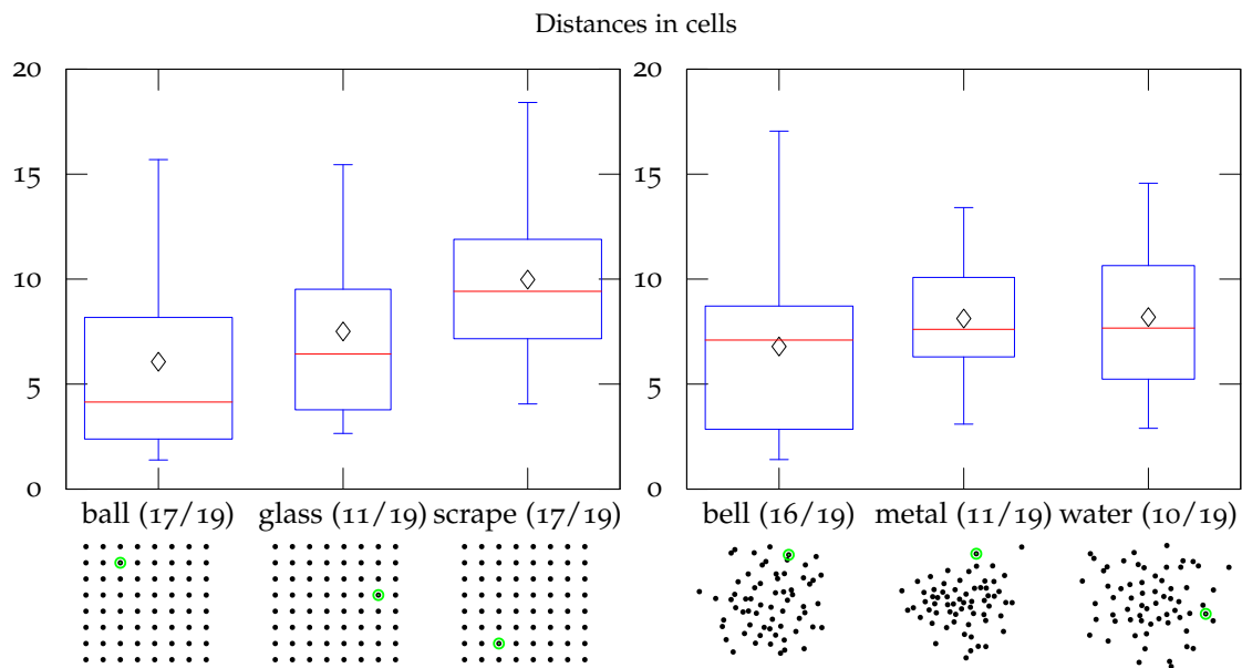
Figure 5.27: Distances per grid then cloud tasks for test 1
