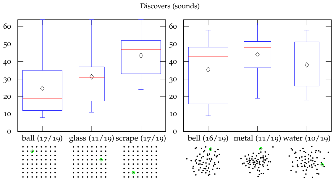
Figure 5.25: Discovers per grid then cloud tasks for test 1
