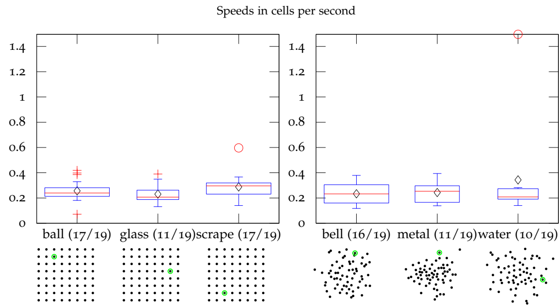
Figure 5.28: Speeds per grid then cloud tasks for test 1
