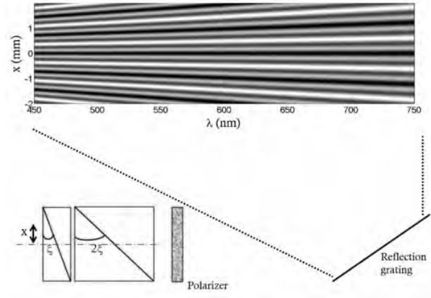
Fig. 2. Global principle of the measurement. The light travels through two double-wedge birefringent components, a linear polarizer, and finally a grating to create the spectrum. A 2D image is obtained with the spectral information in the horizontal direction and the polarization modulation in the vertical one.
