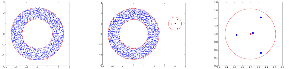
Figure 1.4: Spectrums of \mathbf{A} (left), of \mathbf{A} + \mathbf{P} (center) and zoom on a part of the spectrum of \mathbf{A} + \mathbf{P} (right), for the same matrix \mathbf{A} (chosen as in (1.1) for s_i 's uniformly distributed on [0.5, 4] with N = 10^3 ) and \mathbf{P} with rank 4 having one block \mathbf{R}_3(\theta) and one block \mathbf{R}_1(\theta) in its Jordan Canonical Form ( \theta = 4 + i ). We see, on the right, four outliers around \theta ( \theta is the red cross): three of them are at distance \approx N^{-1/6} and one of them, much closer, is at distance \approx N^{-1/2} . One can notice that the three ones draw an approximately equilateral triangle. This phenomenon will be explained by Theorem 1.2.10.
