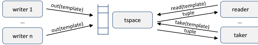
Figure 3.9: TS semantics.
