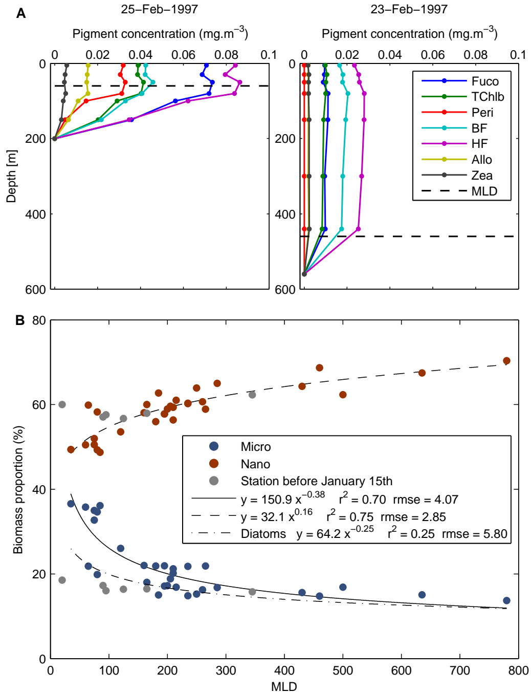
Figure 28. Chemotaxonomic analysis from the CATCH expedition (January-February 1997), see location of the stations on Fig. 22A. (A) Examples of one stratified profile (left) and one deeply mixed profile (right) of pigment concentrations. The horizontal dashed black line marks the MLD. (B) Biomass proportion of nano- and microphytoplankton as function of MLD. Solid and dashed lines represent the best-fit power law function of the data excluding grey dots, which correspond to stations before January 15th (assumed to be extremely light limited). Dash-dot line represent the best-fit power law function of the proportion of diatoms (Fuco / DP).
