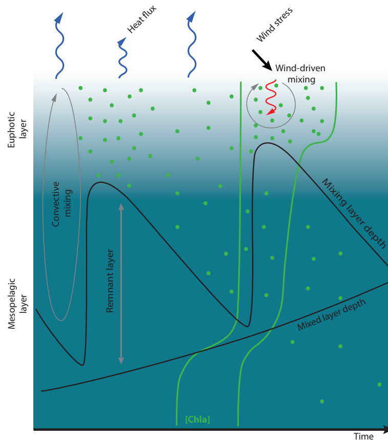
Figure. 29. Schematic of the mixed layer pump.
