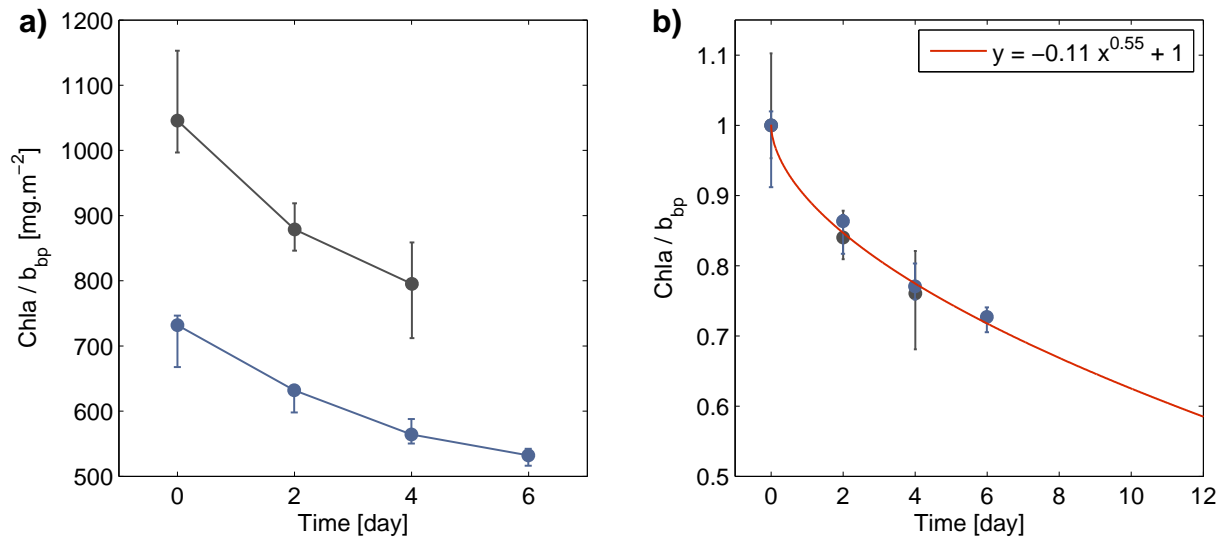
Figure. 35. a) Chla to b_{bp} ratio in the remnant layer as a function of time for sections of float trajectories 22b (black line) and 24c (blue line) shown in Fig. 30 and 34. b) Same curve as in a) but data normalized by their maximum value. The red line represents the best-fit power law function for both float sections. The vertical error bars indicate the range of data points within the remnant layer.
