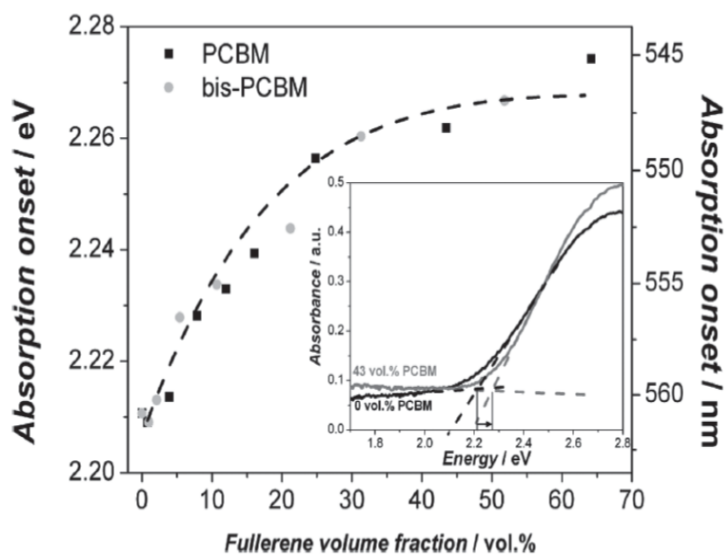
Figure 1.6 Absorption edge position of phenyl- C_{61} -butyric acid methyl ester (PCBM) and bis-PCBM. The absorption spectra of poly(3-hexylthiophene) (P3HT) and P3HT:PCBM (43 vol%) showing the shift of the absorption edge and the way for determining its value is shown in the inset. 21
