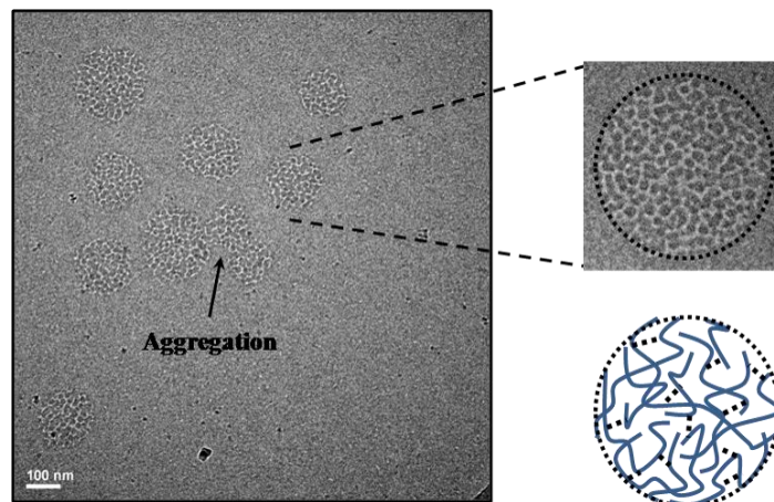
Figure 3.4 Cryo-TEM image of an aqueous sample containing 10 mM in EDOT irradiated at 70 kGy. It exhibits spherical low density objects with a mean diameter of 200 nm attributed to self-assembled hydrophilic PEDOT polymers. An aggregation process of these spherical objects is also observable. Zoom: a single spherical polymer nanoparticle with its schematic representation exhibiting hydrogen bonds interactions between the chains. 13
