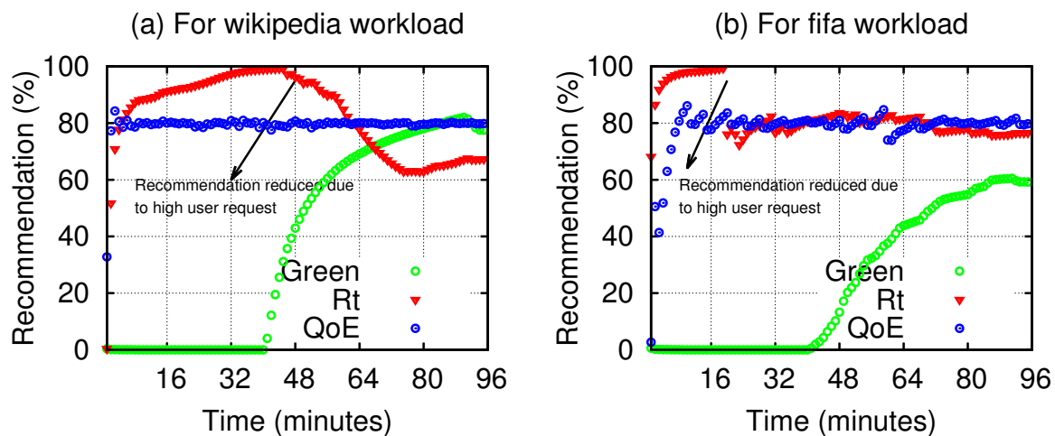
Figure 6.13: SLA validation
