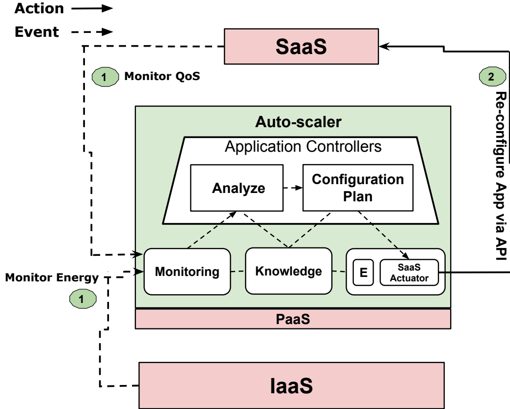
Figure 6.2: Auto-scaler architecture
