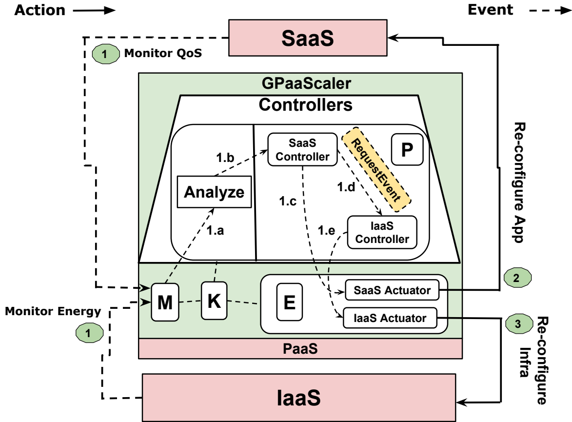
Figure 7.1: GPaaSScaler architecture
