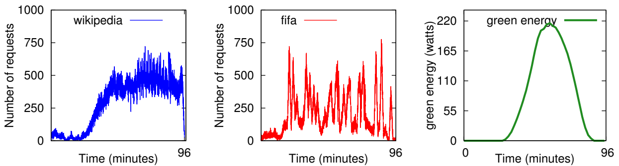
Figure 6.9: Workload trace
