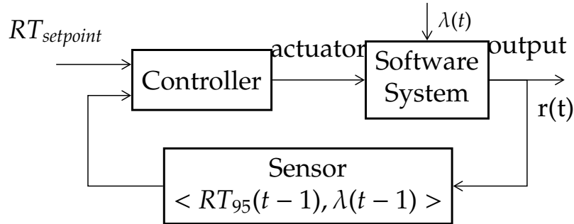
Figure 6.5: Response time aware controller
