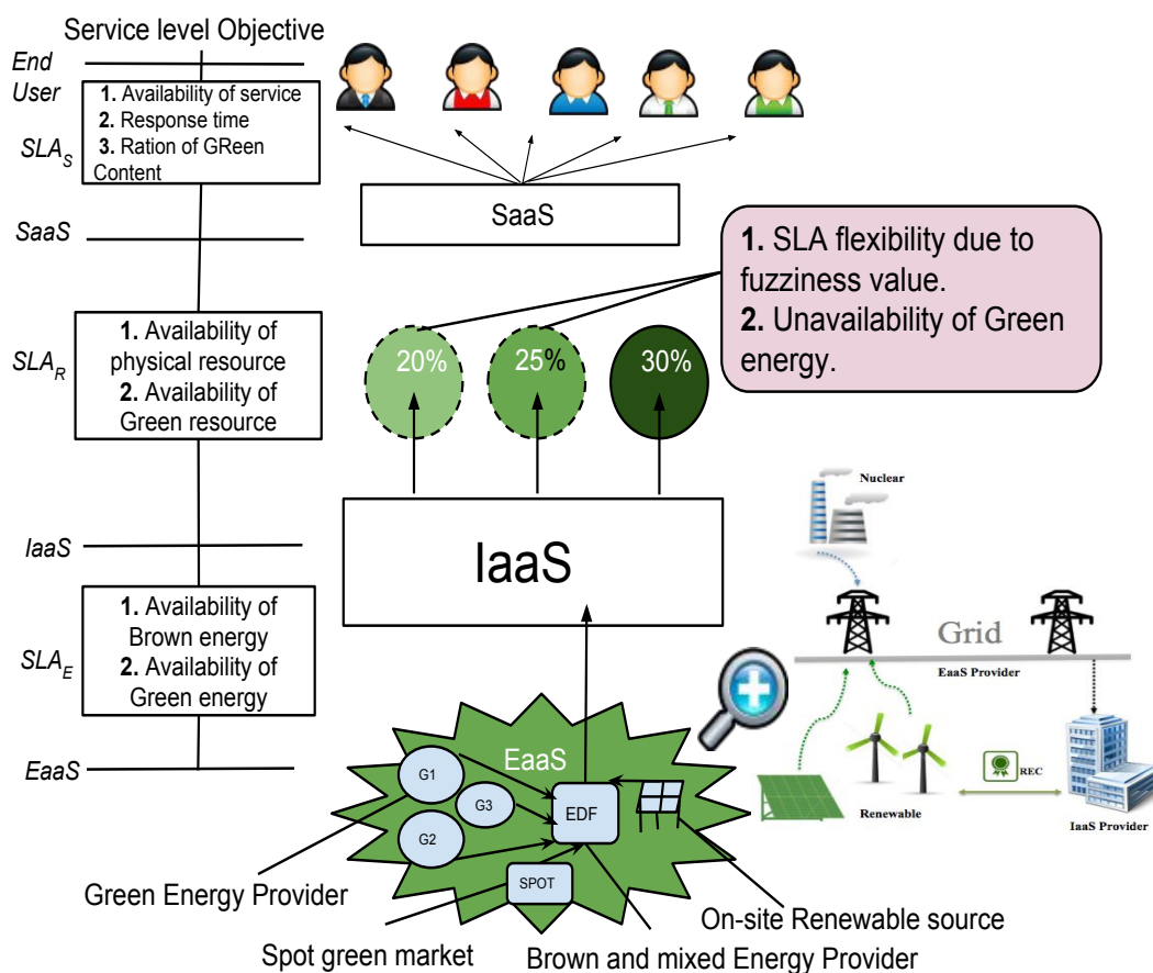
Figure 8.2: Cross-layers SLA
