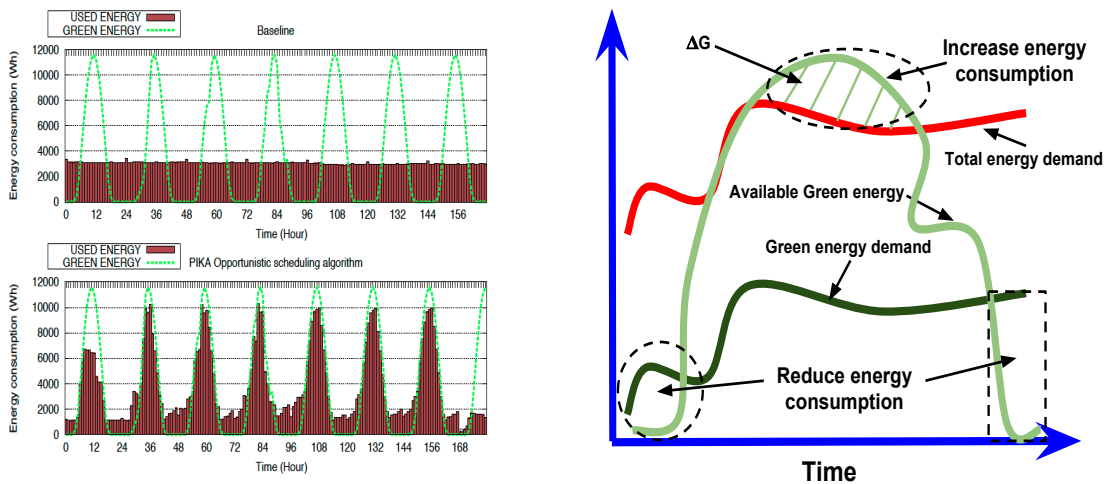
(a) Green energy adaptive batch application [LOM15] (b) Proposal for Green energy adaptive interactive SaaS application
