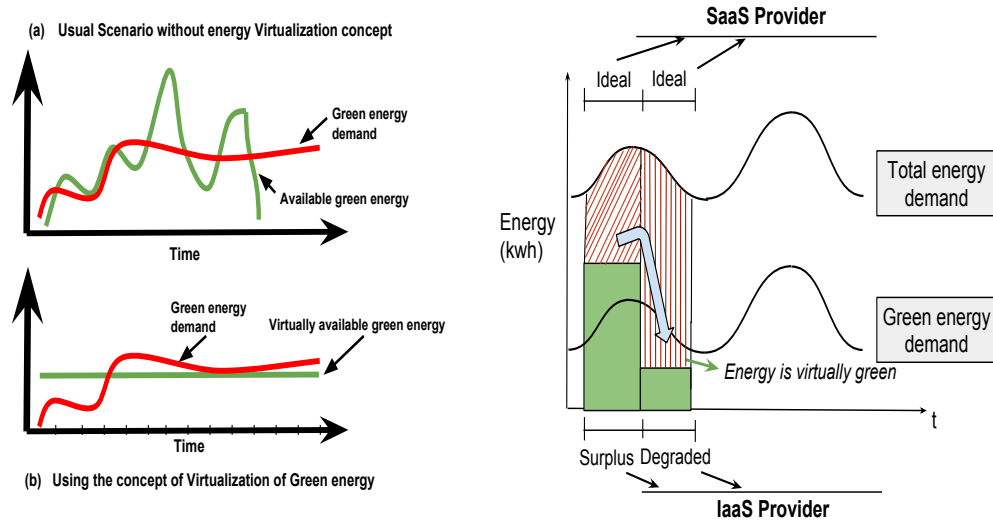
(a) Effect of green energy virtualization
