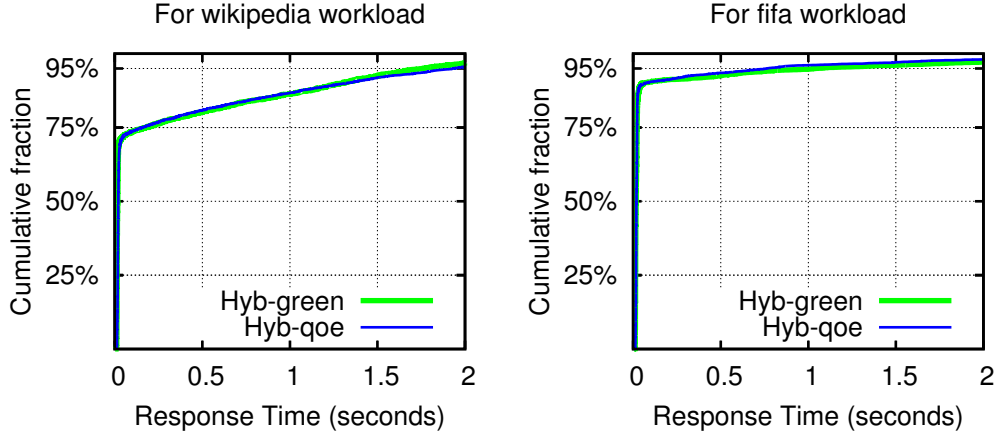
Figure 6.20: Hybrid controller's response time in percentiles
