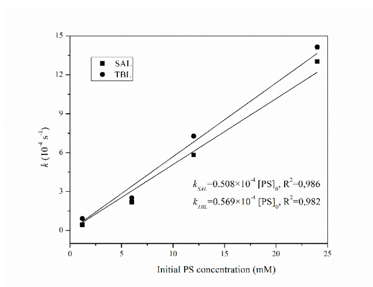
Figure 5.6. Pseudo-first order rate constants for SAL and TBL for different initial PS concentrations ( [SAL]_0 = [TBL]_0 = 120 \mu M , initial pH = 6.5).
