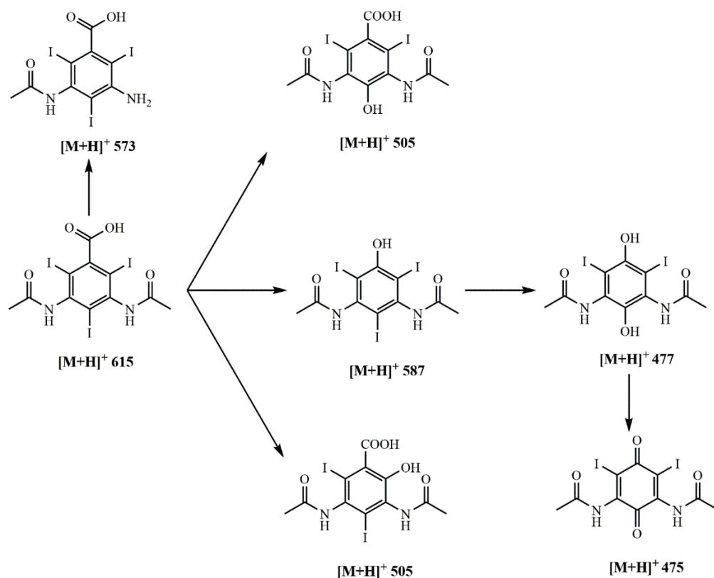
Figure 4.9. Proposed oxidation pathways of DTZ by simulated sunlight activated PS. ( [DTZ]_0 = 30 \text{ mg L}^{-1} , [PS]_0 = 12 \text{ mM} , \text{pH} = 6.5 , reaction time = 60 min).
