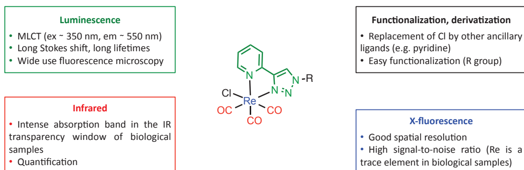
(a) Structure and properties of SCoMPI
