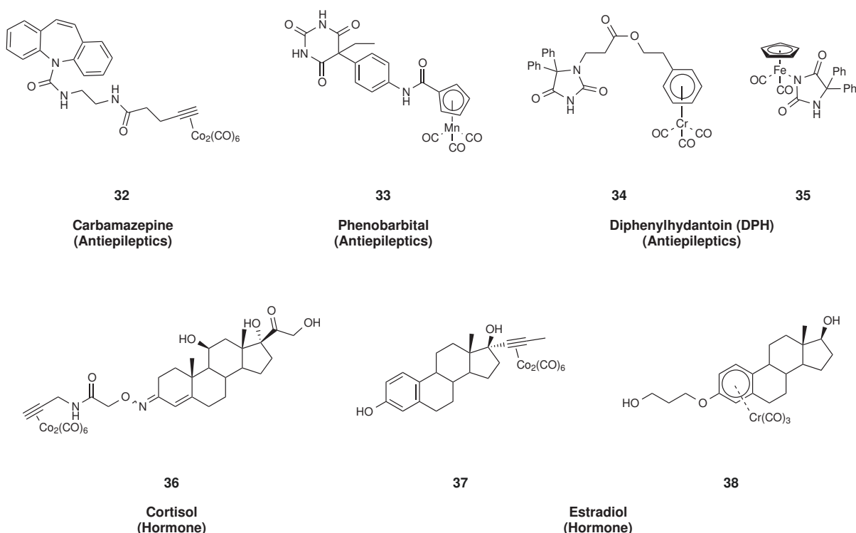
Scheme 9: Examples of molecules labelled with metal-carbonyl complexes for Carbonyl MetalloImmunoAssay (reviewed in [5])
