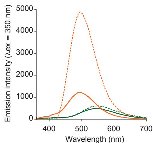
(b) Emission spectra for excitation at 350 nm (emission and excitation slits = 5 nm)
