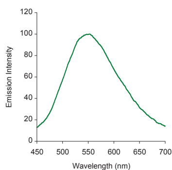
(b) Luminescence signal of SCoMPI ( \lambda_{ex} = 350 nm)
