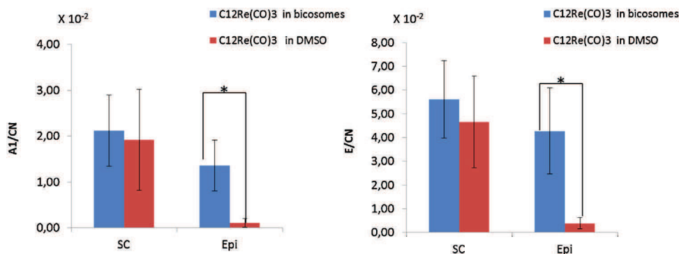
Fig. 5. Mean values and standard deviation (SD) of AUC_{C_{12}Re(CO)_3} , A_1/AUC_{Amide II} ratio (A) and AUC_{C_{12}Re(CO)_3} , E/AUC_{Amide II} ratio (B) as a function of penetration depth through the skin (SC and Epi) for C_{12}Re(CO)_3 incorporated in bicosomes or dissolved in DMSO ( N=9 ).
