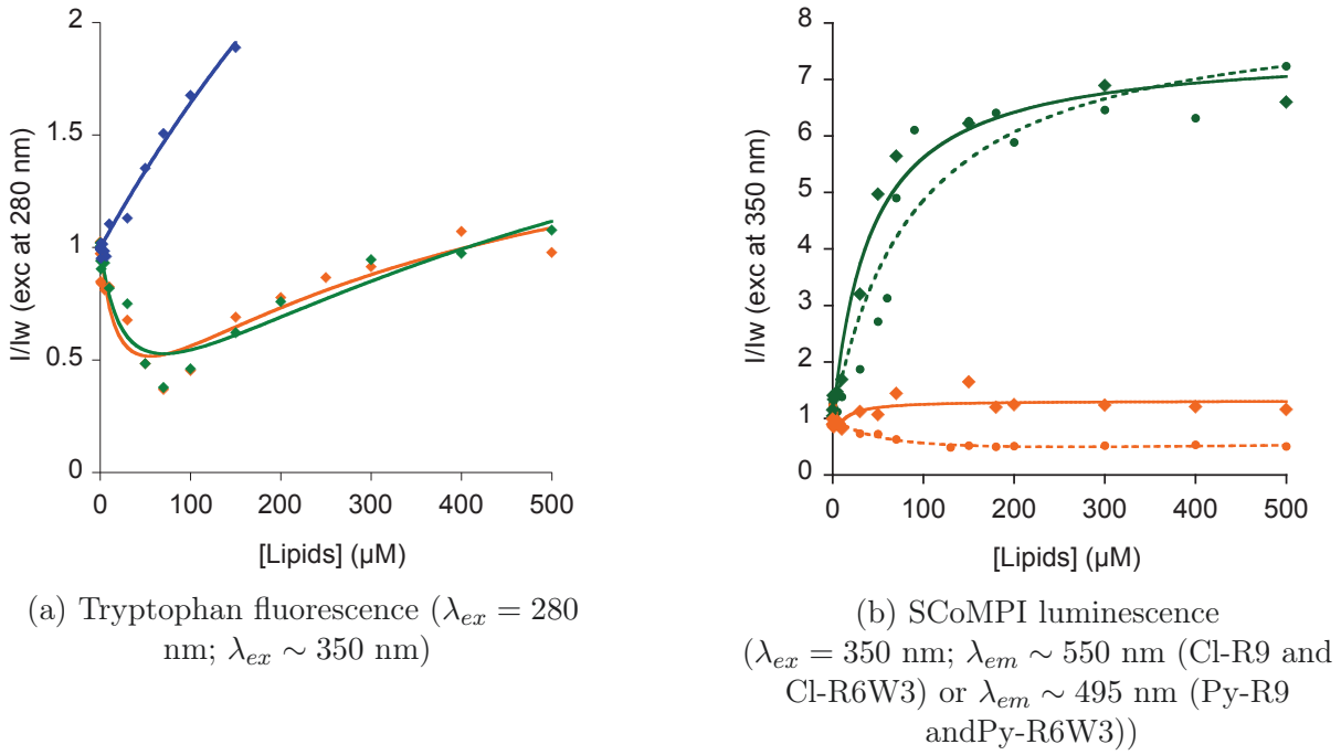
Figure 1.5: Evolution of maximum emission intensity of tryptophan and SCoMPIs with lipid concentration.
