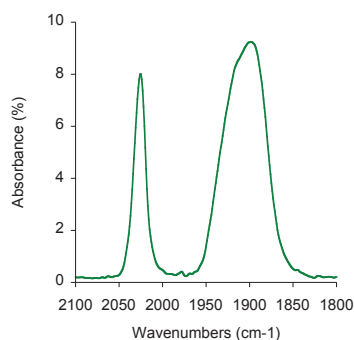
(c) Infrared signal of SCoMPI
