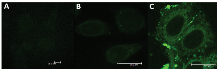
Figure 4: Enhanced cellular uptake of compound 20
