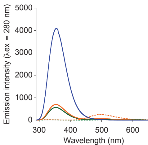
(c) Emission spectra for excitation at 280 nm (emission and excitation slits = 5 nm)
