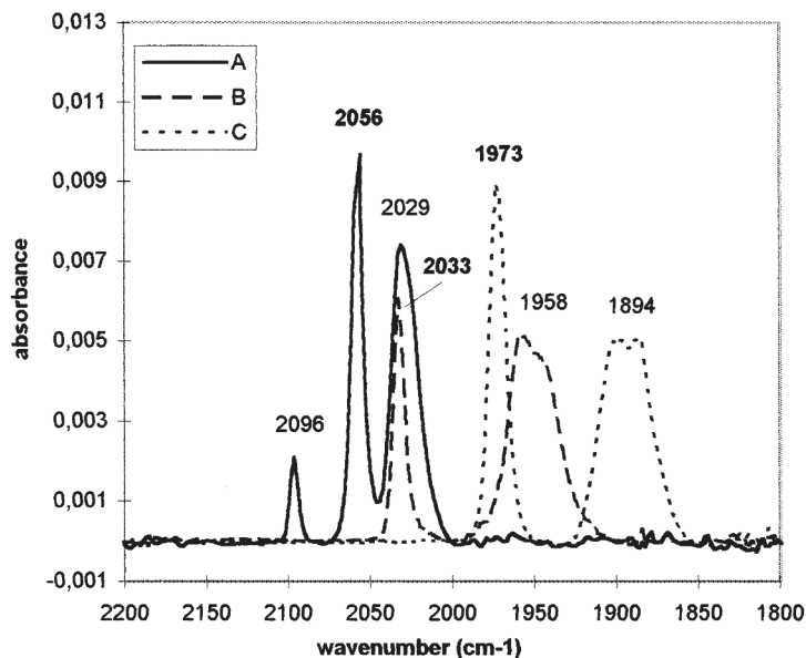
Figure 5: Principle of multi-CMIA: infrared spectra of 32 (A), 33 (B) and 34 (C). Reprinted from reference [58], Copyright (1999), with permission from Elsevier.
