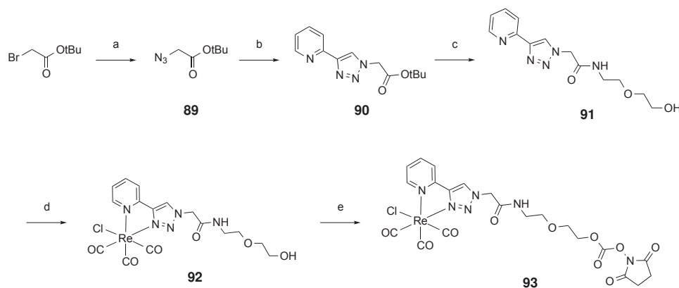
Scheme 3.2: Synthesis of LDAI-SCoMPI reagents: "NHS-activated carbonate" of SCoMPI
