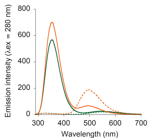
(d) Emission spectra of labelled peptides only for excitation at 280nm (see (c))
