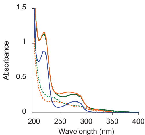
(a) Absorption spectra
