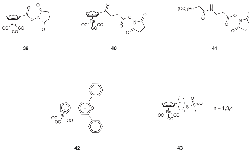
Scheme 10: [\text{Re}(\text{CO})_3(\text{Cp})] complexes for specific labelling of amines and thiols [59–61]
