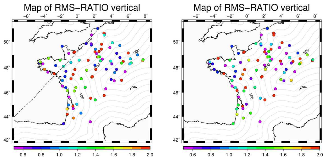
Figure 6.18 – Ratio of the RMS of the GRG and the GR2 solutions during the storm (left) and during the calm period (right). The dashed line indicates the storm ground track (the trajectory of the estimated centers of the depression). The contour lines indicate the coastal distance in km.
