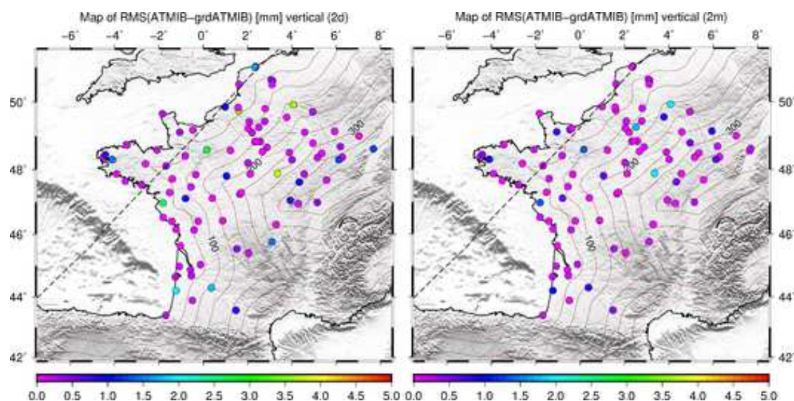
Figure 6.9 – RMS map of the differences between ATMIB and its grid interpolated version (grdATMIB) for two days (left) and for two months (right) around the storm event. The colored circles indicate the RMS values in [mm]. The brown contour lines represent the coastal distance at every 50 km. The black dashed line shows the approximated storm ground track (the trajectory of the estimated centers of the depression). Source of the ground track data: Bertin [2014].
