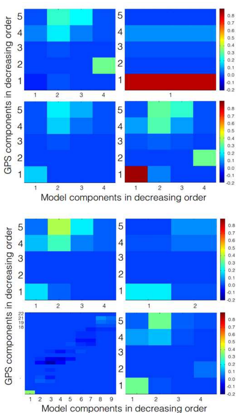
Figure 4.7 – The correlation figures for BRAZ (top) and ALIC (bottom) stations up component for ATML (top left), CWSL (top right), NTOL (bottom left) and the sum of the models (bottom right). The decreasing order means decreasing amplitude of the signal that corresponds to different periods. The colors represent the correlation coefficients between the GPS and the considered model, component by component of the SSA decomposition.
