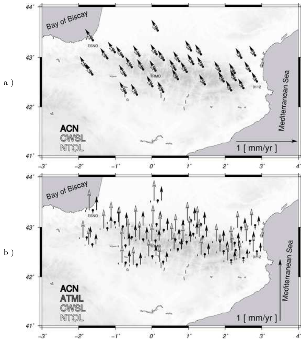
Figure 5.5 – (a) Virtual horizontal and (b) vertical loading velocity results (in mm/yr), corresponding to Table 5.4 (horizontal components), where 3-day observations are simultaneous at all stations at the beginning of July, in the year of the ResPyr campaigns, for the different effects. Accumulated (ACN in black ), atmospheric pressure (ATML, dark grey ), continental hydrology (CWSL, in grey ) and non-tidal ocean loading (NTOL, in white ). TRMO (Cirque de Troumo, France), ESNO (Mont Esnour, France) and 0112 (Montesquieu, France) are campaign station names.
