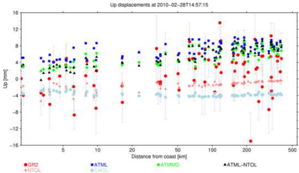
Figure 6.57 – Epoch 4: Instantaneous plot of up displacements as a function of coastal distance (logarithmic scale).
