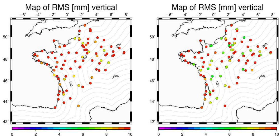
Figure 6.17 – RMS (in mm) of GRG (left) and GR2 (right) results for a two month long calm period. The contour lines indicate the coastal distance in km.
