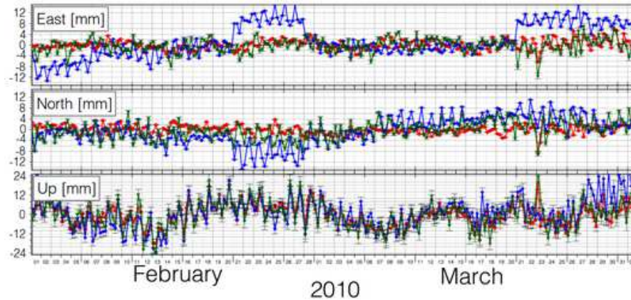
Figure 7.6 – Two months long time series, estimated with GRG (iPPP)(blue), GR2 (iPPP)(red) and IGS (PPP)(green) products at RIGA station.
