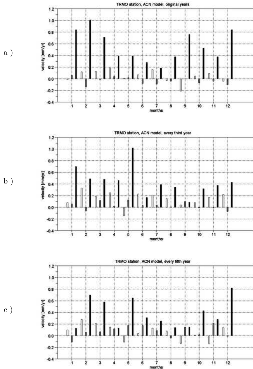
Figure 5.6 – TRMO station (campaign site Cirque de Troumo, France) simulation results in terms of velocity (mm/yr) for accumulated (ACN) loading effects. (a) For virtual campaigns at the same years than ResPyr campaigns, (b) for campaigns performed every 3 years, and (c) every 5 years. The columns correspond to the directions: North ( white ), East ( grey ) and Up ( black ) velocities. The horizontal axis numbers from 1 to 12 represent the months, January to December respectively.
