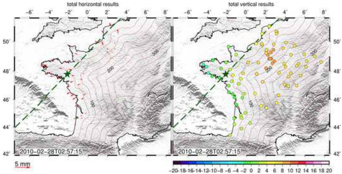
Figure 6.42 – Epoch 2: Horizontal and vertical components of the sum of ATML, CWSL and NTOL models (in mm). The green stars indicate the center of Xynthia (estimated location of depression) and the dashed line indicates the storm ground track. The contour lines represent the coastal distance at every 50 km.
