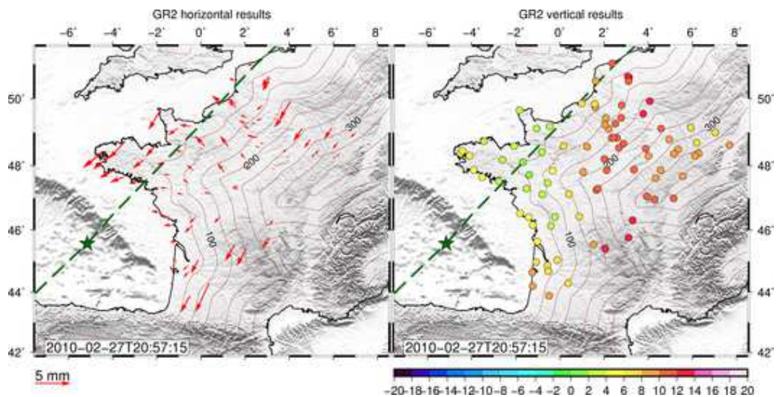
Figure 6.29 – Epoch 1: Horizontal (left) and vertical (right) GPS results (in mm) after a posteriori correction only with CWSL. The green stars indicate the center of Xynthia (estimated location of depression) and the dashed line indicates the storm ground track. The contour lines represent the coastal distance at every 50 km.
