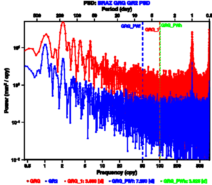
Figure 4.3 – The power spectra of GPS time series estimated using GRG and GR2 products at BRAZ station. The vertical dashed lines represent the period of the full GRGS GPS processing week [7.25 days] (blue), the half of this period [3.625 days] (green) and the signal that was observed by Ray et al. [2013] [3.66 days] (red).
