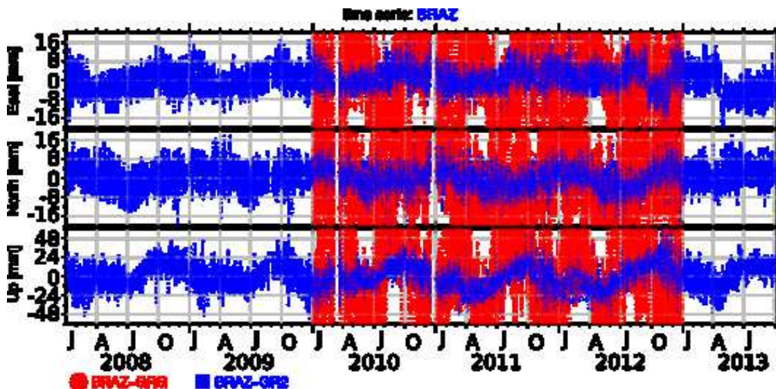
Figure 4.2 – GPS time series estimated using GRG (red) and GR2 (blue) products at BRAZ station.
