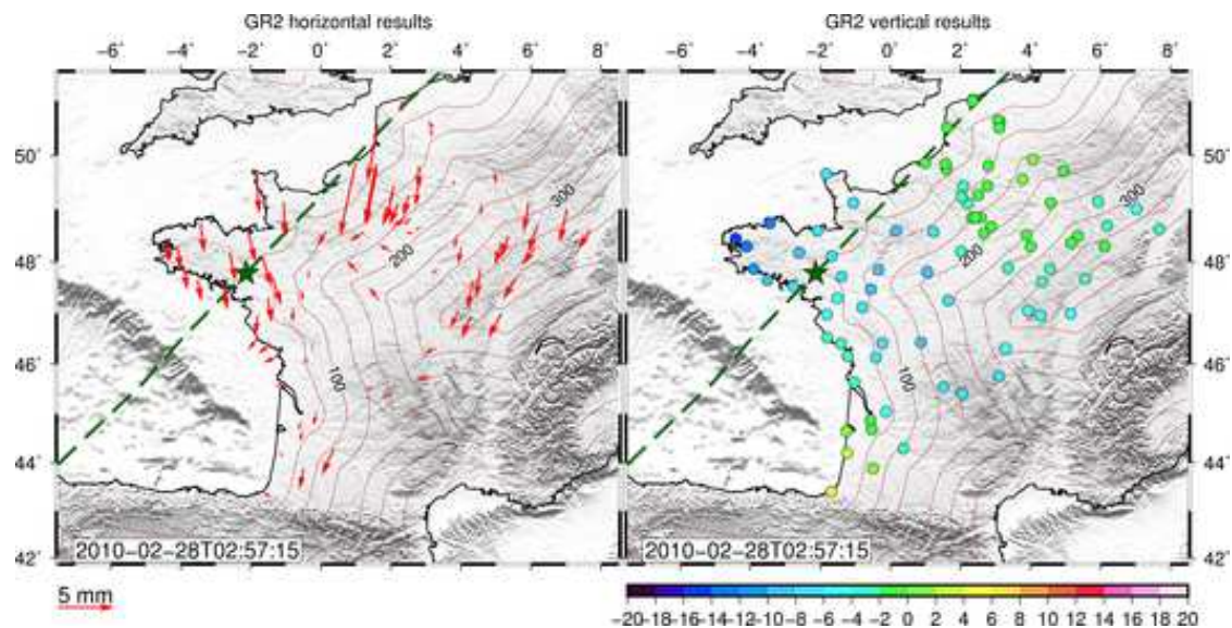
Figure 6.34 – Epoch 2: Horizontal (left) and vertical (right) GPS results (in mm) after a posteriori correction with the sum of ATML and CWSL. The green stars indicate the center of Xynthia (estimated location of depression) and the dashed line indicates the storm ground track. The contour lines represent the coastal distance at every 50 km.
