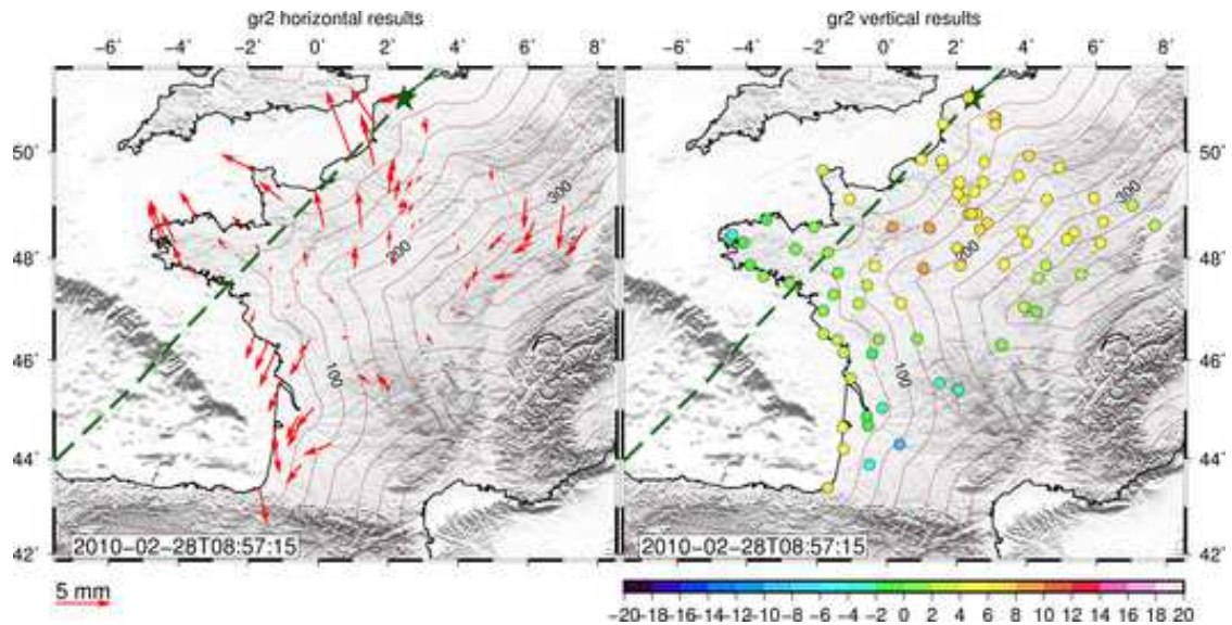
Figure 6.27 – Epoch 3: Horizontal and vertical GPS results (in mm) applying a spatial filter. The green stars indicate the center of Xynthia (estimated location of depression) and the dashed line indicates the storm ground track. The contour lines represent the coastal distance at every 50 km.
