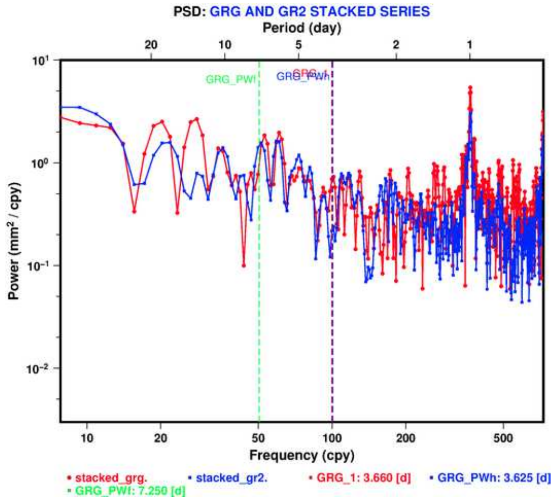
Figure 6.19 – The power spectral density of the stacked GRG (red) and GR2 (blue) time series. The vertical dashed lines represent the period of the full GRGS GPS processing week [7.25 days] (green), the half of this period [3.625 days] (blue) and the signal that was observed by Ray et al. [2013] [3.66 days] (red).
