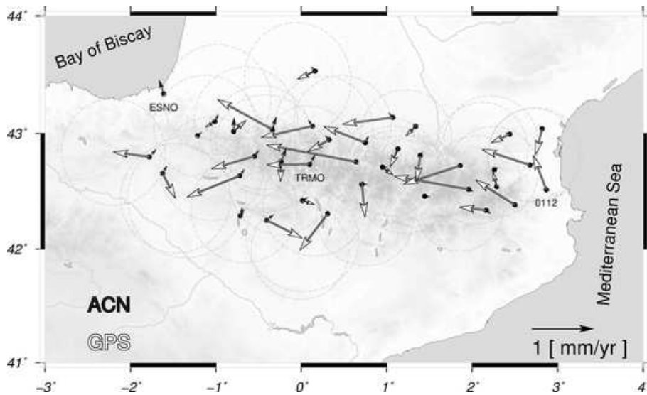
Figure 5.4 – Accumulated loading effect (ACN) and GPS horizontal velocities (in mm/yr). TRMO (Cirque de Troumo, France), ESNO (Mont Esnour, France) and 0112 (Montesquieu, France) are campaign station names.
