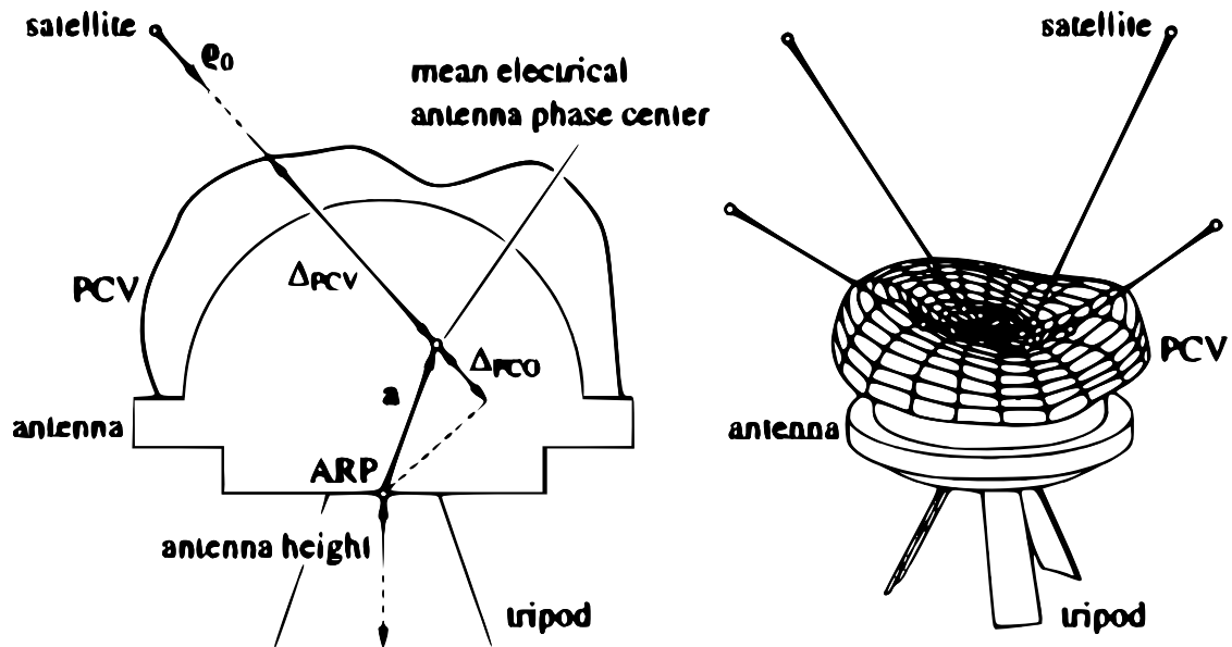
Figure 3.2 – Illustration of antenna reference point (ARP), phase center offset (PCO) and phase center variation (PCV) [Hofmann-Wellenhof et al. 2007].
