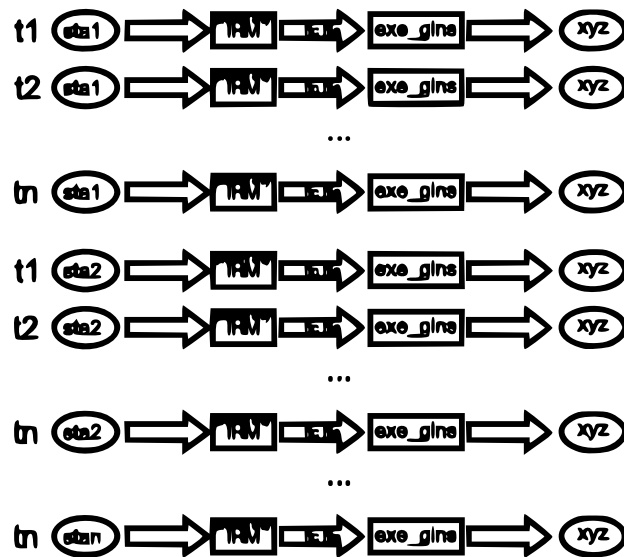
Figure 7.18 – Processing scheme that we apply at the moment.
