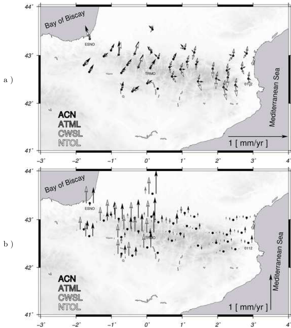
Figure 5.3 – (a) Horizontal and (b) vertical velocities (in mm/yr) for different loading effects. Accumulated (ACN, in black ), atmospheric pressure (ATML, in dark grey ), non-tidal ocean loading (NTOL, in white ), and continental hydrology (CWSL, in light grey ). TRMO (Cirque de Troumo, France), ESNO (Mont Esnour, France) and 0112 (Montesquieu, France) are campaign station names.
