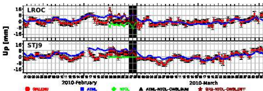
Figure 6.8 – GPS and model time series for two stations: LROC (top) and STJ9 (bottom), during two months centered on Xynthia. The storm Xynthia is indicated with the grey rectangle. The different colors are: GPS (red), ATML (blue), NTOL (green), sum of the models (black) and GPS a posteriori corrected with the sum of NTOL and CWSL (claret).
