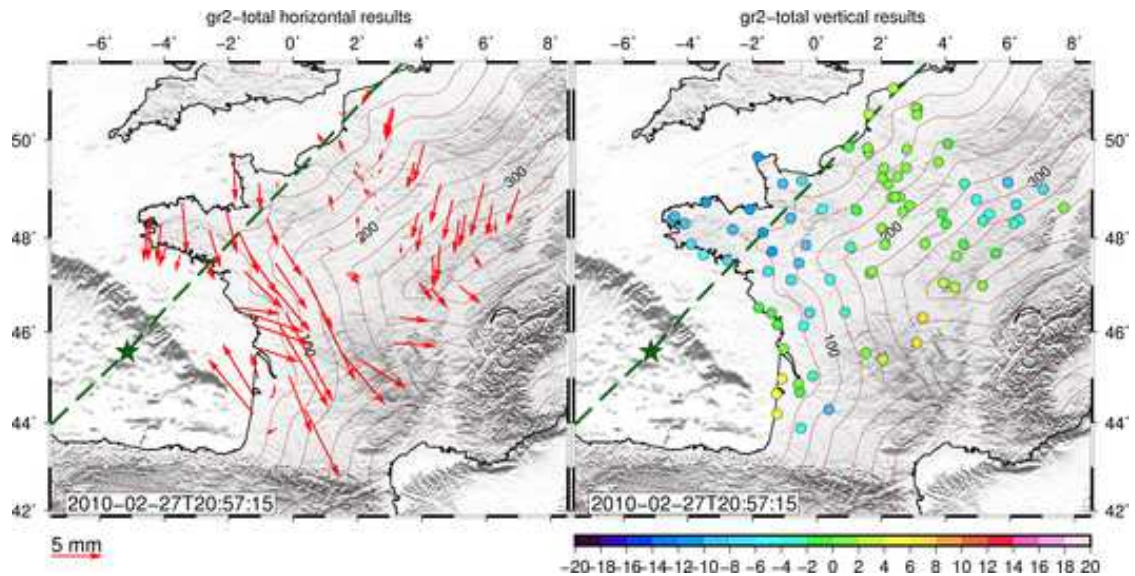
Figure 6.45 – Epoch 1: Horizontal (left) and vertical (right) GPS results (in mm) after a posteriori correction with the sum of ATML, CWSL and NTOL. The green stars indicate the center of Xynthia (estimated location of depression) and the dashed line indicates the storm ground track. The contour lines represent the coastal distance at every 50 km.
