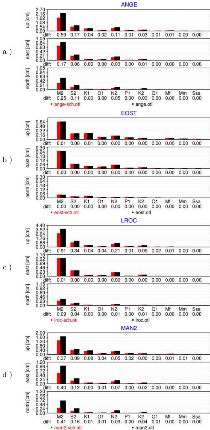
Figure 7.14 – Comparison of 11 tidal waves ( M2 , S2 , K1 , O1 , N2 , P1 , K2 , Q1 , Mf , Mm and Ssa ) from nominal FES2004 (black) and Scherneck FES2004 files (red) at a) ANGE [ \approx 108 km], b) EOST [ \approx 396 km], c) LROC [ \approx 4 km] and d) MAN2 [ \approx 129 km].
