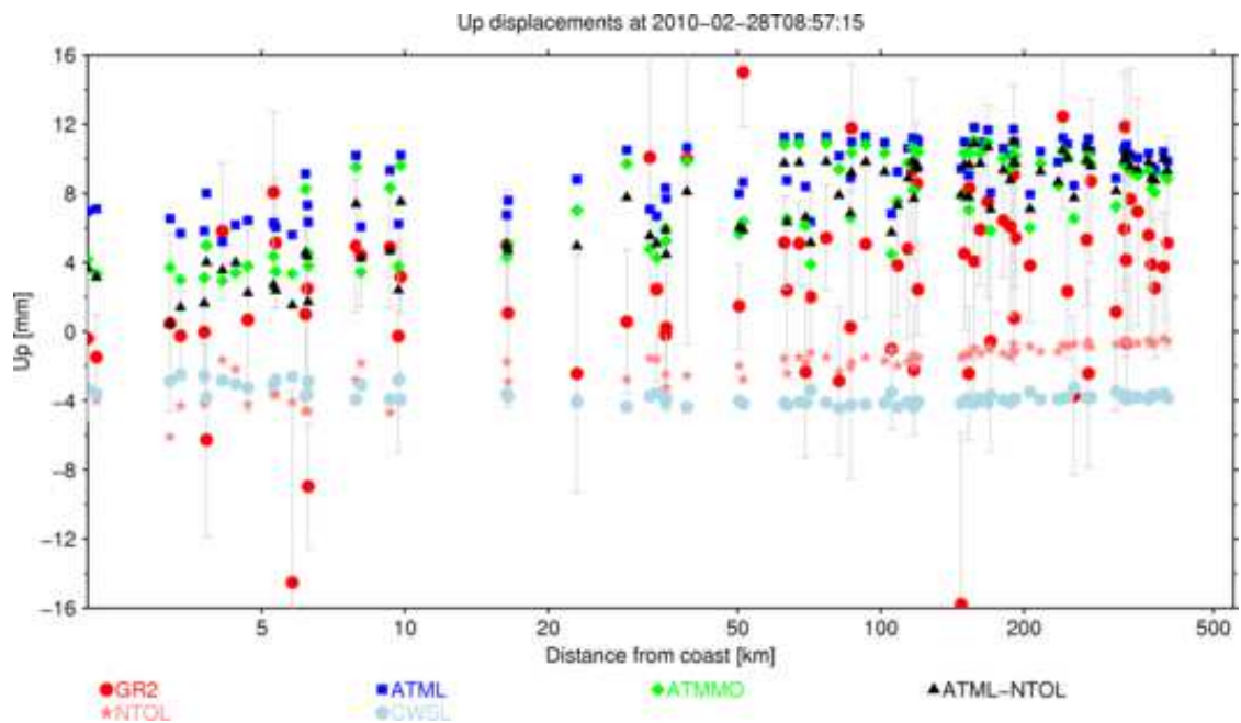
Figure 6.56 – Epoch 3: Instantaneous plot of up displacements as a function of coastal distance (logarithmic scale).
