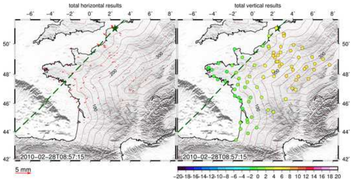
Figure 6.43 – Epoch 3: Horizontal and vertical components of the sum of ATML, CWSL and NTOL models (in mm). The green stars indicate the center of Xynthia (estimated location of depression) and the dashed line indicates the storm ground track. The contour lines represent the coastal distance at every 50 km.
