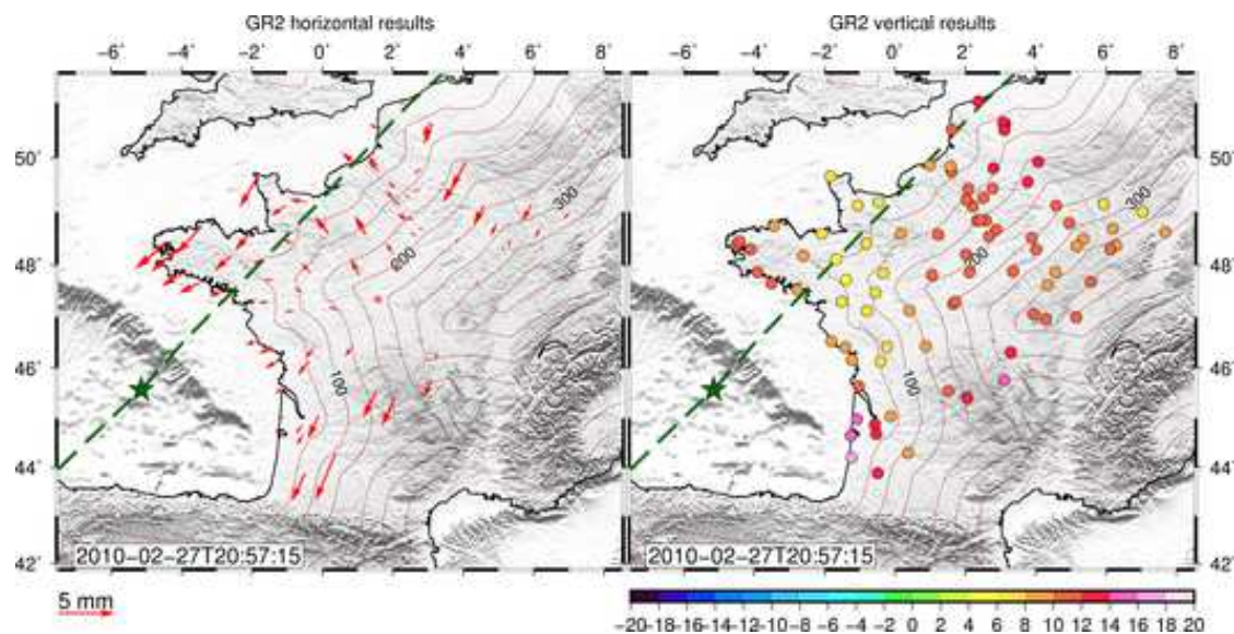
Figure 6.37 – Epoch 1: Horizontal (left) and vertical (right) GPS results (in mm) after a posteriori correction with the sum of NTOL and CWSL. The green stars indicate the center of Xynthia (estimated location of depression) and the dashed line indicates the storm ground track. The contour lines represent the coastal distance at every 50 km.
