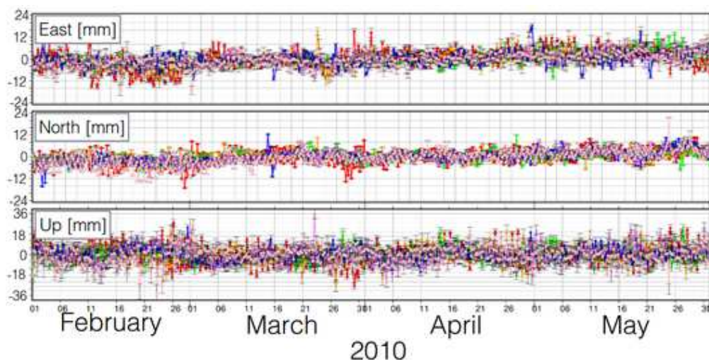
Figure 7.2 – Superposition of four months long PPP time series, estimated with IGS products at different European stations: BRST (red), LROC (yellow), PENC (green), POTS (blue), RIGA (purple) and TLSE (pink) (same as in Figure 7.1).
