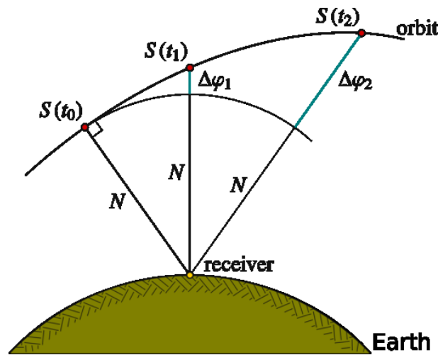
Figure 3.4 – Phase range measurement and the corresponding ambiguity ( N ) over the satellite pass [Hofmann-Wellenhof et al. 2007].
