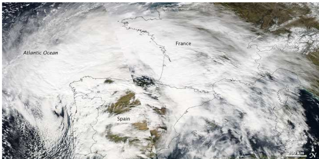
Figure 6.3 – Satellite image of Xynthia. Source: NASA.
