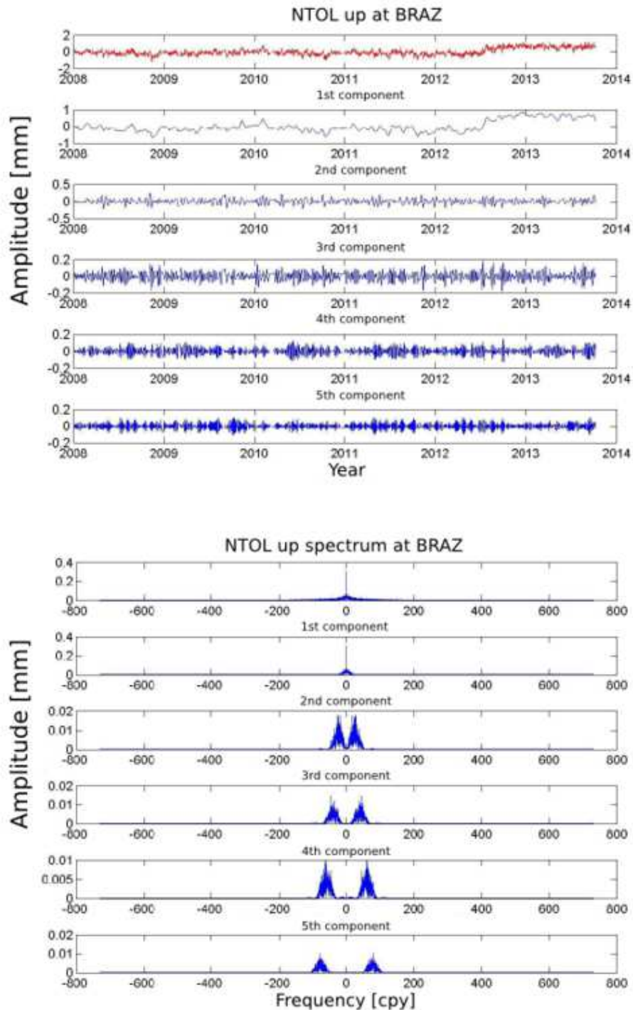
Figure A.2 – NTOL time series components (top) and their spectrum (bottom) at BRAZ station up component in decreasing order of amplitude (in mm). For example the first component corresponds to an annual period.
