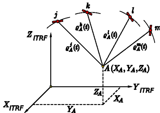
Figure 3.3 – Principle idea of GPS-PPP configuration. X_A , Y_A and Z_A are the cartesian coordinates of the GPS station. The small case latin letters j , k , l and m signify visible satellites at epoch. The greek letter \rho represents range measurements between the corresponding satellite and the geodetic site. The ITRF in the subscript shows the reference system. Source: Hofmann-Wellenhof and Moritz [2005].
