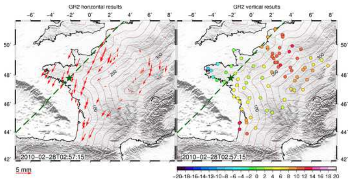
Figure 6.30 – Epoch 2: Horizontal (left) and vertical (right) GPS results (in mm) after a posteriori correction only with CWSL. The green stars indicate the center of Xynthia (estimated location of depression) and the dashed line indicates the storm ground track. The contour lines represent the coastal distance at every 50 km.
