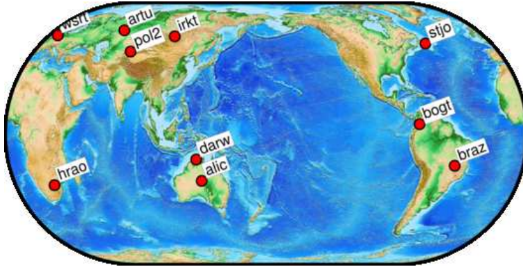
Figure 4.1 – Our network containing 10 GPS stations.
