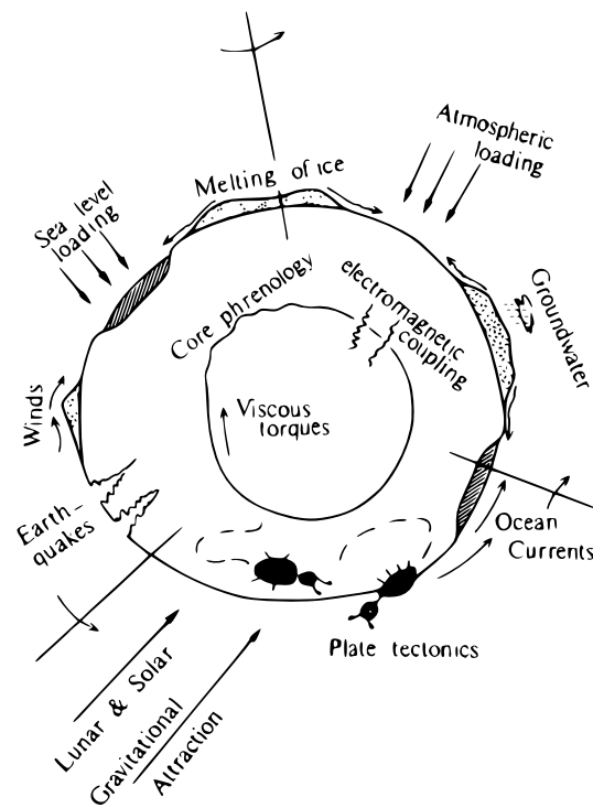
Figure 1.3 – Surface deformation processes on the Earth. Source: Lambeck [1980].
