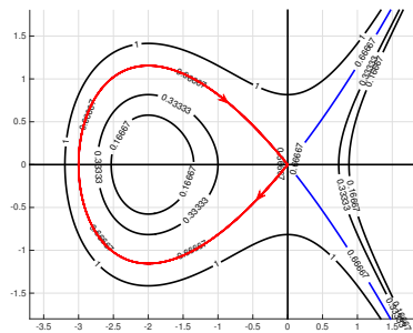
FIGURE 5.3 – Level curves of the Hamiltonian \mathcal{H} in the (KdV - - 4) case ( h \equiv \frac{1}{2} ) and for \Lambda = 1 – The blue curve corresponds to the level \frac{2}{3} and the red one to the homoclinic orbit
