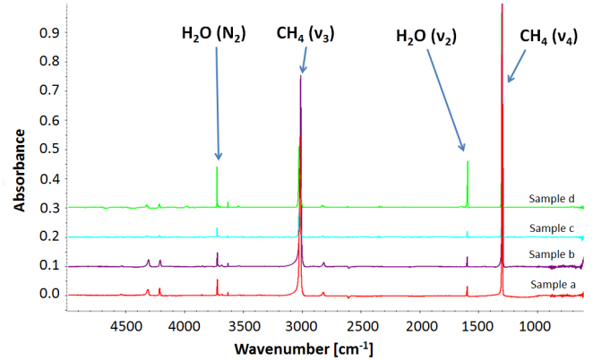
Fig. 2. Infrared spectra of samples a to d. Samples a and b were deposited using a (90:10) \text{N}_2 - \text{CH}_4 mixture, and samples c and d using a (98:2) mixture. Spectra were shifted for clarity. Small amounts of water contamination are present in the spectra. The major bands are identified, see text and Table 1 for details.
