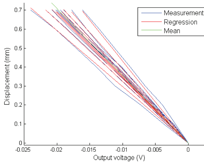
FIGURE B.15: Calibration measurement for the photointerrupter 2 for 10 reeds in the RF \tilde{Y} .
