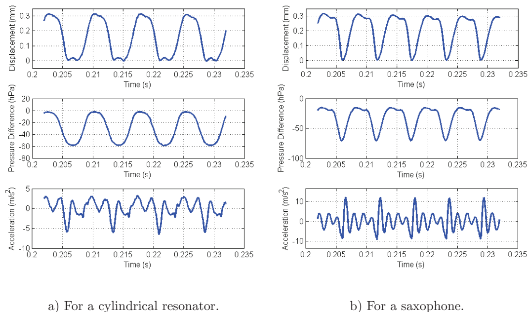
FIGURE 2.7: Measured reed displacement, pressure difference and acceleration on the mouthpiece.
