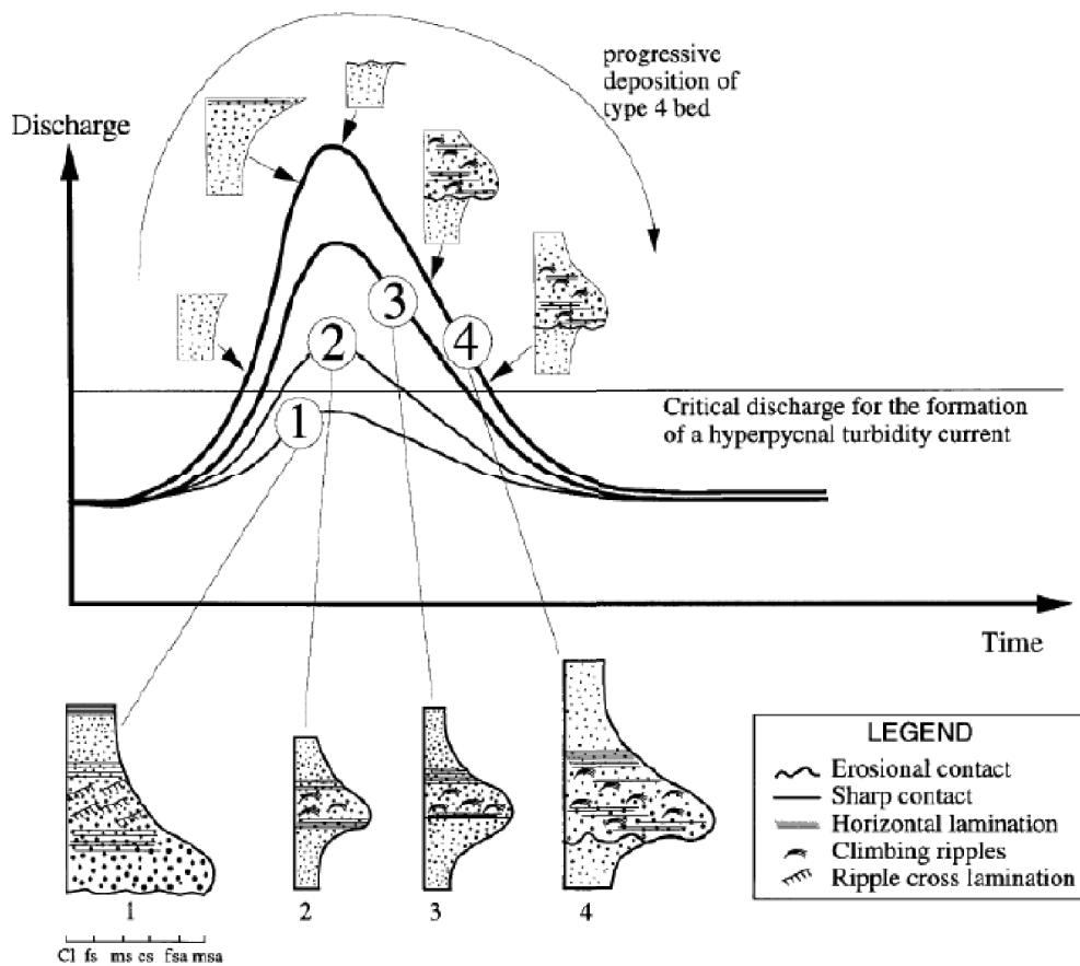
Figure 2.5: Sequence and facies of a hyperpycnal deposit according to the charge and discharge of the river during flood (after Mulder et al., 2003)
