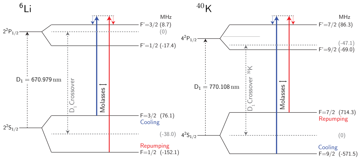
Figure 2.5: Level schemes corresponding to the D_1 line transitions of {}^6\text{Li} and {}^{40}\text{K} , as presented in [148]. Solid and dashed arrows illustrate the frequencies and detunings required for the sub-Doppler cooling, respectively. The lasers are frequency locked to the saturated absorption crossover signals 2^2S_{1/2} (|F=1/2\rangle, |F=3/2\rangle) \rightarrow 2^2P_{1/2} of {}^6\text{Li} and 4^2S_{1/2} (|F=1\rangle, |F=2\rangle) \rightarrow 4^2P_{1/2} |F'=2\rangle of {}^{39}\text{K} . The D_1 sub-Doppler cooling is presented in Chapter 3.
