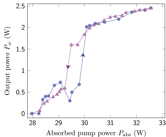
Figure 6.8: Infrared unidirectional output power P_w as a function of the absorbed pump power P_{\text{abs}} . The setup is optimized for the maximal absorbed pump power P_{\text{abs,max}} = 32.5 W. The oscillation threshold is found at P_{\text{abs}} \sim 28 W. The data shows hysteresis between P_{\text{abs}} = 29 W and 30 W, as indicated by the arrows for increasing or decreasing pump power. This behavior is typical for high-power designs. After a sudden rise the output power increases only slowly until it eventually reaches the maximum of 2.5 W at P_{\text{abs,max}} . Lines are guides to the eye only.
