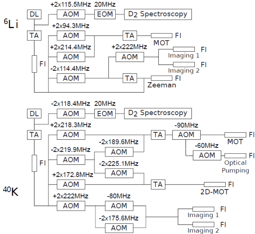
Figure 2.4: Laser systems for addressing the D 2 line transitions of 6 Li and 40 K. The frequencies and amplitudes for the different beams are controlled by AOMs in single pass (sp) or double pass (dp) configuration. The EOMs modulate the phase of the spectroscopy beam for frequency stabilization of the diode lasers. Single-mode polarization maintaining fibers (FI) clean the beams spatially. The indicated AOM frequencies correspond to the beam frequencies required for the MOT operation, see Figures 2.2 and 2.3.
