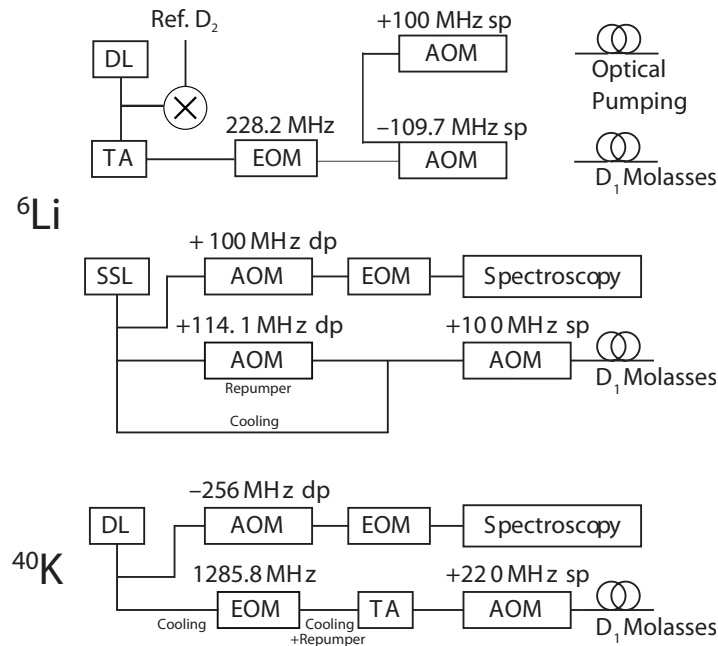
Figure 2.6: Laser systems of the D_1 molasses cooling schemes for {}^6\text{Li} and {}^{40}\text{K} . The frequencies and amplitudes of the various beams are controlled by AOMs in single pass (sp) or double pass (dp) configuration. EOMs creates the repumping frequency in the {}^{40}\text{K} setup and in the diode laser (DL) {}^6\text{Li} setup. The EOMs in the spectroscopy phase modulate a sample of the beam for the frequency-lock of the lasers. Single mode polarization maintaining fibers transmit the beams to the main experimental table. The indicated AOM frequencies correspond to the beam frequencies required for the molasses cooling, see Figure 2.5.
