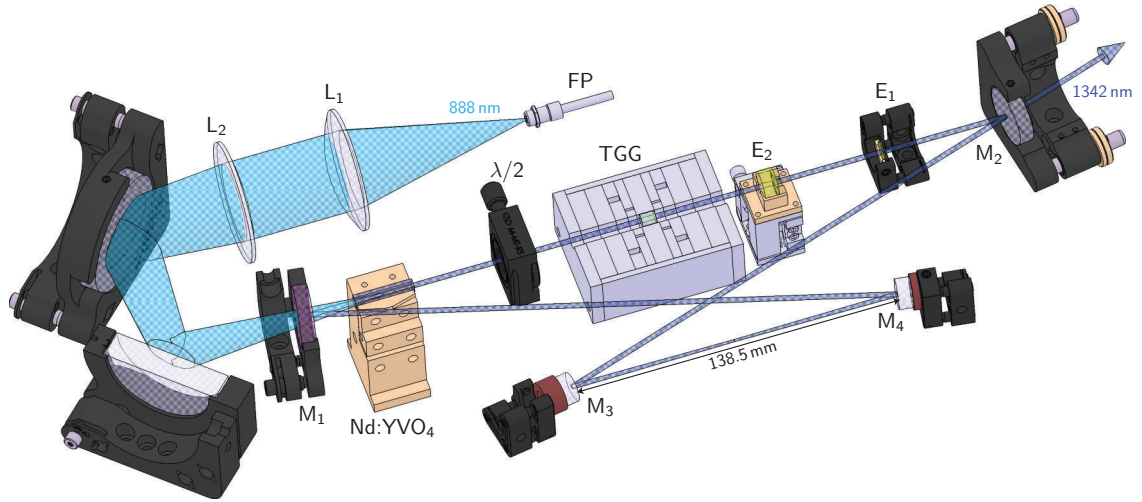
Fig. 1. (Color online) Setup of the 1342 nm laser source. Two lenses, L_1 and L_2 , image the output of the pump source, a fiber-coupled diode laser bar (FP), into the Nd:YVO 4 gain medium. The ring resonator consists of four mirrors M_{1-4} in bow-tie configuration, which are all highly reflective at 1342 nm except M_2 serving as partly transmitting output coupling mirror. A Faraday rotator (TGG) in combination with a half-wave plate ( \lambda/2 ) enforces unidirectional operation. Insertion of two etalons E_{1-2} allows for single-longitudinal-mode behavior and wavelength tunability.
