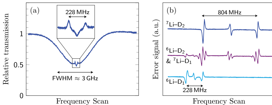
Figure 6.11: Doppler-free saturated absorption spectroscopy of the lithium D-lines. (a) Sample scan over the entire 6 Li D 1 Doppler-broadened absorption peak. The inset shows the sub-Doppler features. Similar spectra are obtained for all lithium D lines. (b) Error signals of all lithium D line transitions, generated by phase modulation spectroscopy. These signals provide an excellent reference for frequency-locking of the laser.
