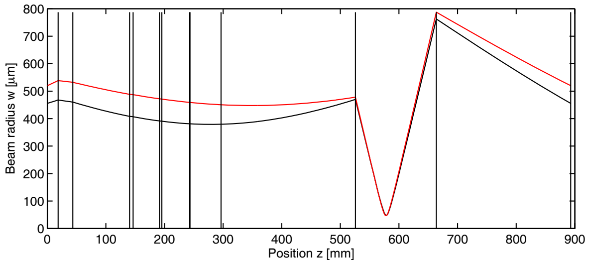
Figure 5.19: The eigenmode of the laser resonator. The horizontal (black) and the vertical (red) widths of the laser beam mode are shown as a function of the position inside the cavity. The vertical lines indicate the position of optical surfaces related to intra-cavity elements. z = 0 corresponds to the position of the convex pump coupler ( M_1 ), and the sense of propagation is directed towards the output coupler ( M_2 ), which is located at 297 mm.
