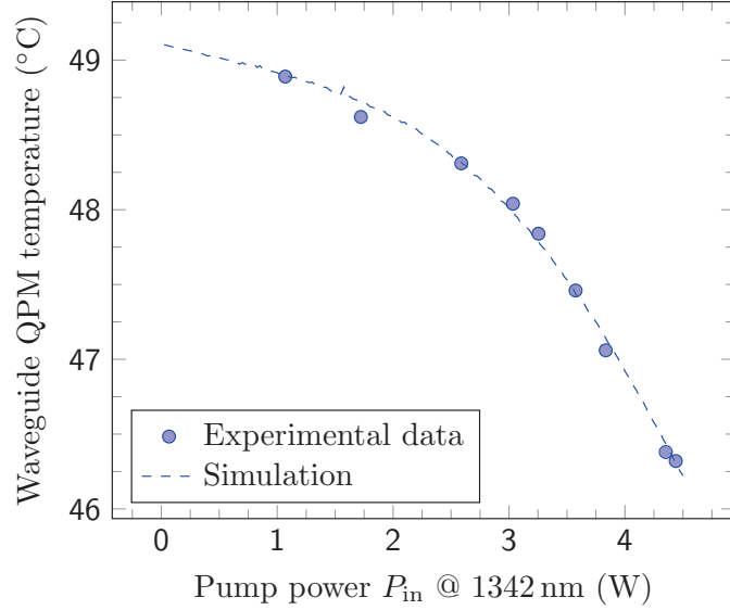
Fig. 5. (Color online) Optimal crystal mount temperature T_{\text{mount,opt}} during SHG process in dependence of the fundamental IR pump power P_{\omega} coupled to the waveguide. The crystal mount temperature is adjusted for every pump power value in order to maximize the corresponding SH power.
