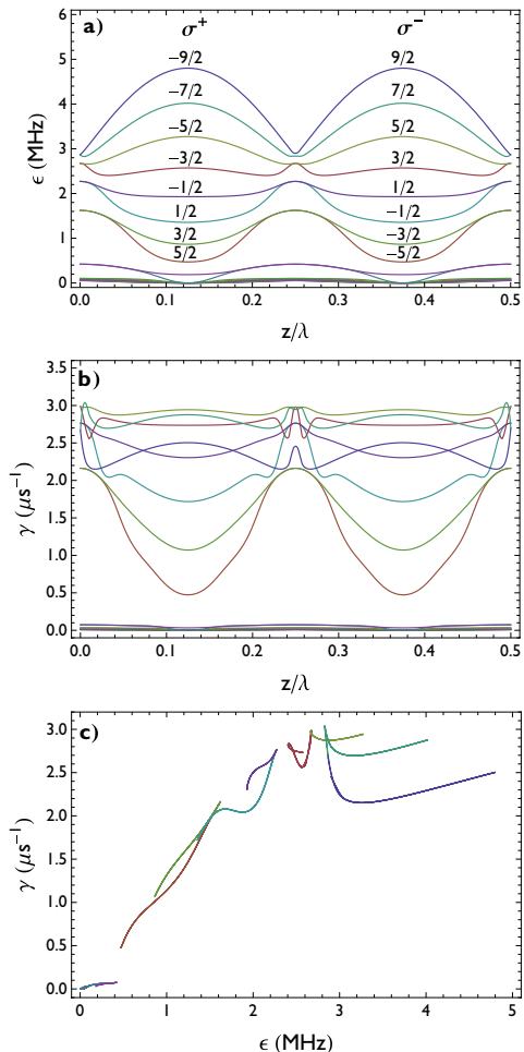
Fig. 3: (Color online) Semi-classical calculation of the effect of dual frequency counterpropagating laser beams in a 1D lin \perp lin configuration on a ^{40}\text{K} atom at rest. a) Light shifts \epsilon vs. position; b) optical pumping rates \gamma ; c) optical pumping rates vs. light shifts. The laser intensities are I_{\text{cool}} = 20I_{\text{sat}} and I_{\text{repump}} = I_{\text{cool}}/8 per beam, with \delta = +3\Gamma . The different lines correspond to the 18 dressed states of the ^2S_{1/2} ground state. At z = \lambda/8 the local polarization is \sigma^+ and here each curve corresponds to a pure m_F state. At this position the light shift increases with -m_F . The |^2S_{1/2}, F = 7/2\rangle manifold interacts only weakly with light since the repumping beam is kept at low intensity. Consequently, the light shifts and optical pumping rates are small.
