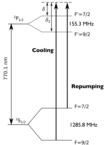
Fig. 2: Level scheme for the D_1 transition of ^{40}\text{K} and transitions used for gray-molasses cooling. The laser detuning from the cooling/repumping transitions is \delta and the detuning from the off-resonant excited hyperfine state F' = 9/2 is \delta_2 (see text).
