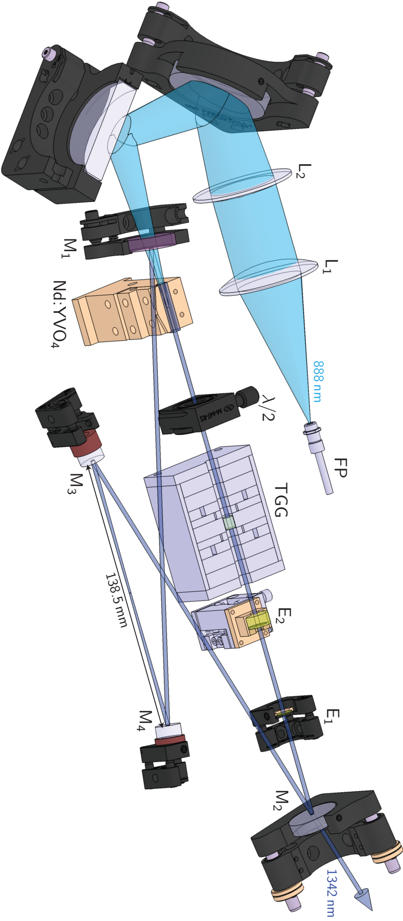
Figure 5.1. – Setup of the 1342 nm laser source from [140]. Two lenses, L 1 and L 2 , image the output of the pump source, a fiber-coupled diode laser bar (FP) emitting at 888 nm, into the Nd:YVO 4 gain medium. The ring resonator consists of four mirrors M 1-4 in bow-tie configuration, which are all highly reflective at 1342 nm except M 2 serving as partly transmitting output coupling mirror. A Faraday rotator (TGG) in combination with a half-wave plate ( \lambda/2 ) enforces unidirectional operation. Insertion of two etalons E 1-2 allows for single-longitudinal-mode behavior and wavelength tunability. For a technical drawing of the cavity setup see Figure 5.10.
