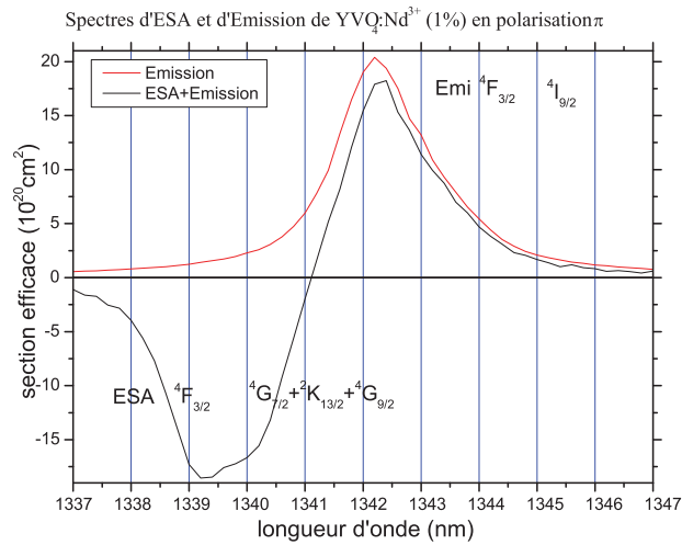
Figure 5.5: High-resolution emission spectrum around the 1342 nm transition, measured on the c-axis by the group of R. Moncorgé [195] and first published in [184]. For the wavelength 2\lambda_{\text{LiD-Lines}} we are interested in, one can deduce an emission cross-section of \sigma_{\text{em}}(2\lambda_{\text{LiD-Lines}}) = 12 \times 10^{-20} \text{ cm}^2 and an excited-state absorption (ESA) cross-section of \sigma_{\text{ESA}}(2\lambda_{\text{LiD-Lines}}) = 3 \times 10^{-20} \text{ cm}^2
