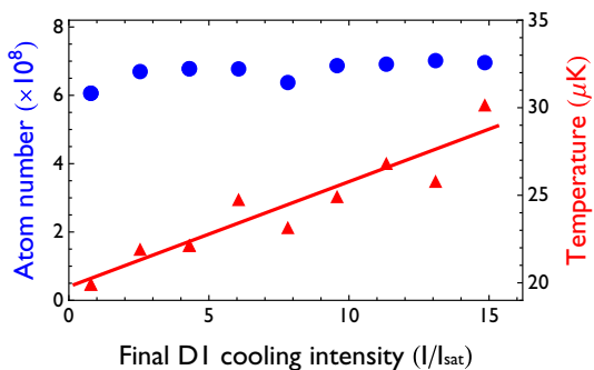
Fig. 6: (Color online) Number of atoms captured in the D_1 molasses (circles) and their temperature (triangles) after a 6 ms capture phase at high intensity I_{\text{cool}} = 14I_{\text{sat}} followed by a 2 ms linear intensity ramp to adjustable value. The detuning is fixed to \delta = 2.3\Gamma . The number of atoms in the compressed MOT was 7 \times 10^8 .
