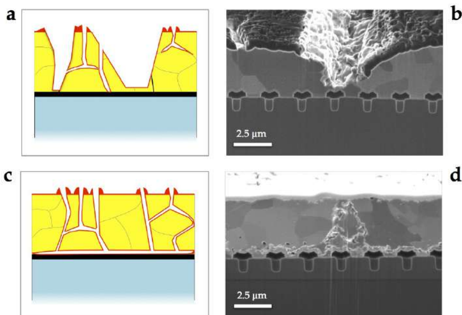
Figure 126: Crack propagation models through the Al layer at failure. (a) For SPD06 power modules at the final aging stage until failure, fatigues cracks running from the surface along the grain boundaries become broader and broader. (b) SIM cross-sectional image of the cracked metal in a failed SPD06, showing a crack width on the same order of the metallization thickness. (c) In To7D17 failed power modules, finer vertical cracks branch out and propagate horizontally all long the MOSFETs region. (d) Relative SIM cross-sectional imaging from a 70°C aged module.
