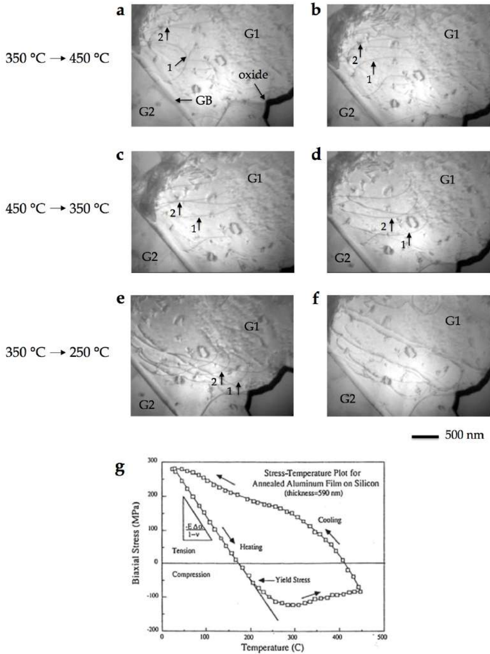
Figure 87: In situ TEM thermal cycling from 25 °C to 450 °C of a device cross-section prepared by tripod. The Si substrate is preserved, inducing a reversible motion, according to the stress inversion for a Al/Si substrate thin film in the stress-temperature curve [Fli87]. (a)-(b) are snapshots captured during the heating up phase from 350 °C to 450 °C, showing the dislocation activation. During the cooling down phase, the reversible motion is characterized by an initial dislocation straightening (c) followed by a bowing in the opposite direction (d), towards the oxide (d)-(e).
