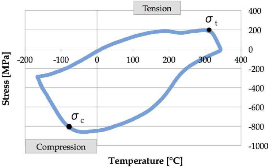
Figure 140: Stress-Temperature cycle for the Al thin film deposited onto the Si wafer. The relative stress is measured along the larger die dimension, and the zero value is here taken at 350°C. The cycle is initiated at T = -190°C, and the T gradient is set to 20°C/min during heating and cooling.
