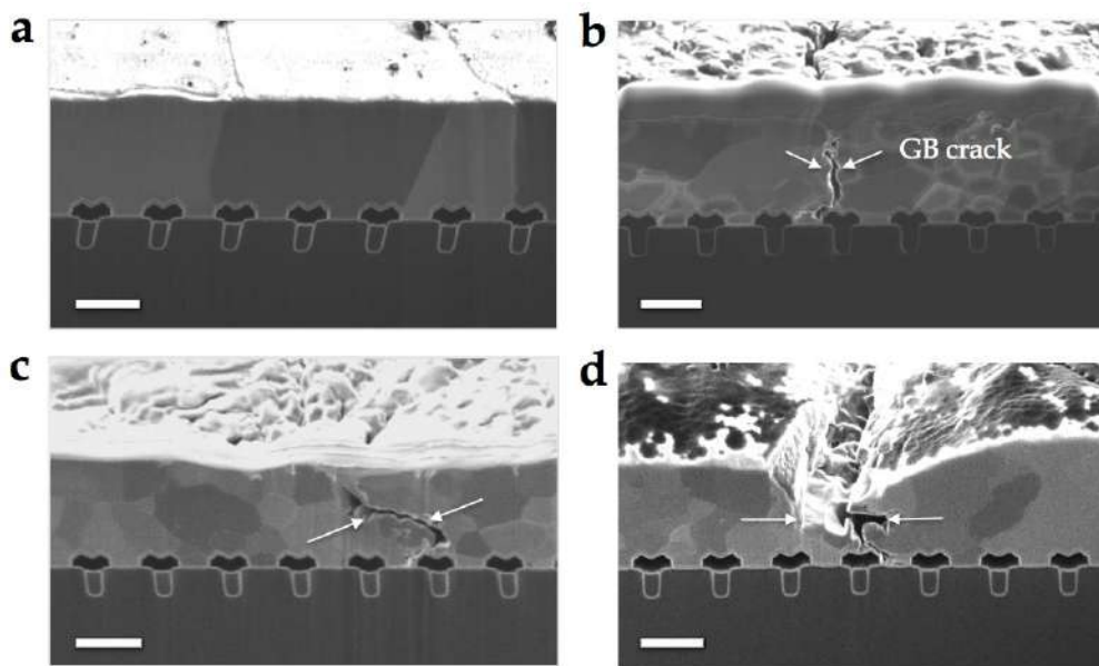
Figure 79: SIM imaging of the Al source metallization of an (a) as-is and (b) 100, (c) 200 and (d) 300 kcycles aged power modules. Scale bar 2 μm.
