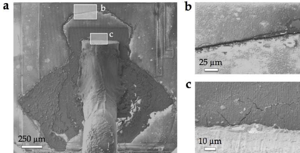
Figure 105: (a) Top view SEM image of an Al bond wire welded on the Al source metallization in a 25^{\circ}\text{C} aged device, after a short-circuit event. At higher magnification, big cracks propagating in (b) the passivated metallization and (c) next to the bonding wire (located in the boxes (b) and (c) in (a)).
