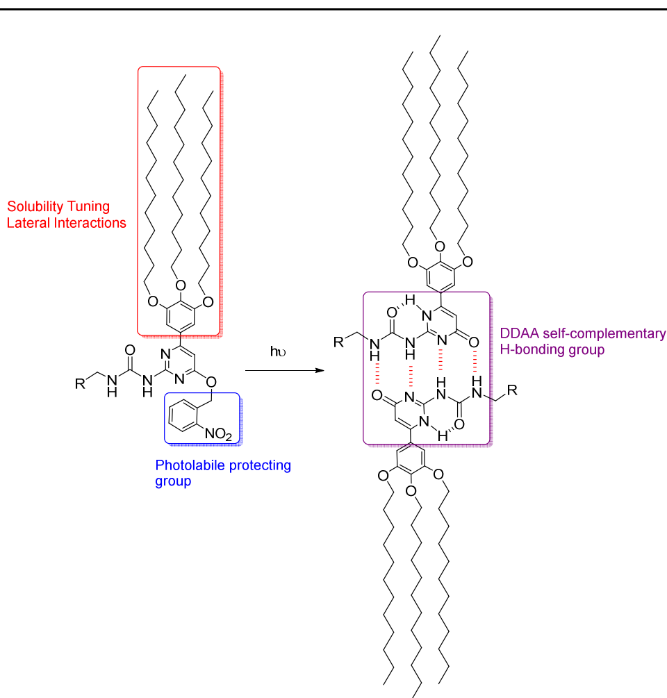
Figure 72 | Design of a multifunctional Upy connector.
