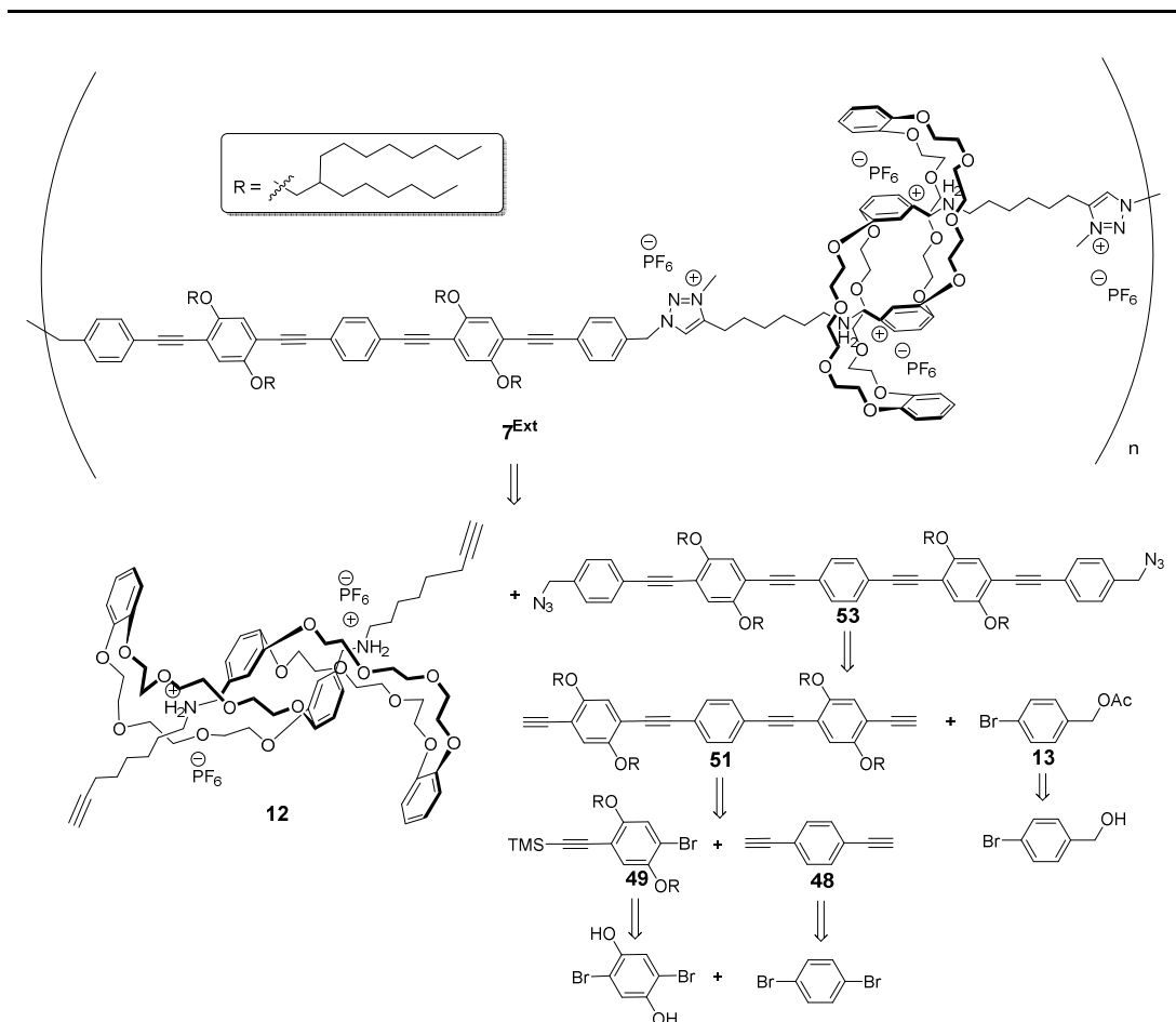
Figure 86 | Retrosynthetic scheme for covalent polymer 7 Ext .
