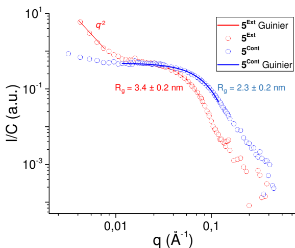
Figure 82 | Scattering profile for toluene solutions of 5 Cont at 3.24 \times 10^{-3} M and 5 Ext at 3.15 \times 10^{-3} M normalized by the concentration.
