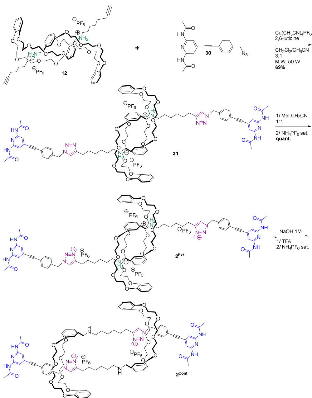
Scheme 14 | Synthesis of the bis-2,6-diacetylaminopyridine [c2]daisy chains 2 Ext and its contraction into 2 Cont .
