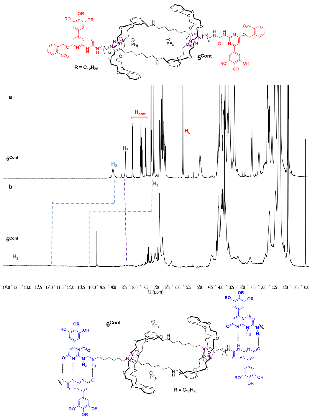
Figure A 5 | ^1\text{H} NMR in \text{CDCl}_3 of a 5 mM solution of a) 5Cont and b) 6Cont after 6 hours of irradiation.
