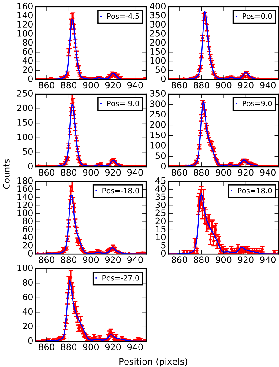
Figure 3.6 – Experimental data (red error bars) and fitted profile (blue lines) F(x) for different spectra corresponding to different positions Pos. with respect the theoretical focal position (which does not corresponds to the real one as one can see from the width of the lines). The peak asymmetry on the high-energy side of the peak (right) is due to the typical aberration of Johann-type spectrometer from the X rays diffracted by the regions of the crystal far from its centre.
