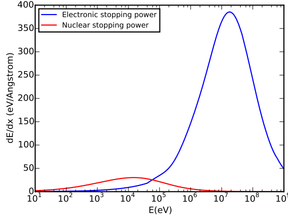
Figure 5.2 – Electric and nuclear stopping power of Ne ions of MnAs as function of the ion kinetic energy obtained by SRIM [182, 187].
