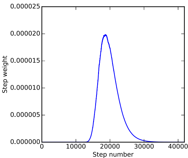
Fig. 4. Weights associated to discarded value at each step, which are proportional to the product \mathcal{L}_m \Delta X_m .
