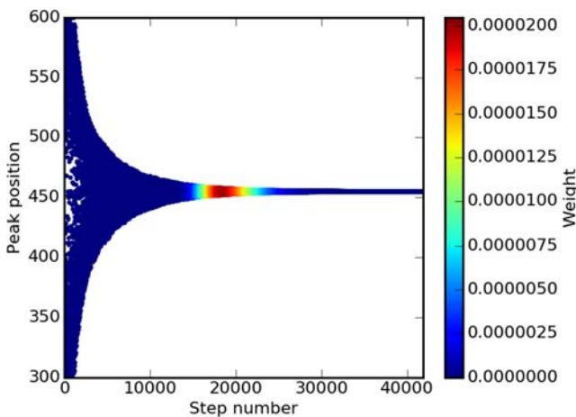
Fig. 3. Evolution of the sampled parameter value relative to the peak over the algorithm step.
