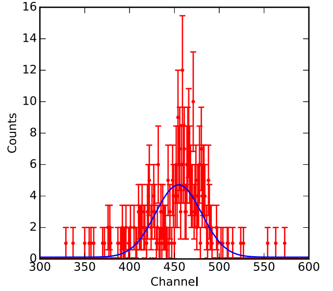
Fig. 2. High-resolution X-ray spectrum of the helium-like uranium 1s2p \ ^3P_2 \rightarrow 1s2s \ ^3S_1 intrashell transition from Ref. [31] and corresponding fit with one Gaussian peak (plus a flat background).
