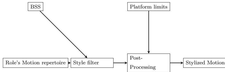
FIGURE 4.5: Pipeline of Stylistic treatment of data
