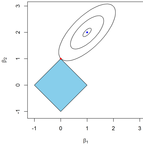
FIGURE 1.2 – Lasso
