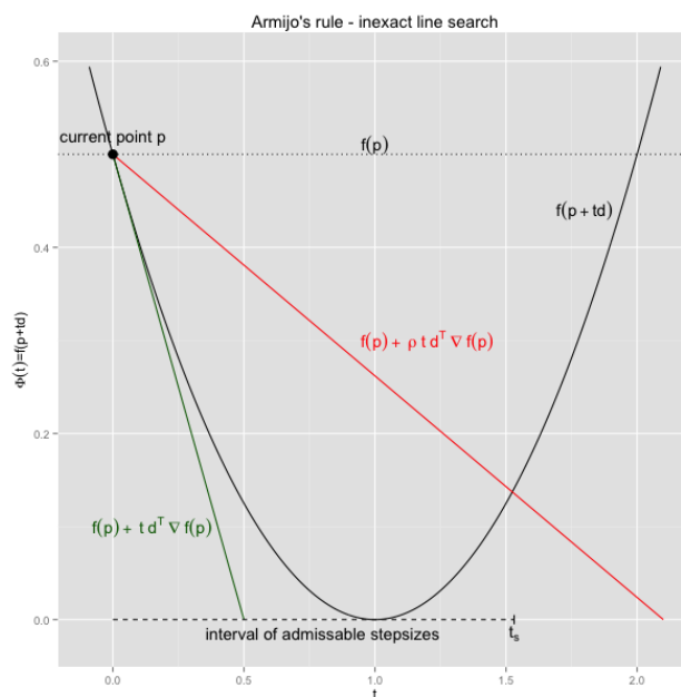
FIGURE 2.2 – Condition d'Armijo. Source 1
